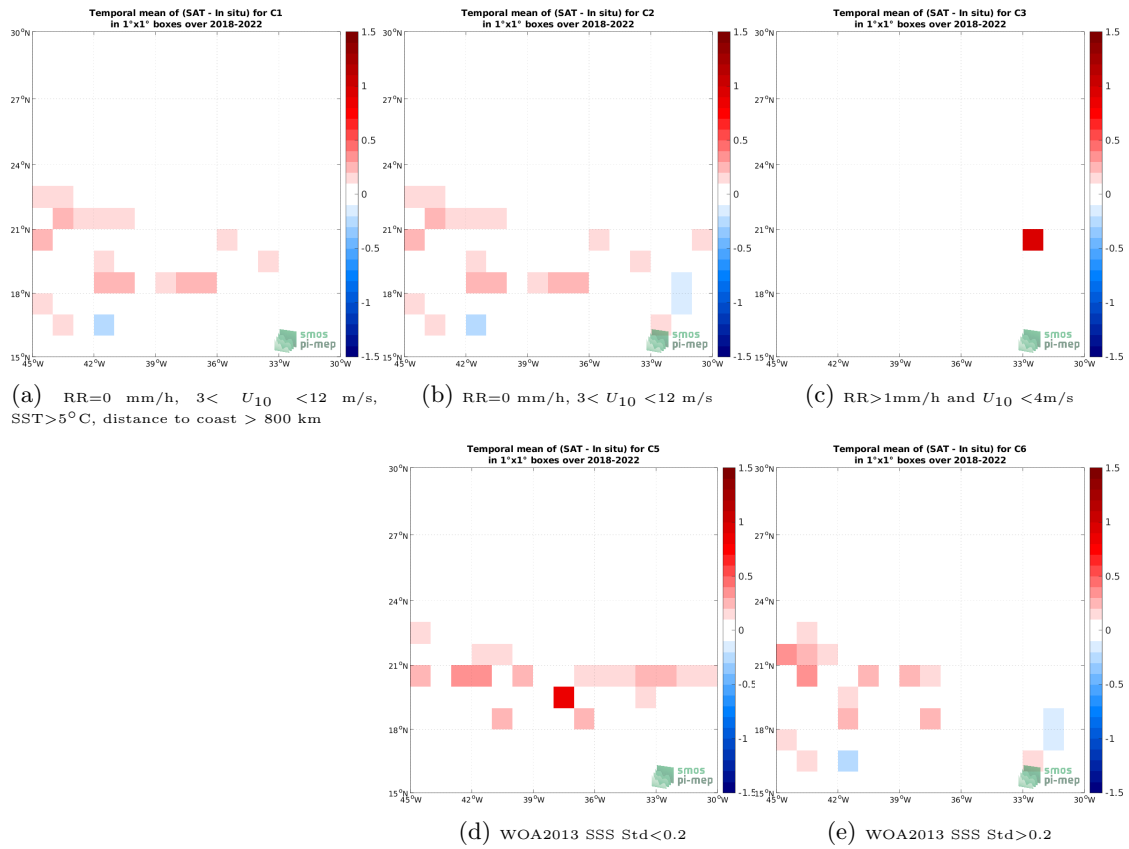
Figure 12: Temporal mean gridded over spatial boxes of size 1^\circ \times 1^\circ of \Delta SSS (SMAP SSS L3 v5 - Monthly (RSS) - TSG (SAMOS)) for 5 different subdatasets corresponding to:RR=0 mm/h, 3 < U_{10} < 12 m/s, SST >5^\circ\text{C} , distance to coast > 800 km (a), RR=0 mm/h, 3 < U_{10} < 12 m/s (b), RR >1 mm/h and U_{10} < 4 m/s (c), WOA2013 SSS Std <0.2 (d), WOA2013 SSS Std >0.2 (e).
