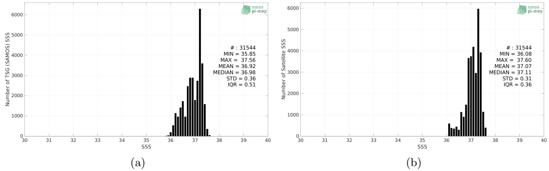
Figure 2: Histograms of SSS from TSG (SAMOS) (a) and SMAP SSS L3 v5 - Monthly (RSS) (b) considering all match-up pairs per bins of 0.1 over the SPURS 1 Pi-MEP region and for the full satellite product period.
