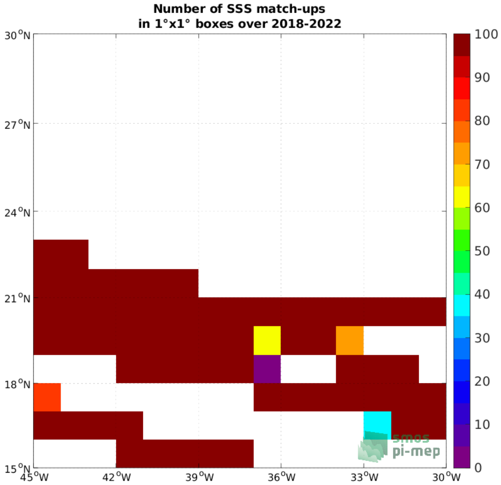
Figure 4: Number of SSS match-ups between TSG (SAMOS) SSS and the SMAP SSS L3 v5 - Monthly (RSS) SSS product for the SPURS 1 Pi-MEP region over 1^\circ \times 1^\circ boxes and for the full satellite product period.
