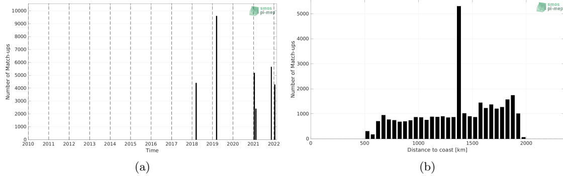
Figure 1: Number of match-ups between TSG (SAMOS) and SMAP SSS L3 v5 - Monthly (RSS) SSS as a function of time (a) and as function of the distance to coast (b) over the SPURS 1 Pi-MEP region and for the full satellite product period.
