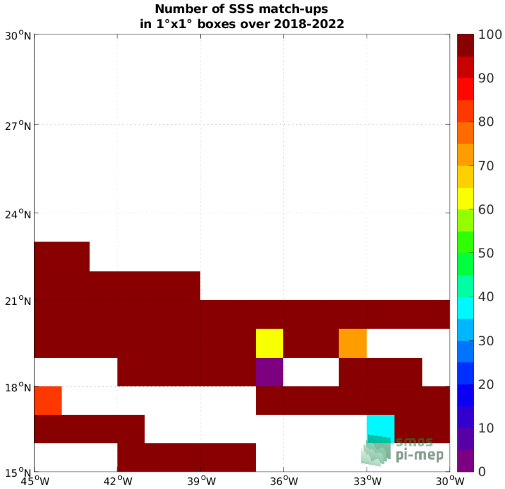
Figure 4: Number of SSS match-ups between TSG (SAMOS) SSS and the SMAP SSS L3 v5 - Monthly (RSS) SSS product for the SPURS 1 Pi-MEP region over 1°x1° boxes and for the full satellite product period.
