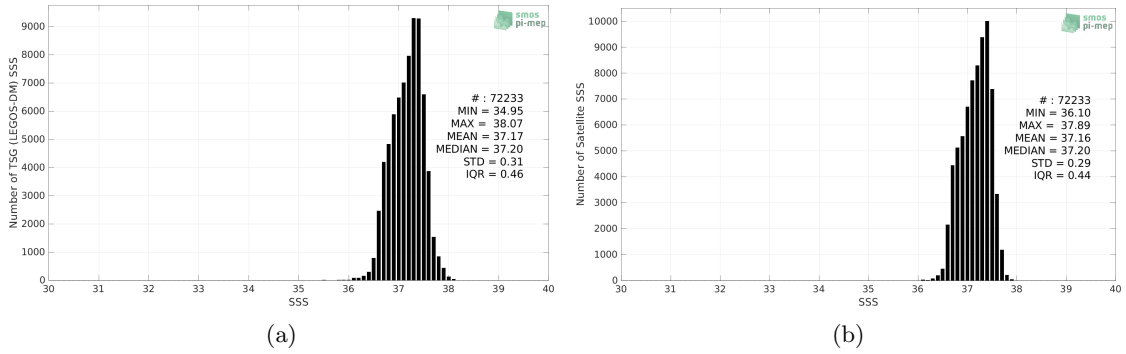
Figure 2: Histograms of SSS from TSG (LEGOS-DM) (a) and SMAP SSS L3 v5 - Monthly (RSS) (b) considering all match-up pairs per bins of 0.1 over the SPURS 1 Pi-MEP region and for the full satellite product period.
