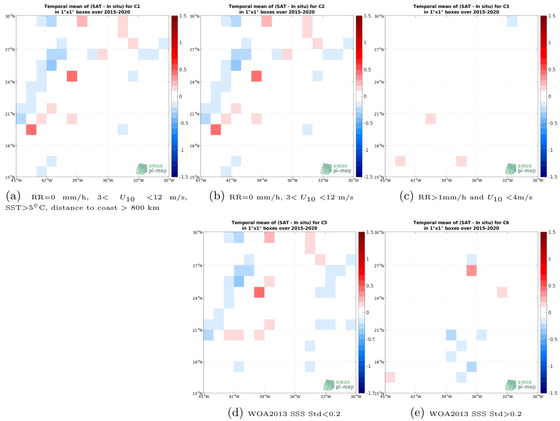
Figure 12: Temporal mean gridded over spatial boxes of size 1^\circ \times 1^\circ of \Delta SSS (SMAP SSS L3 v5 - Monthly (RSS) - TSG (LEGOS-DM)) for 5 different subdatasets corresponding to: RR=0 mm/h, 3 < U_{10} < 12 m/s, SST > 5^\circ\text{C} , distance to coast > 800 km (a), RR=0 mm/h, 3 < U_{10} < 12 m/s (b), RR > 1 mm/h and U_{10} < 4 m/s (c), WOA2013 SSS Std < 0.2 (d), WOA2013 SSS Std > 0.2 (e).
