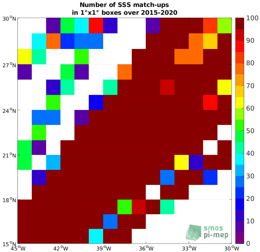
Figure 4: Number of SSS match-ups between TSG (LEGOS-DM) SSS and the SMAP SSS L3 v5 - Monthly (RSS) SSS product for the SPURS 1 Pi-MEP region over 1^\circ \times 1^\circ boxes and for the full satellite product period.
