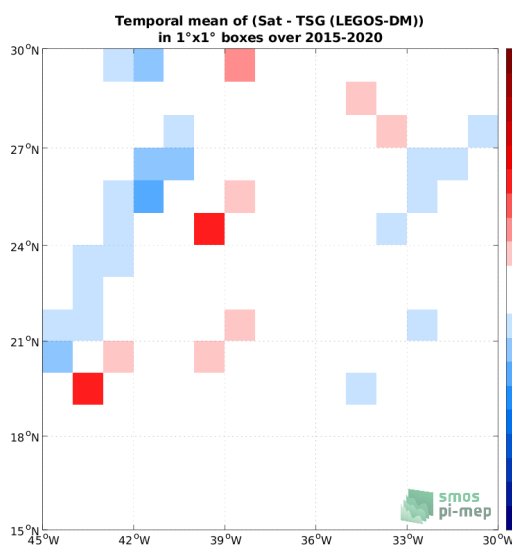
(e) MEAN( \Delta SSS) (Satellite - TSG (LEGOS-DM))
