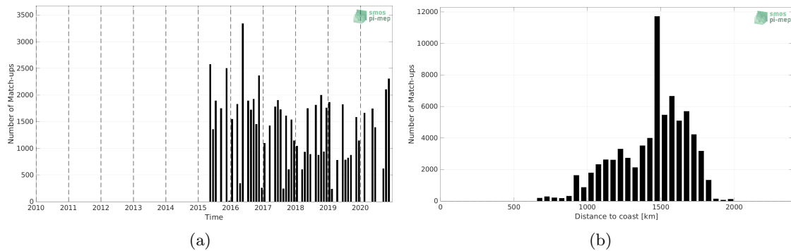
Figure 1: Number of match-ups between TSG (LEGOS-DM) and SMAP SSS L3 v5 - Monthly (RSS) SSS as a function of time (a) and as function of the distance to coast (b) over the SPURS 1 Pi-MEP region and for the full satellite product period.
