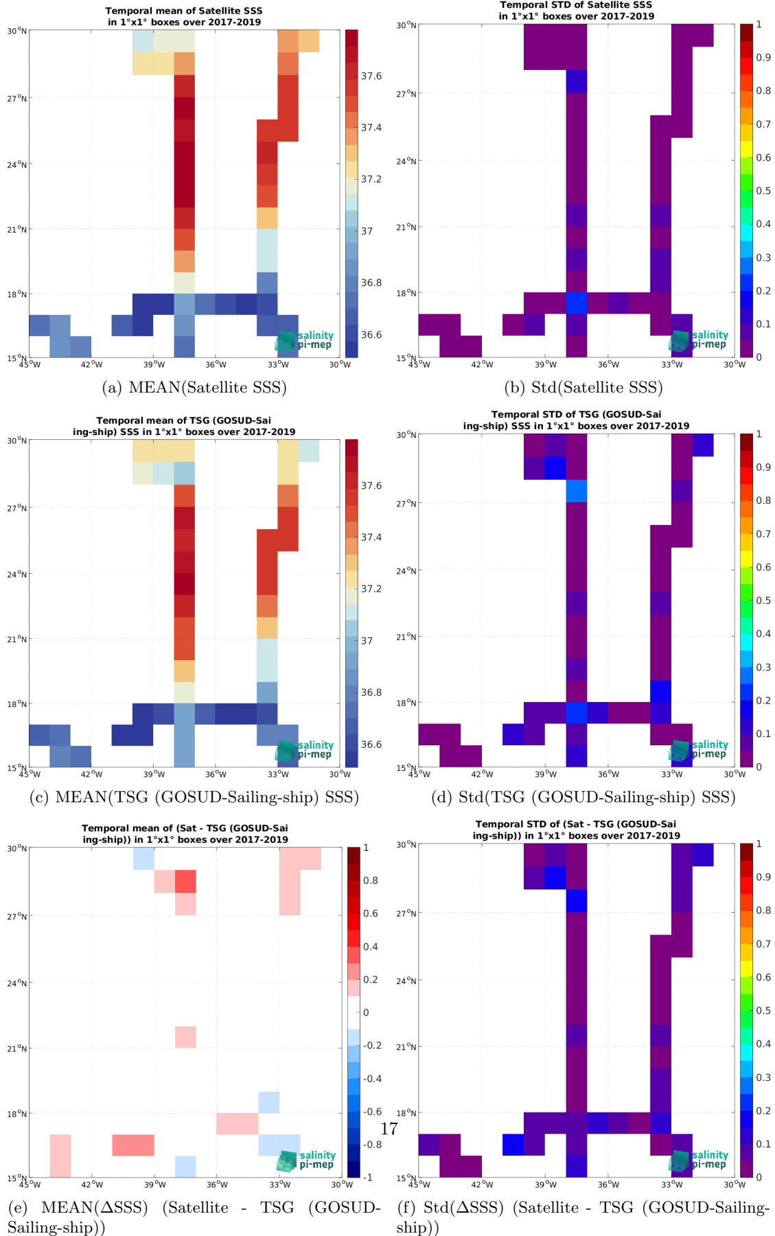
Figure 6: Temporal mean (left) and Std (right) of SSS from SMAP SSS L3 v5 - Monthly (RSS) (top), TSG (GOSUD-Sailing-ship) (middle), and of \Delta SSS (Satellite - TSG (GOSUD-Sailing-ship)). Only match-up pairs are used to generate these maps.
