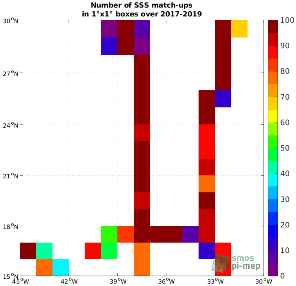
Figure 4: Number of SSS match-ups between TSG (GOSUD-Sailing-ship) SSS and the SMAP SSS L3 v5 - Monthly (RSS) SSS product for the SPURS 1 Pi-MEP region over 1^\circ \times 1^\circ boxes and for the full satellite product period.
