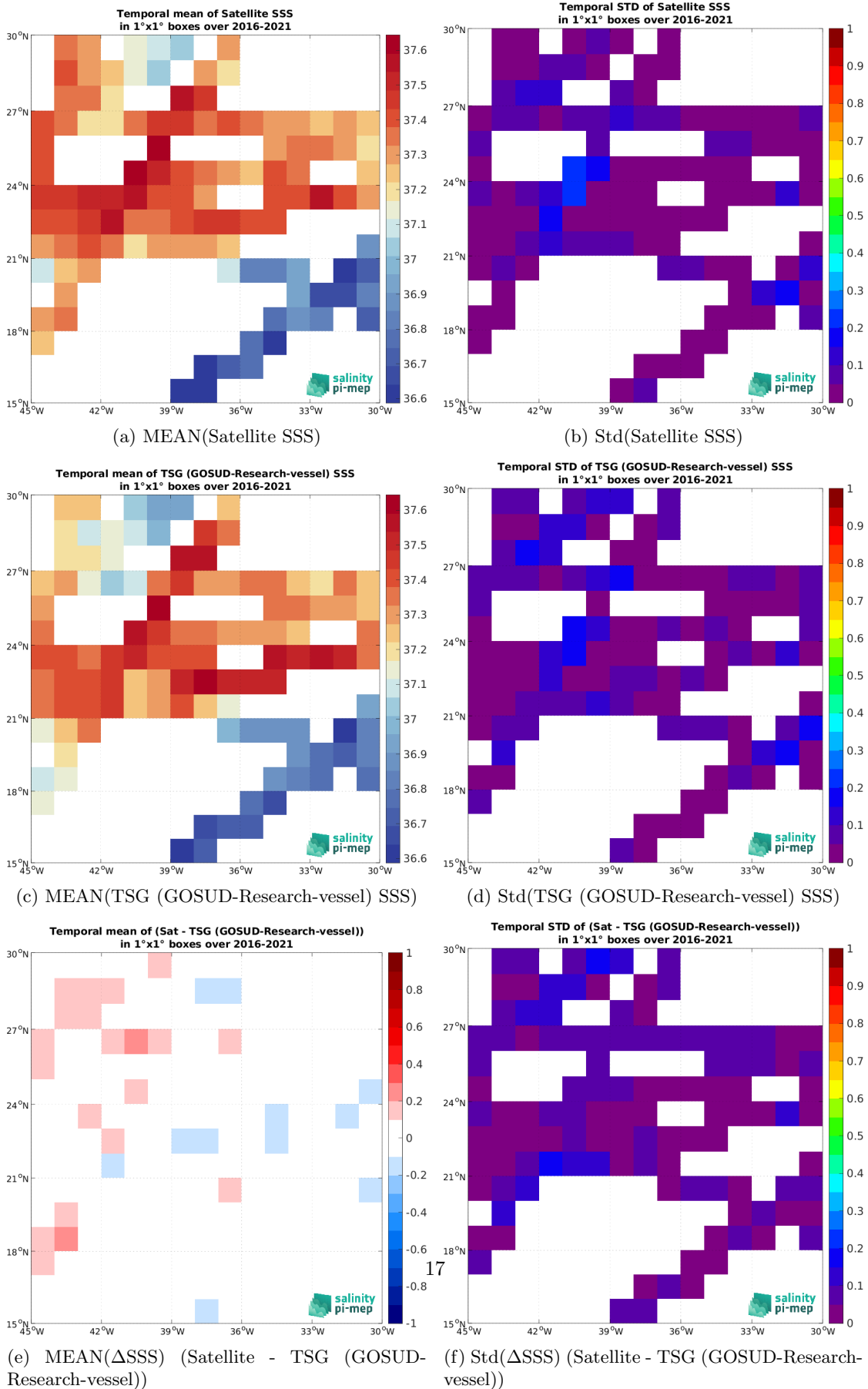
Figure 6: Temporal mean (left) and Std (right) of SSS from SMAP SSS L3 v5 - Monthly (RSS) (top), TSG (GOSUD-Research-vessel) (middle), and of \Delta SSS (Satellite - TSG (GOSUD-Research-vessel)). Only match-up pairs are used to generate these maps.
