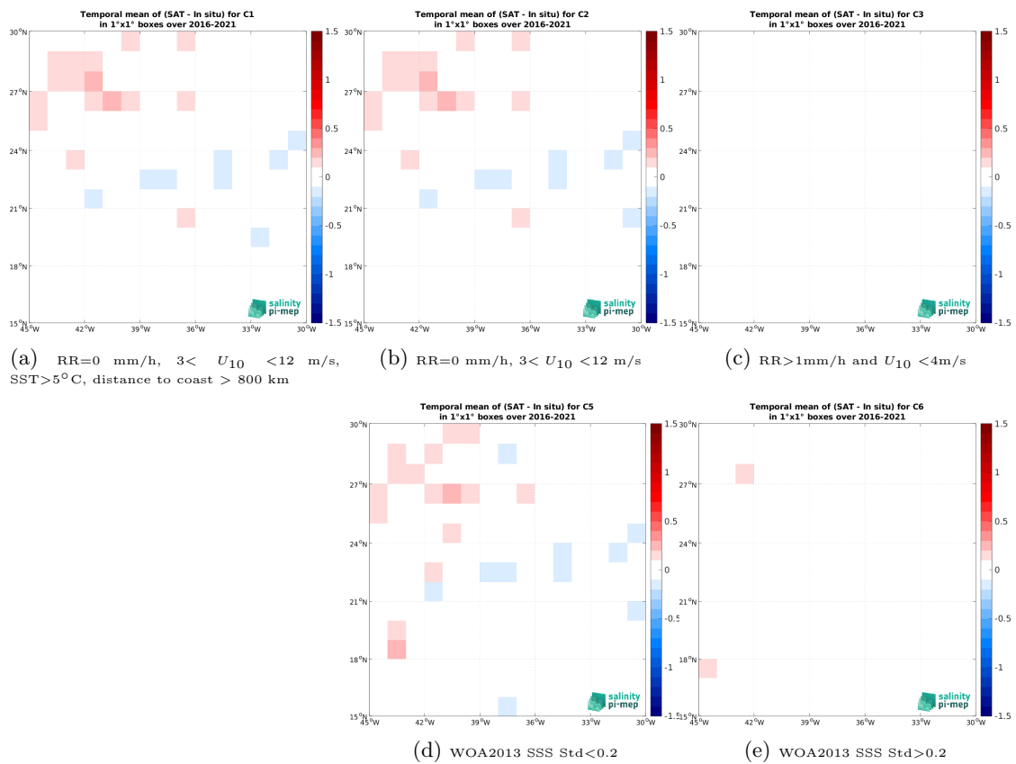
Figure 12: Temporal mean gridded over spatial boxes of size 1^\circ \times 1^\circ of \Delta\text{SSS} (SMAP SSS L3 v5 - Monthly (RSS) - TSG (GOSUD-Research-vessel)) for 5 different subdatasets corresponding to: \text{RR}=0 \text{ mm/h} , 3 < U_{10} < 12 \text{ m/s} , \text{SST} > 5^\circ\text{C} , distance to coast > 800 \text{ km} (a), \text{RR}=0 \text{ mm/h} , 3 < U_{10} < 12 \text{ m/s} (b), \text{RR} > 1\text{mm/h} and U_{10} < 4\text{m/s} (c), WOA2013 SSS Std < 0.2 (d), WOA2013 SSS Std > 0.2 (e).
