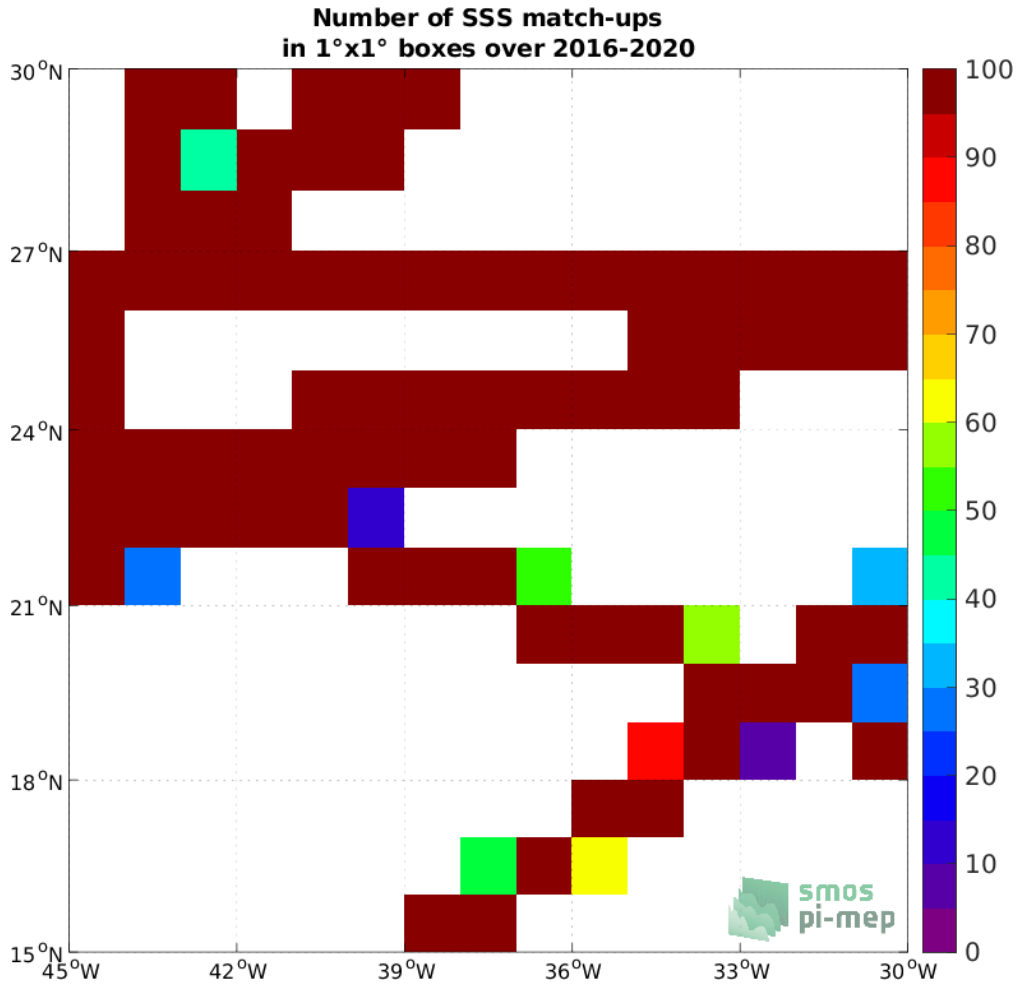
Figure 4: Number of SSS match-ups between TSG (GOSUD-Research-vessel) SSS and the SMAP SSS L3 v5 - Monthly (RSS) SSS product for the SPURS 1 Pi-MEP region over 1°x1° boxes and for the full satellite product period.
