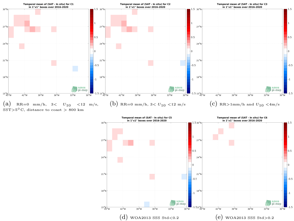
Figure 12: Temporal mean gridded over spatial boxes of size 1^\circ \times 1^\circ of \Delta SSS (SMAP SSS L3 v5 - Monthly (RSS) - TSG (GOSUD-Research-vessel)) for 5 different subdatasets corresponding to:RR=0 mm/h, 3 < U_{10} < 12 m/s, SST >5^\circ C, distance to coast > 800 km (a), RR=0 mm/h, 3 < U_{10} < 12 m/s (b), RR >1 mm/h and U_{10} < 4 m/s (c), WOA2013 SSS Std <0.2 (d), WOA2013 SSS Std >0.2 (e).
