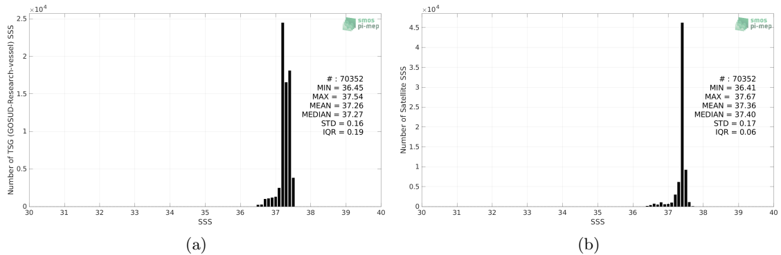
Figure 2: Histograms of SSS from TSG (GOSUD-Research-vessel) (a) and SMAP SSS L3 v5 - Monthly (RSS) (b) considering all match-up pairs per bins of 0.1 over the SPURS 1 Pi-MEP region and for the full satellite product period.
