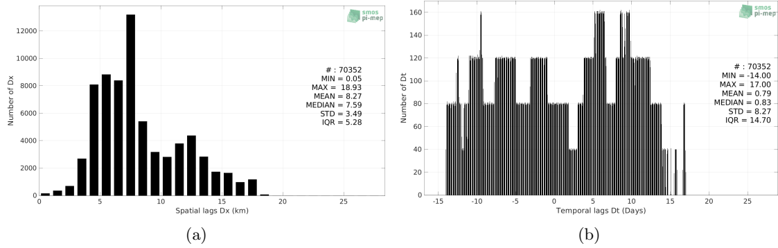
Figure 5: Histograms of the spatial (a) and temporal (b) lags between the location/time of the TSG (GOSUD-Research-vessel) measurement and the date of the corresponding SMAP SSS L3 v5 - Monthly (RSS) SSS pixel.
