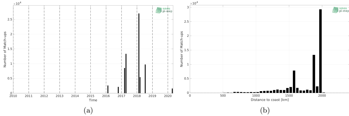
Figure 1: Number of match-ups between TSG (GOSUD-Research-vessel) and SMAP SSS L3 v5 - Monthly (RSS) SSS as a function of time (a) and as function of the distance to coast (b) over the SPURS 1 Pi-MEP region and for the full satellite product period.
