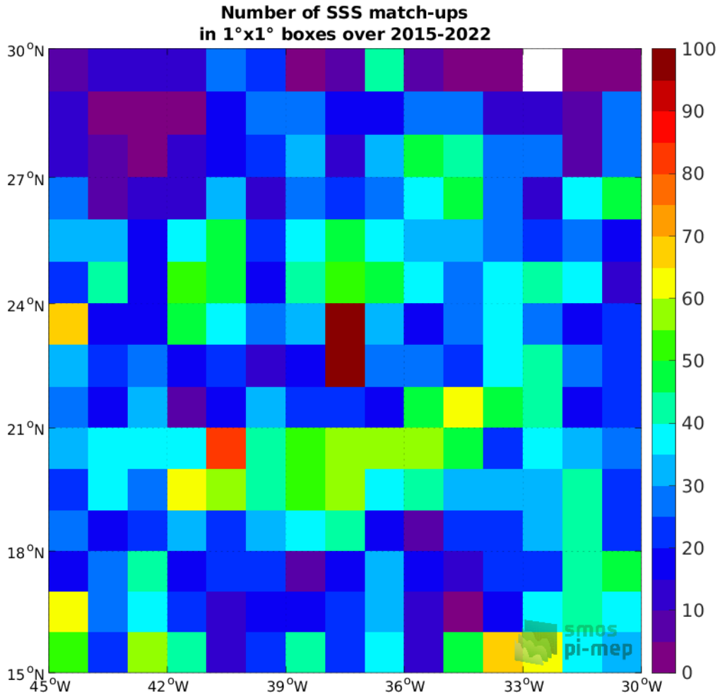
Figure 4: Number of SSS match-ups between Argo SSS and the SMAP SSS L3 v5 - Monthly (RSS) SSS product for the SPURS 1 Pi-MEP region over 1°x1° boxes and for the full satellite product period.
