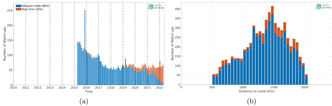
Figure 1: Number of match-ups between Argo and SMAP SSS L3 v5 - Monthly (RSS) SSS as a function of time (a) and as function of the distance to coast (b) over the SPURS 1 Pi-MEP region and for the full satellite product period.
