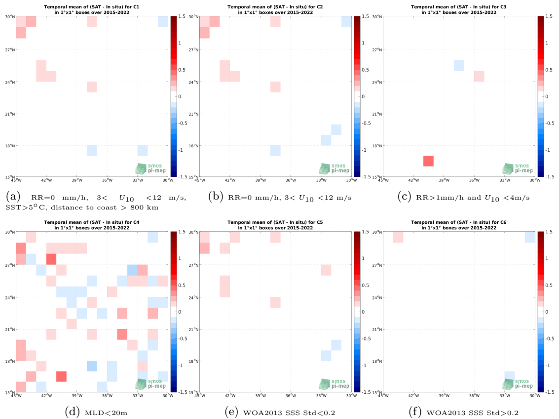
Figure 12: Temporal mean gridded over spatial boxes of size 1^\circ \times 1^\circ of \Delta SSS (SMAP SSS L3 v5 - Monthly (RSS) - Argo) for 6 different subdatasets corresponding to:RR=0 mm/h, 3 < U_{10} < 12 m/s, SST >5^\circ C, distance to coast > 800 km (a), RR=0 mm/h, 3 < U_{10} < 12 m/s (b), RR >1 mm/h and U_{10} < 4 m/s (c),MLD <20 m (d),WOA2013 SSS Std <0.2 (e),WOA2013 SSS Std >0.2 (f).
