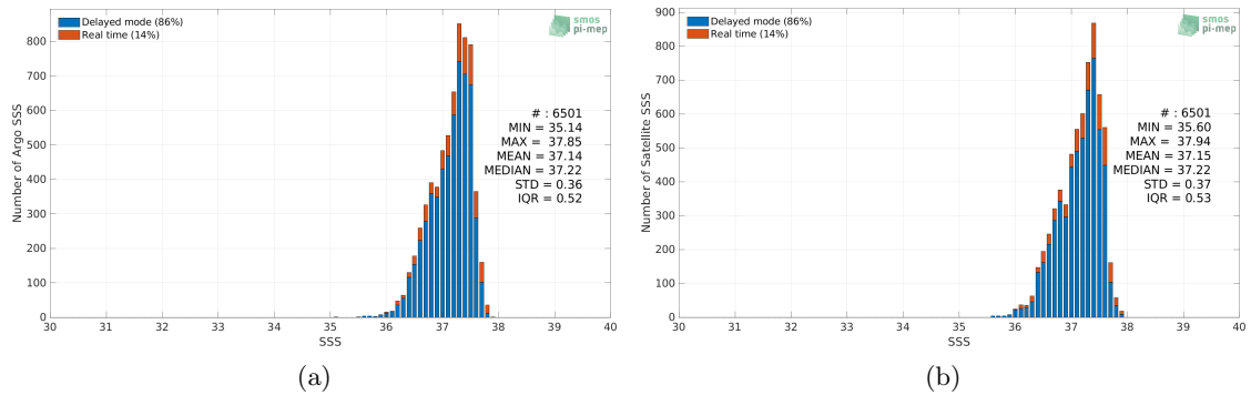
Figure 2: Histograms of SSS from Argo (a) and SMAP SSS L3 v5 - Monthly (RSS) (b) considering all match-up pairs per bins of 0.1 over the SPURS 1 Pi-MEP region and for the full satellite product period.
