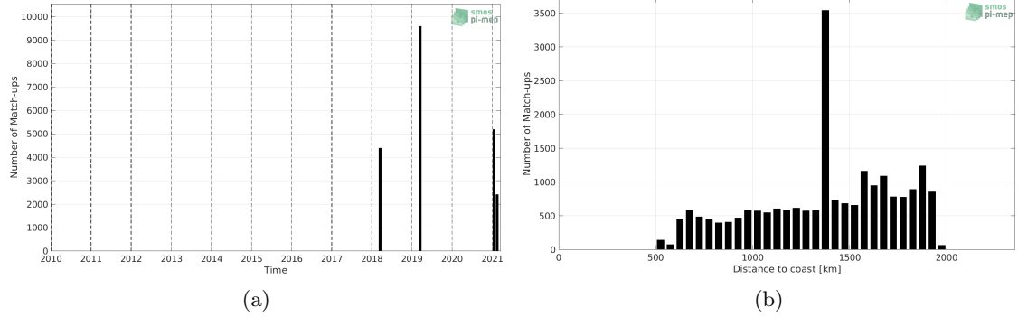
Figure 1: Number of match-ups between TSG (SAMOS) and SMAP SSS L3 v4 - 8-Day running (RSS) SSS as a function of time (a) and as function of the distance to coast (b) over the SPURS 1 Pi-MEP region and for the full satellite product period.
