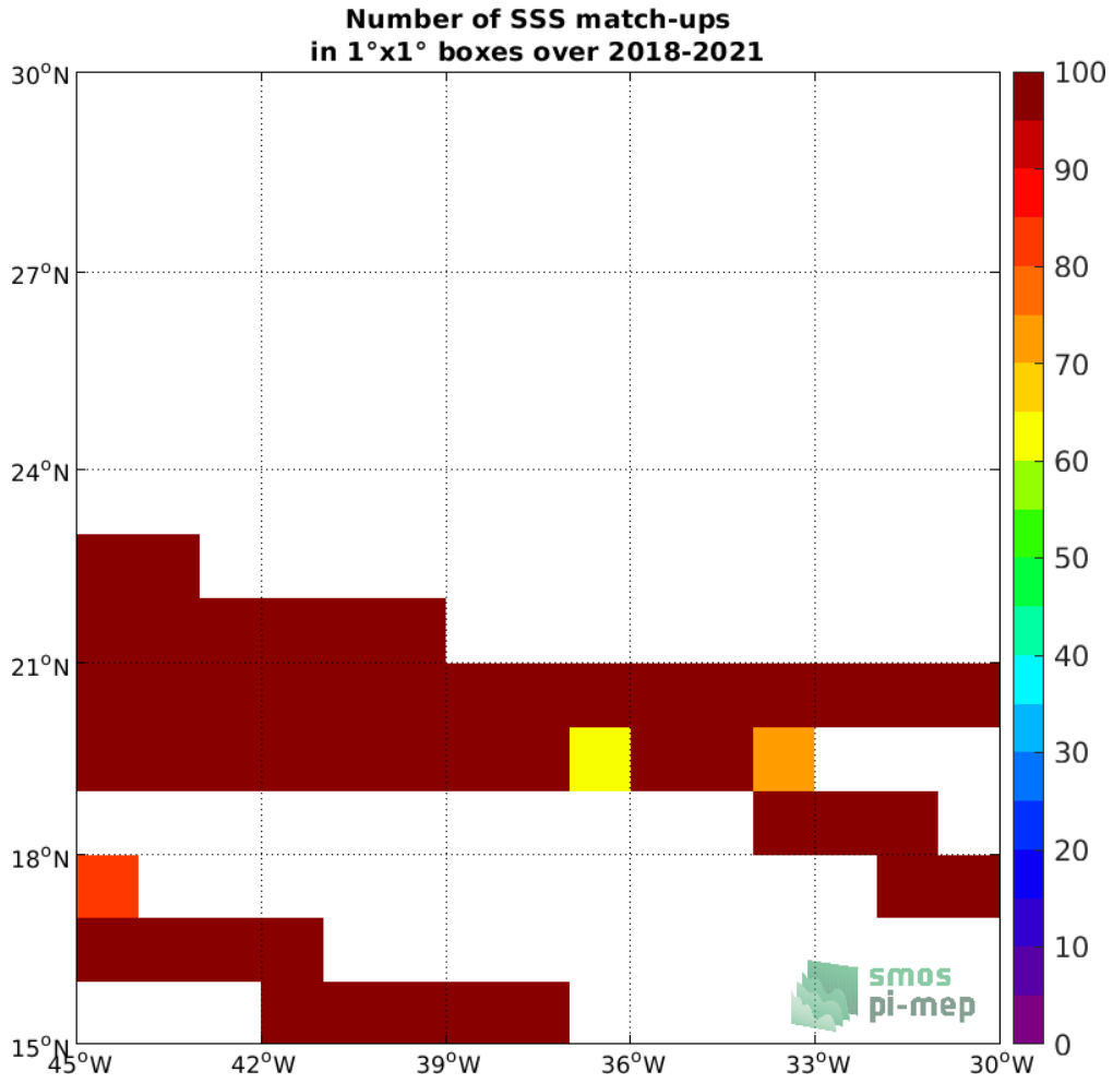
Figure 4: Number of SSS match-ups between TSG (SAMOS) SSS and the SMAP SSS L3 v4 - 8-Day running (RSS) SSS product for the SPURS 1 Pi-MEP region over 1°x1° boxes and for the full satellite product period.
