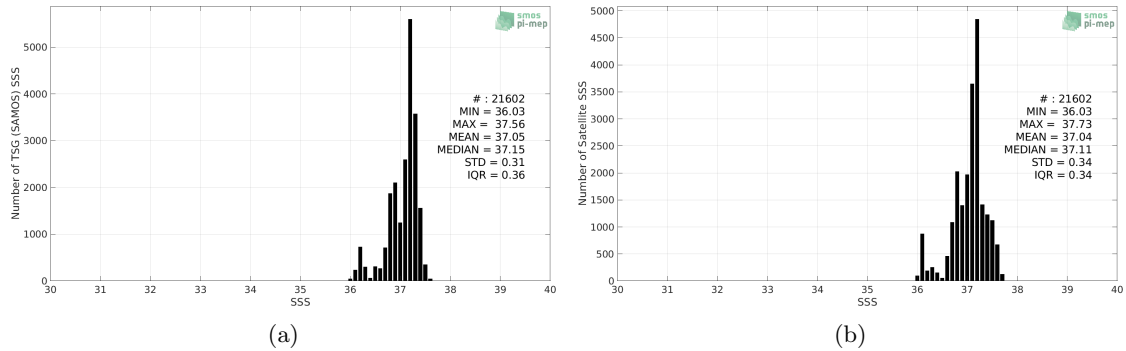
Figure 2: Histograms of SSS from TSG (SAMOS) (a) and SMAP SSS L3 v4 - 8-Day running (RSS) (b) considering all match-up pairs per bins of 0.1 over the SPURS 1 Pi-MEP region and for the full satellite product period.
