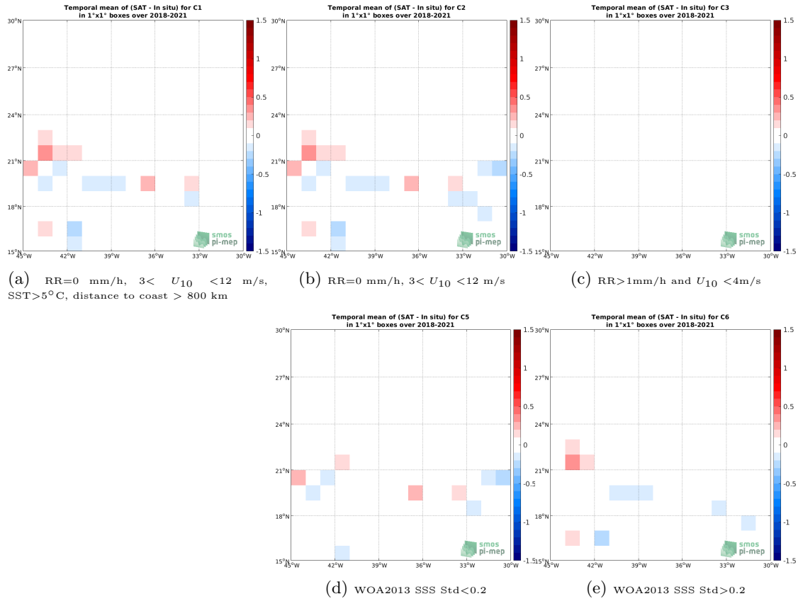
Figure 12: Temporal mean gridded over spatial boxes of size 1^\circ \times 1^\circ of \Delta SSS (SMAP SSS L3 v4 - 8-Day running (RSS) - TSG (SAMOS)) for 5 different subdatasets corresponding to:RR=0 mm/h, 3 < U_{10} < 12 m/s, SST >5^\circ\text{C} , distance to coast > 800 km (a), RR=0 mm/h, 3 < U_{10} < 12 m/s (b), RR >1 mm/h and U_{10} < 4 m/s (c), WOA2013 SSS Std <0.2 (d), WOA2013 SSS Std >0.2 (e).
