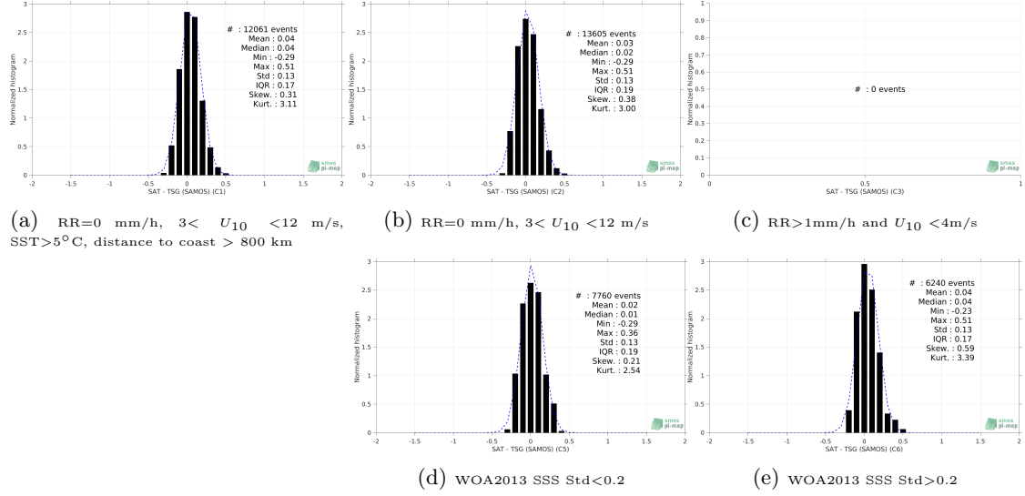
Figure 13: Normalized histogram of \Delta SSS (SMAP SSS L3 v4 - 8-Day running (RSS) - TSG (SAMOS)) for 5 different subdatasets corresponding to: RR=0 mm/h, 3 < U_{10} < 12 m/s, SST > 5^\circ\text{C} , distance to coast > 800 km (a), RR=0 mm/h, 3 < U_{10} < 12 m/s (b), RR > 1\text{mm/h} and U_{10} < 4\text{m/s} (c), WOA2013 SSS Std < 0.2 (d), WOA2013 SSS Std > 0.2 (e).
