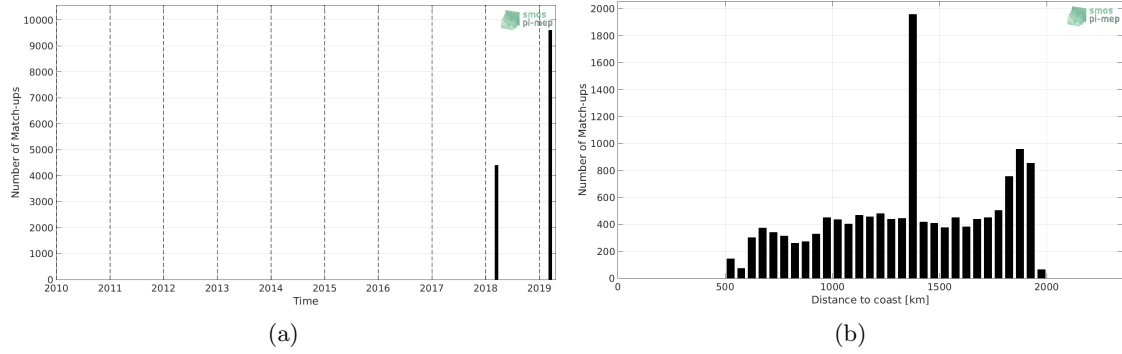
Figure 1: Number of match-ups between TSG-SAMOS and SMAP-L3-RSS-V4-8DAY-RUNNING SSS as a function of time (a) and as function of the distance to coast (b) over the SPURS 1 Pi-MEP region and for the full satellite product period.
