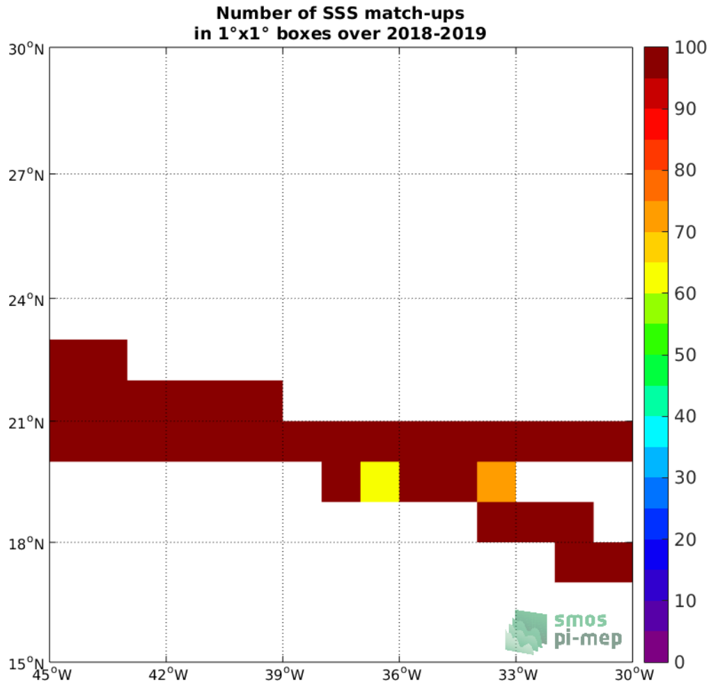
Figure 4: Number of SSS match-ups between TSG-SAMOS SSS and the SMAP-L3-RSS-V4-8DAY-RUNNING SSS product for the SPURS 1 Pi-MEP region over 1°x1° boxes and for the full satellite product period.
