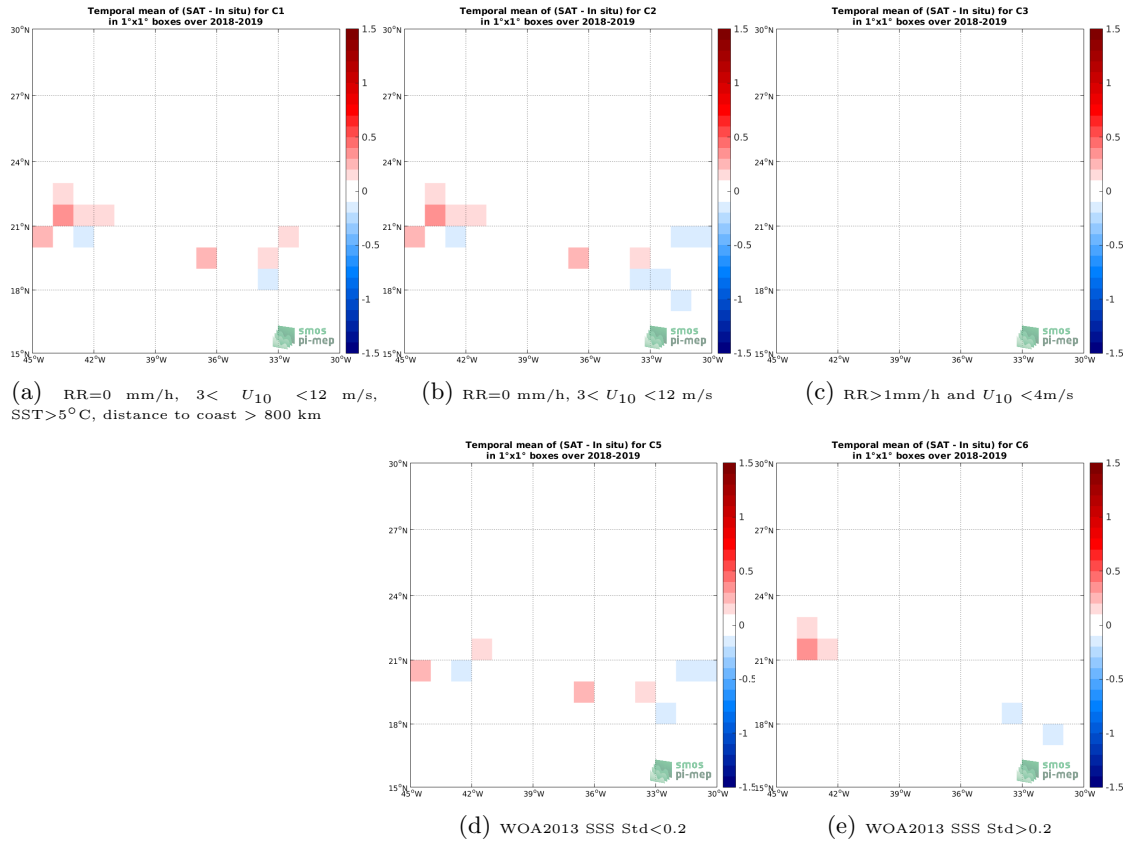
Figure 12: Temporal mean gridded over spatial boxes of size 1^\circ \times 1^\circ of \Delta SSS (SMAP-L3-RSS-V4-8DAY-RUNNING - TSG-SAMOS) for 5 different subdatasets corresponding to: RR=0 mm/h, 3 < U_{10} < 12 m/s, SST > 5^\circ\text{C} , distance to coast > 800 km (a), RR=0 mm/h, 3 < U_{10} < 12 m/s (b), RR > 1 mm/h and U_{10} < 4 m/s (c), WOA2013 SSS Std < 0.2 (d), WOA2013 SSS Std > 0.2 (e).
