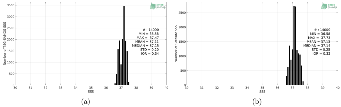
Figure 2: Histograms of SSS from TSG-SAMOS (a) and SMAP-L3-RSS-V4-8DAY-RUNNING (b) considering all match-up pairs per bins of 0.1 over the SPURS 1 Pi-MEP region and for the full satellite product period.
