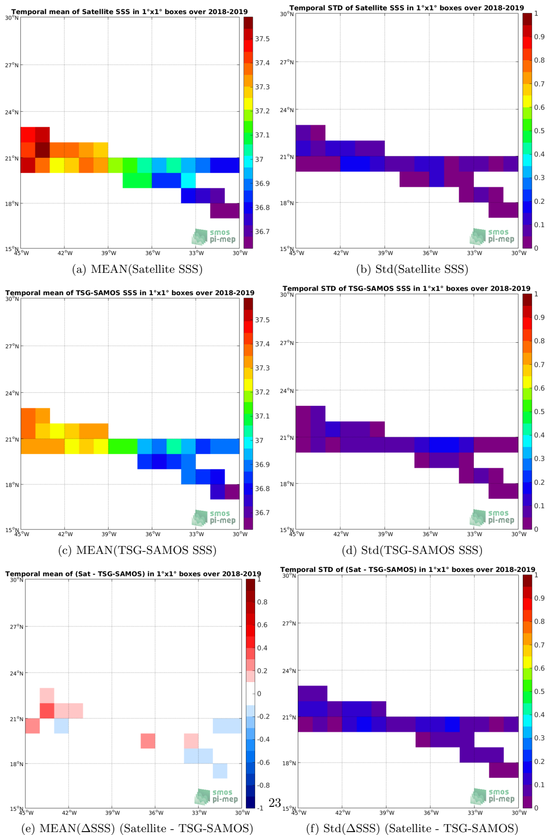
Figure 6: Temporal mean (left) and Std (right) of SSS from SMAP-L3-RSS-V4-8DAY-RUNNING (top), TSG-SAMOS (middle), and of \Delta SSS (Satellite - TSG-SAMOS). Only match-up pairs are used to generate these maps.
