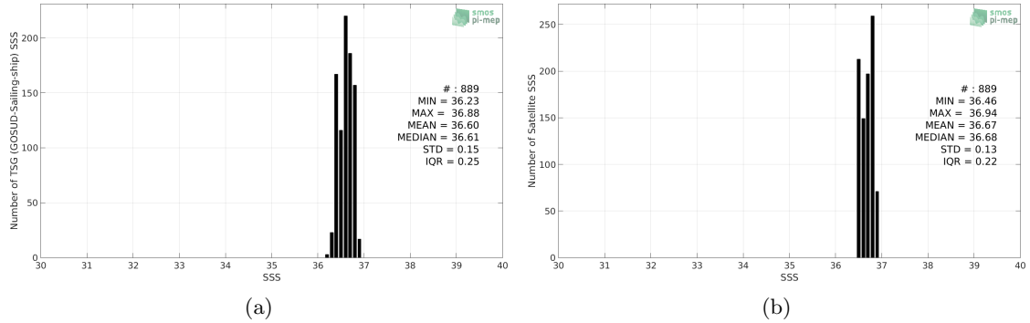
Figure 2: Histograms of SSS from TSG (GOSUD-Sailing-ship) (a) and SMAP SSS L3 v4 - 8-Day running (RSS) (b) considering all match-up pairs per bins of 0.1 over the SPURS 1 Pi-MEP region and for the full satellite product period.
