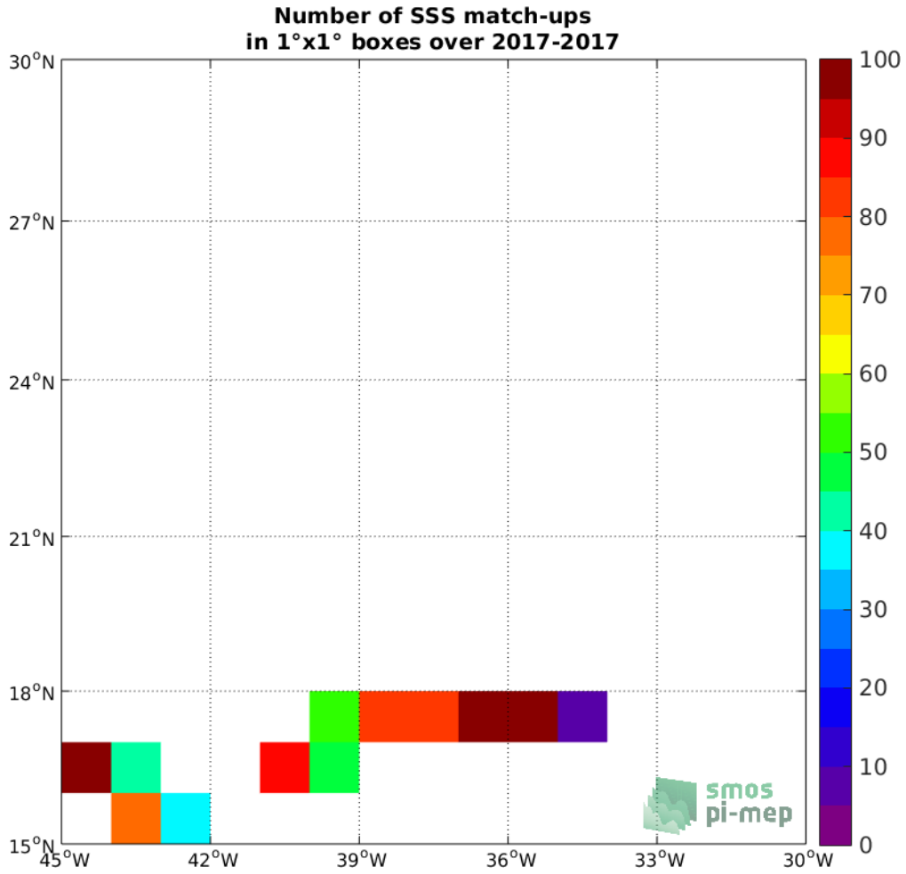
Figure 4: Number of SSS match-ups between TSG (GOSUD-Sailing-ship) SSS and the SMAP SSS L3 v4 - 8-Day running (RSS) SSS product for the SPURS 1 Pi-MEP region over 1°x1° boxes and for the full satellite product period.
