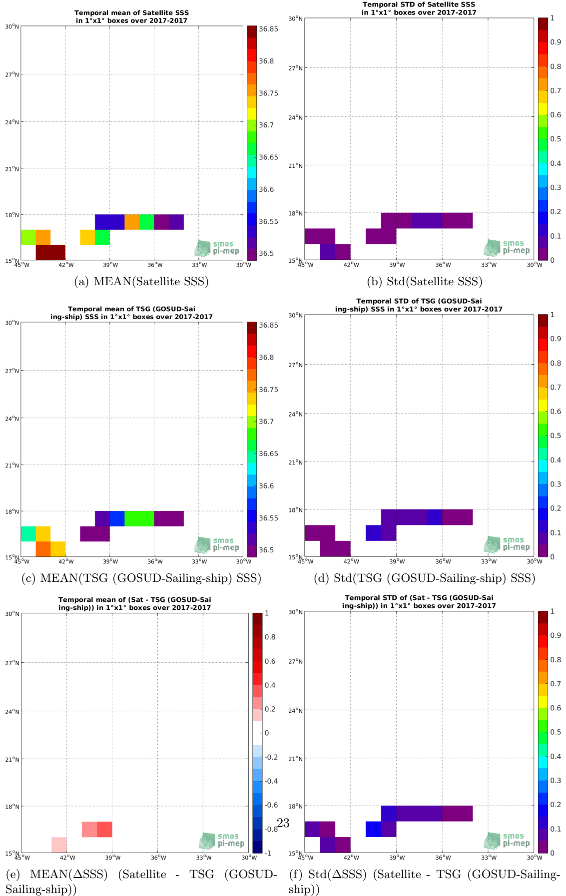
Figure 6: Temporal mean (left) and Std (right) of SSS from SMAP SSS L3 v4 - 8-Day running (RSS) (top), TSG (GOSUD-Sailing-ship) (middle), and of \Delta SSS (Satellite - TSG (GOSUD-Sailing-ship)). Only match-up pairs are used to generate these maps.
