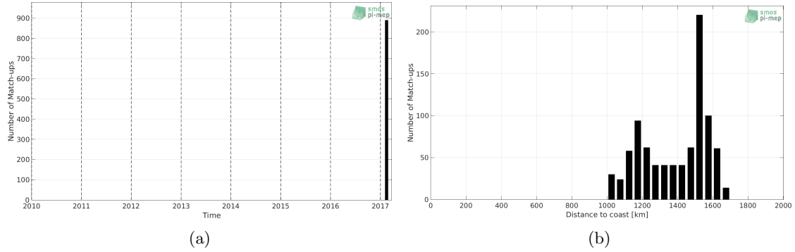
Figure 1: Number of match-ups between TSG (GOSUD-Sailing-ship) and SMAP SSS L3 v4 - 8-Day running (RSS) SSS as a function of time (a) and as function of the distance to coast (b) over the SPURS 1 Pi-MEP region and for the full satellite product period.
