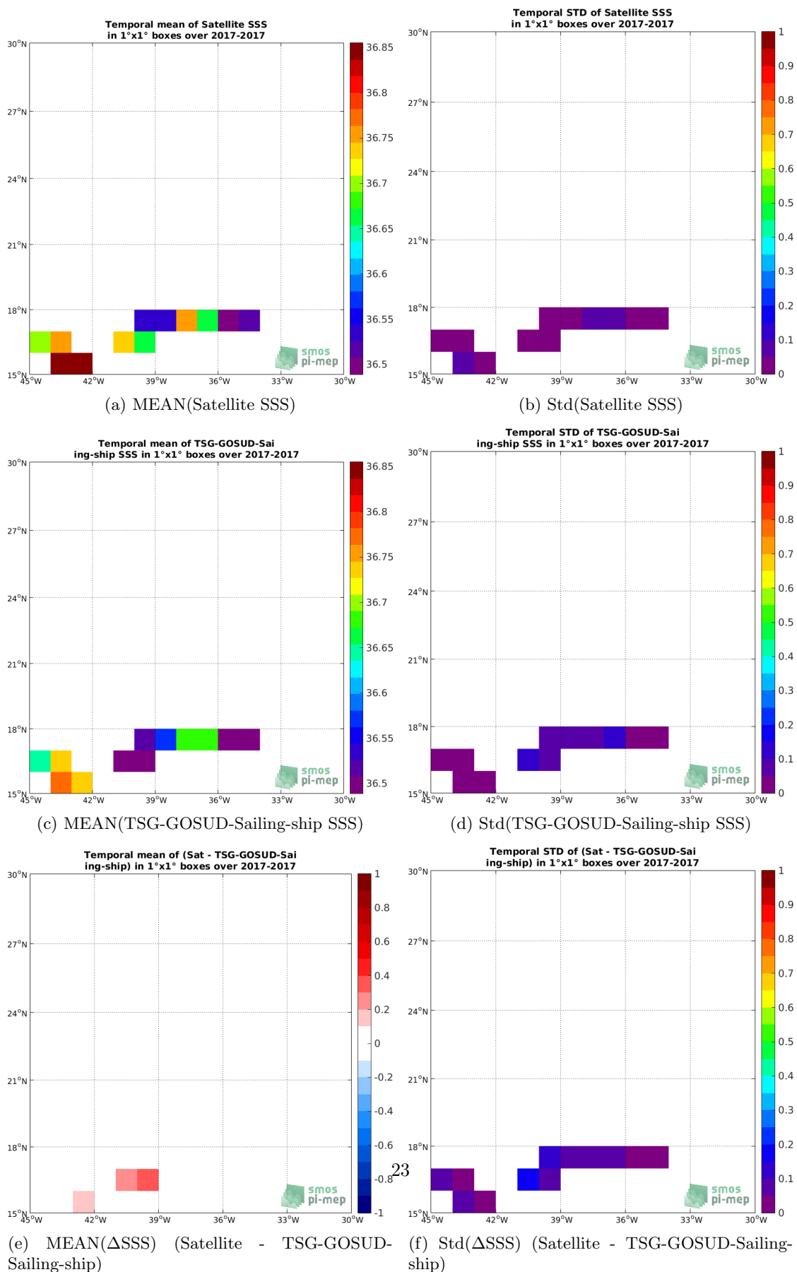
Figure 6: Temporal mean (left) and Std (right) of SSS from SMAP-L3-RSS-V4-8DAY-RUNNING (top), TSG-GOSUD-Sailing-ship (middle), and of \Delta SSS (Satellite - TSG-GOSUD-Sailing-ship). Only match-up pairs are used to generate these maps.
