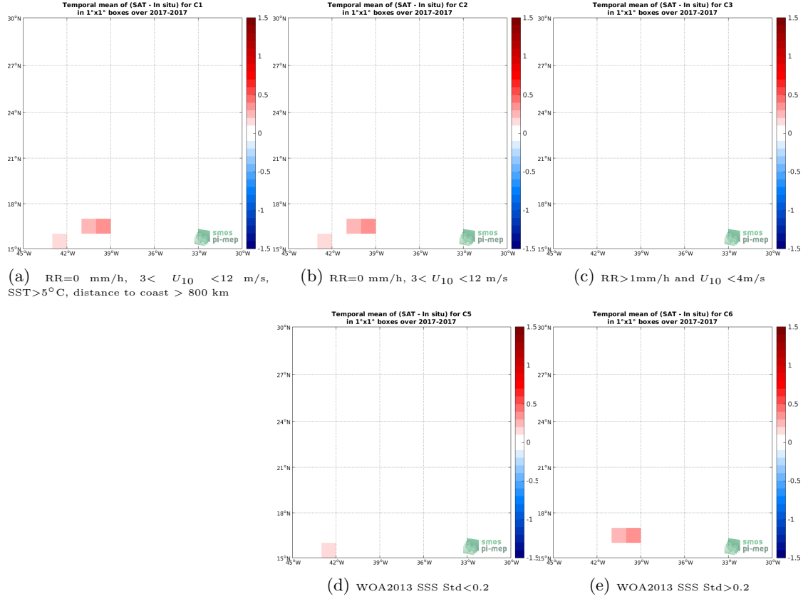
Figure 12: Temporal mean gridded over spatial boxes of size 1°x1° of \Delta SSS (SMAP-L3-RSS-V4-8DAY-RUNNING - TSG-GOSUD-Sailing-ship) for 5 different subdatasets corresponding to: RR=0 mm/h, 3 < U_{10} < 12 m/s, SST > 5°C, distance to coast > 800 km (a), RR=0 mm/h, 3 < U_{10} < 12 m/s (b), RR > 1 mm/h and U_{10} < 4 m/s (c), WOA2013 SSS Std < 0.2 (d), WOA2013 SSS Std > 0.2 (e).
