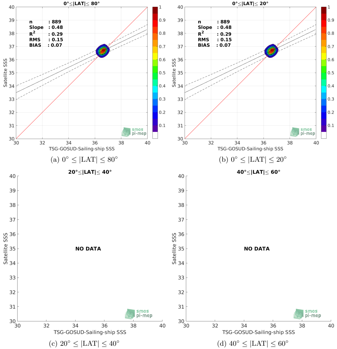
Figure 9: Contour maps of the concentration of SMAP-L3-RSS-V4-8DAY-RUNNING SSS (y-axis) versus TSG-GOSUD-Sailing-ship SSS (x-axis) at match-up pairs for different latitude bands. For each plot, the red line shows x=y . The black thin and dashed lines indicate a linear fit through the data cloud and the \pm 95\% confidence levels, respectively. The number match-up pairs n , the slope and R^2 coefficient of the linear fit, the root mean square (RMS) and the mean bias between satellite and in situ data are indicated for each latitude band in each plots.
