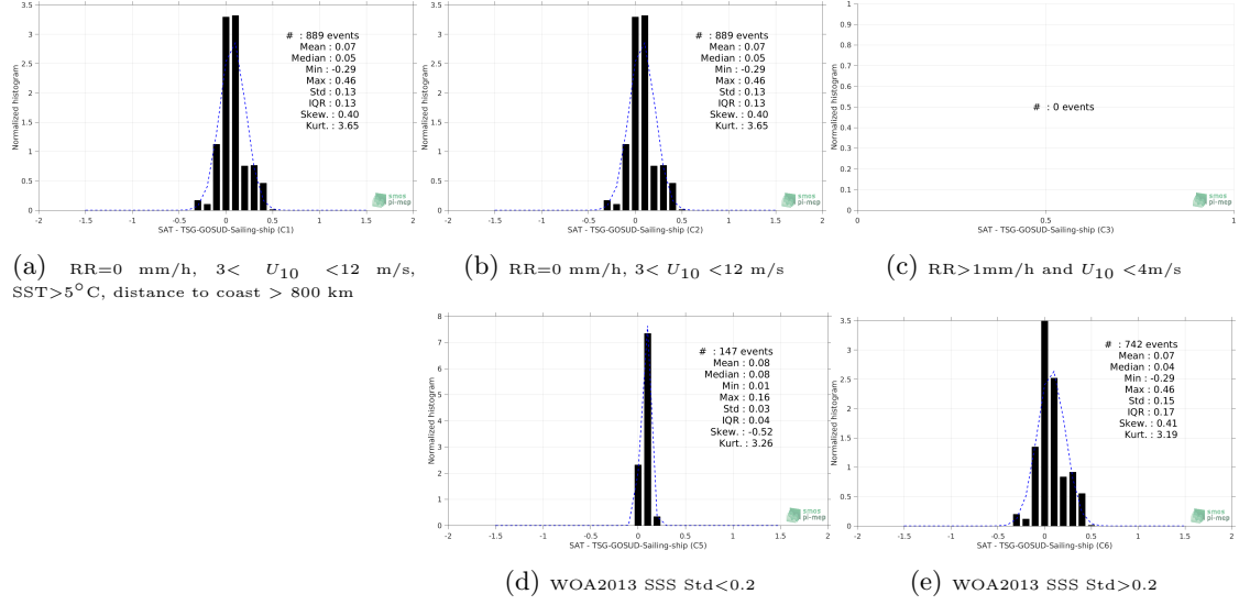
Figure 13: Normalized histogram of \Delta SSS (SMAP-L3-RSS-V4-8DAY-RUNNING - TSG-GOSUD-Sailing-ship) for 5 different subdatasets corresponding to: RR=0 mm/h, 3 < U_{10} < 12 m/s, SST>5°C, distance to coast > 800 km (a), RR=0 mm/h, 3 < U_{10} < 12 m/s (b), RR>1mm/h and U_{10} < 4 m/s (c), WOA2013 SSS Std<0.2 (d), WOA2013 SSS Std>0.2 (e).
