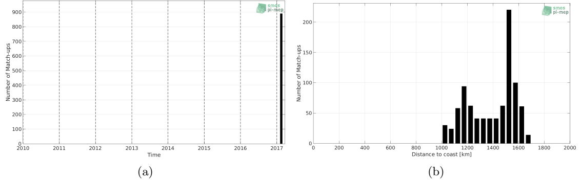
Figure 1: Number of match-ups between TSG-GOSUD-Sailing-ship and SMAP-L3-RSS-V4-8DAY-RUNNING SSS as a function of time (a) and as function of the distance to coast (b) over the SPURS 1 Pi-MEP region and for the full satellite product period.
