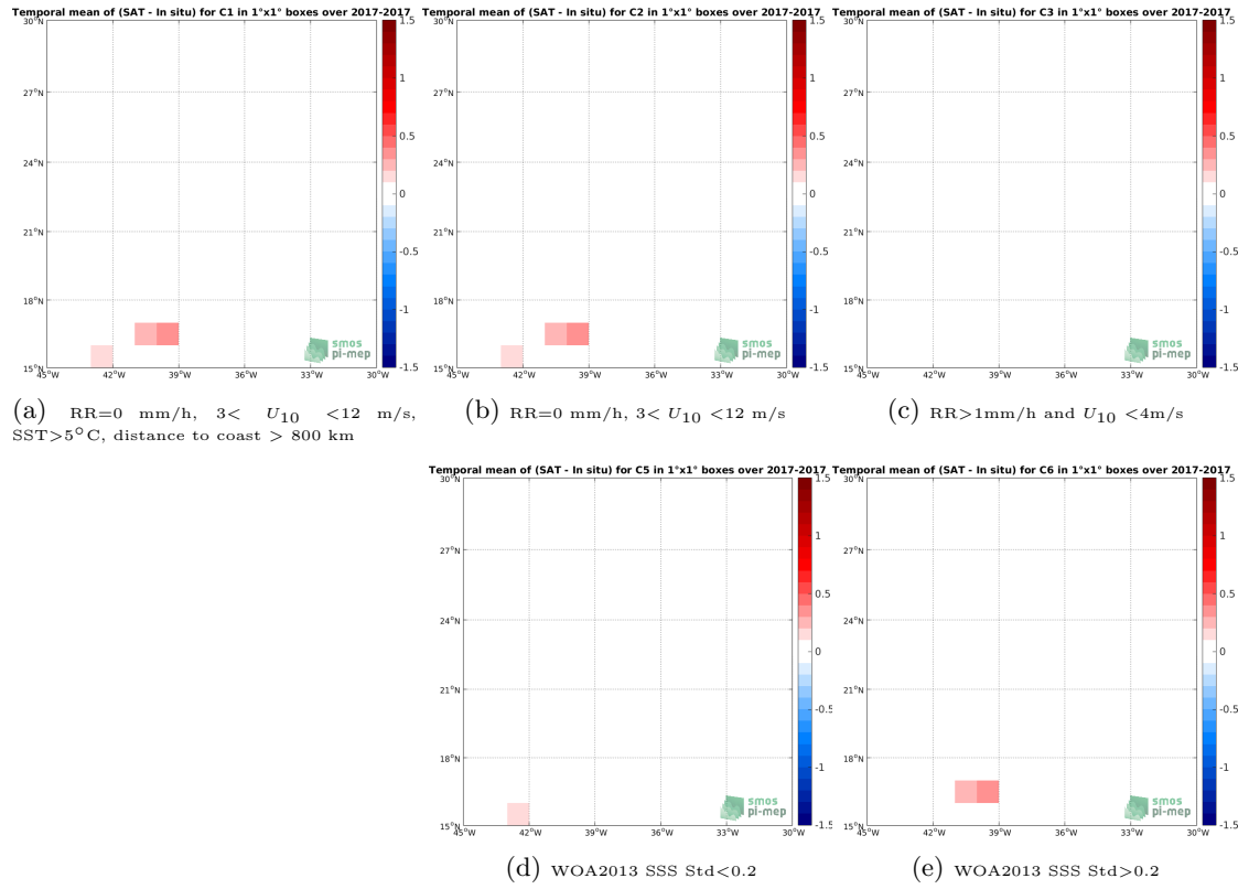
Figure 12: Temporal mean gridded over spatial boxes of size 1^\circ \times 1^\circ of \Delta SSS (SMAP-L3-RSS-V4-8DAY-RUNNING - TSG-GOSUD-Sailing-ship) for 5 different subdatasets corresponding to: RR=0 mm/h, 3 < U_{10} < 12 m/s, SST >5^\circ\text{C} , distance to coast > 800 km (a), RR=0 mm/h, 3 < U_{10} < 12 m/s (b), RR >1 mm/h and U_{10} < 4 m/s (c), WOA2013 SSS Std <0.2 (d), WOA2013 SSS Std >0.2 (e).
