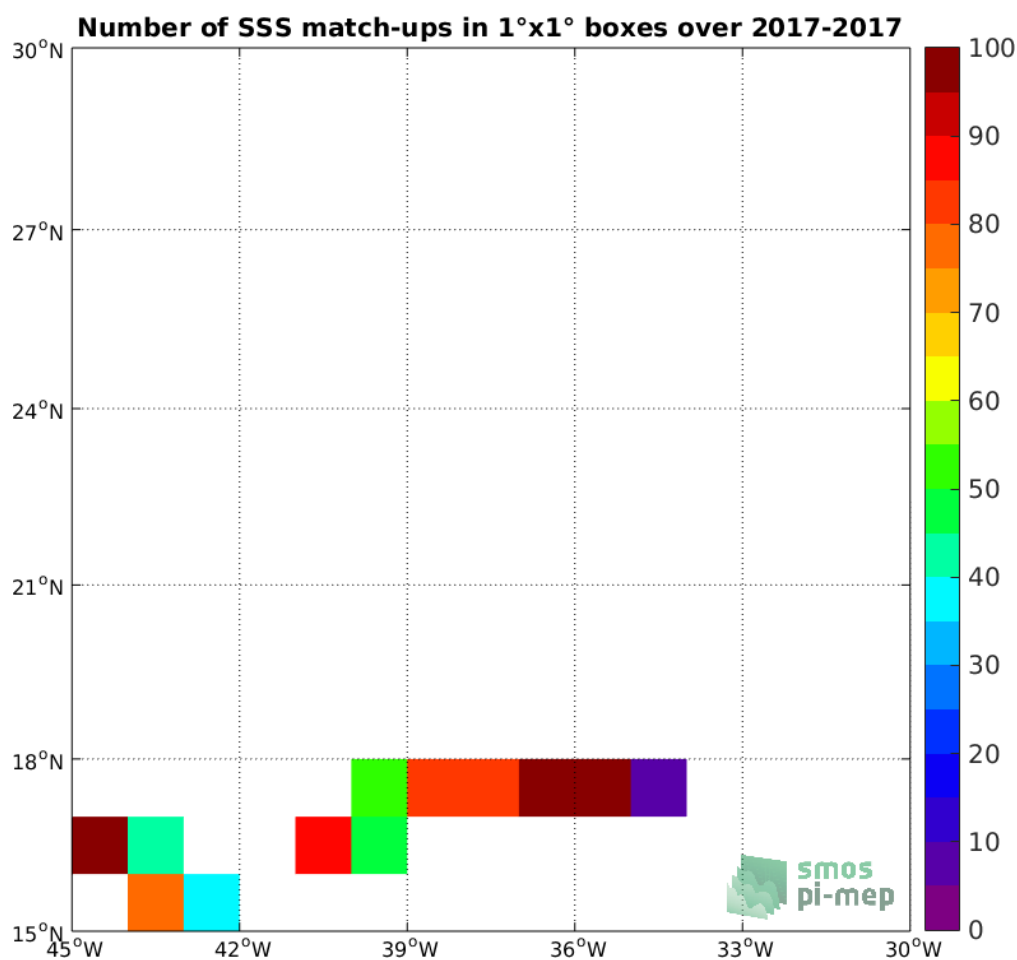
Figure 4: Number of SSS match-ups between TSG-GOSUD-Sailing-ship SSS and the SMAP-L3-RSS-V4-8DAY-RUNNING SSS product for the SPURS 1 Pi-MEP region over 1°x1° boxes and for the full satellite product period.
