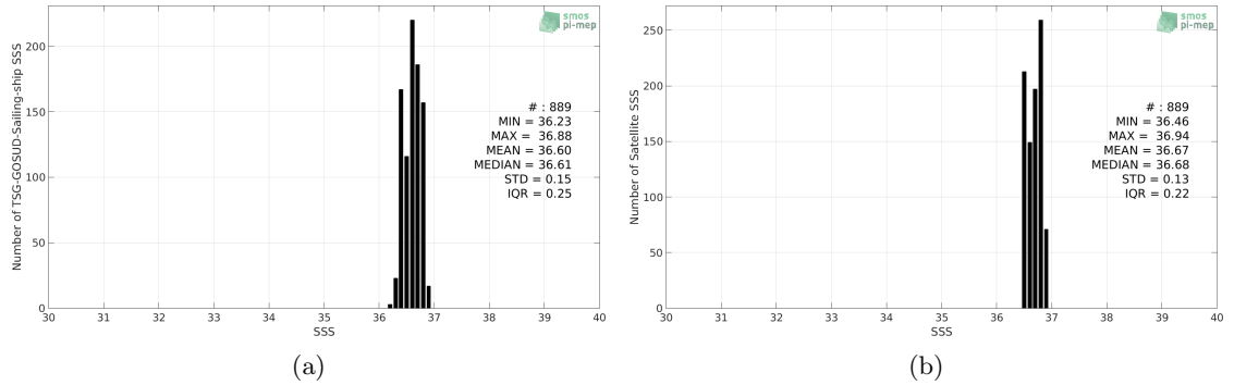
Figure 2: Histograms of SSS from TSG-GOSUD-Sailing-ship (a) and SMAP-L3-RSS-V4-8DAY-RUNNING (b) considering all match-up pairs per bins of 0.1 over the SPURS 1 Pi-MEP region and for the full satellite product period.
