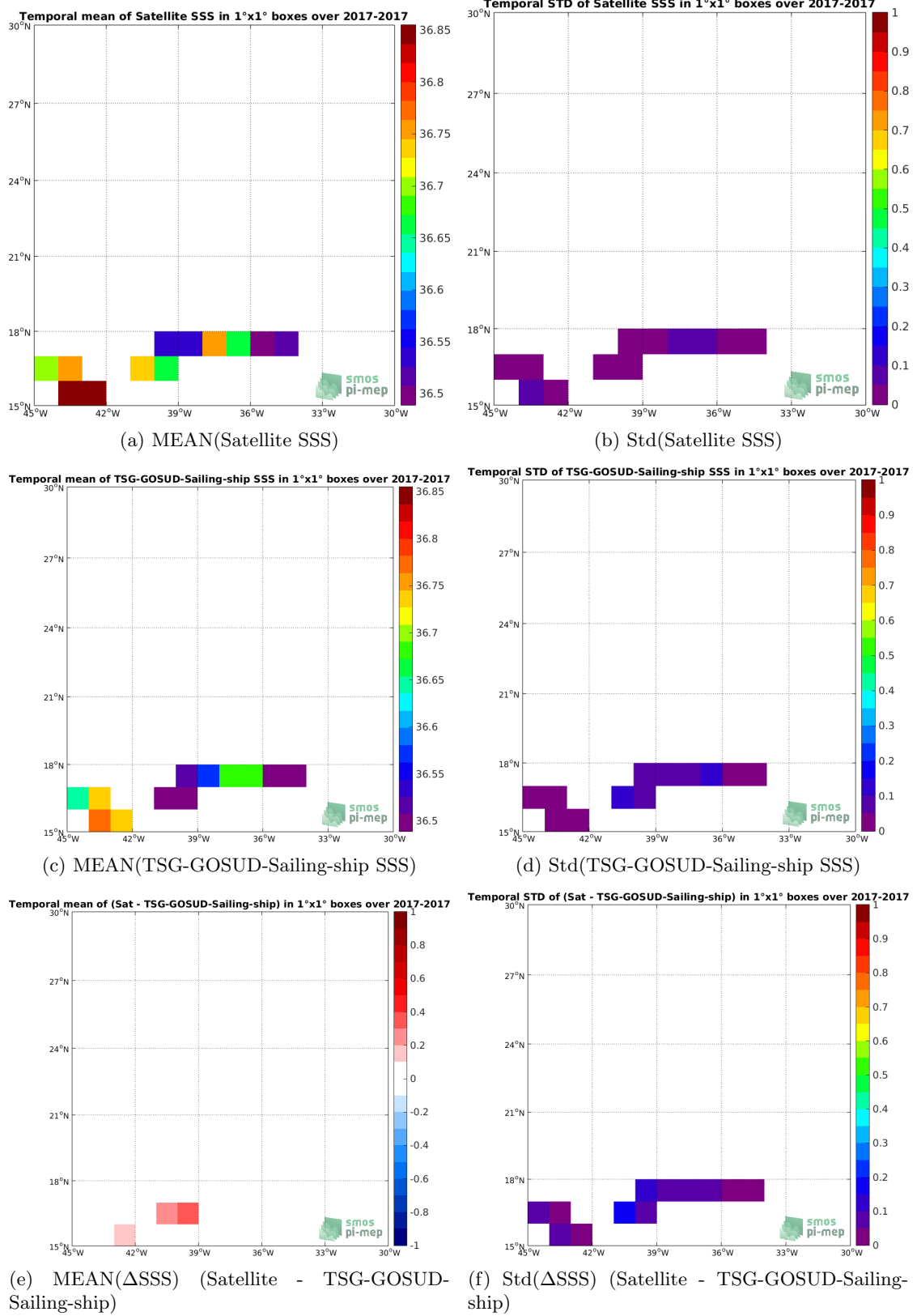
Figure 6: Temporal mean (left) and Std (right) of SSS from SMAP-L3-RSS-V4-8DAY-RUNNING (top), TSG-GOSUD-Sailing-ship (middle), and of \Delta SSS (Satellite - TSG-GOSUD-Sailing-ship). Only match-up pairs are used to generate these maps.
