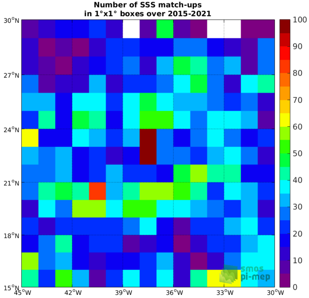
Figure 4: Number of SSS match-ups between Argo SSS and the SMAP SSS L3 v4 - 8-Day running (RSS) SSS product for the SPURS 1 Pi-MEP region over 1^\circ \times 1^\circ boxes and for the full satellite product period.
