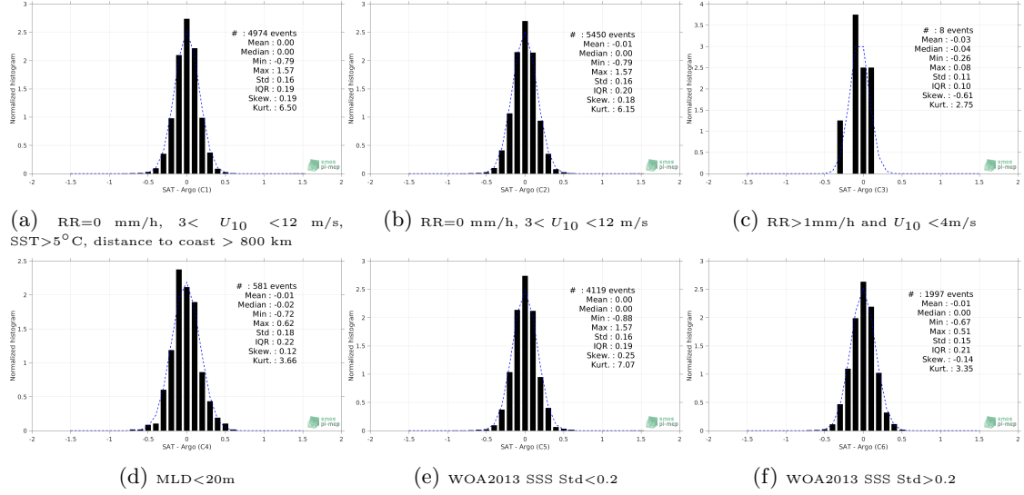
Figure 13: Normalized histogram of \Delta\text{SSS} (SMAP SSS L3 v4 - 8-Day running (RSS) - Argo) for 6 different subdatasets corresponding to: RR=0 mm/h, 3 < U_{10} < 12 m/s, SST>5°C, distance to coast > 800 km (a), RR=0 mm/h, 3 < U_{10} < 12 m/s (b), RR>1mm/h and U_{10} < 4 m/s (c), MLD<20m (d), WOA2013 SSS Std<0.2 (e), WOA2013 SSS Std>0.2 (f).
