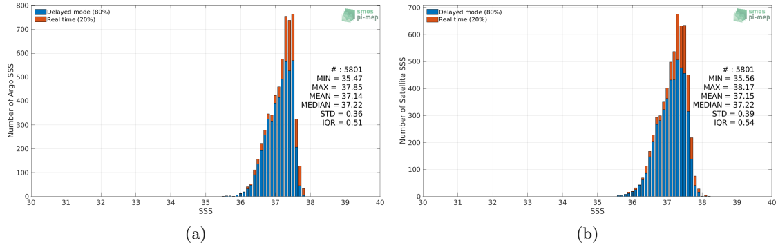
Figure 2: Histograms of SSS from Argo (a) and SMAP SSS L3 v4 - 8-Day running (RSS) (b) considering all match-up pairs per bins of 0.1 over the SPURS 1 Pi-MEP region and for the full satellite product period.
