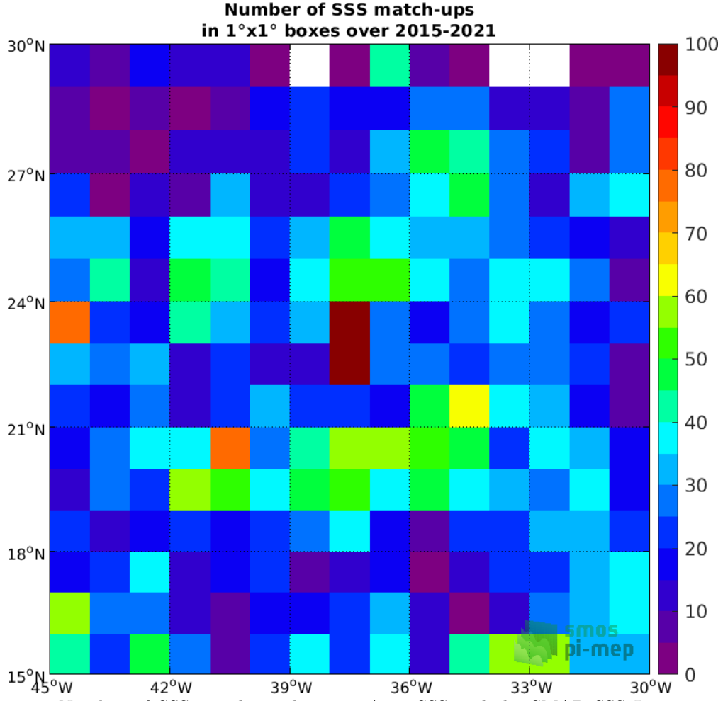
Figure 4: Number of SSS match-ups between Argo SSS and the SMAP SSS L3 v4 - 8-Day running (RSS) SSS product for the SPURS 1 Pi-MEP region over 1°x1° boxes and for the full satellite product period.
