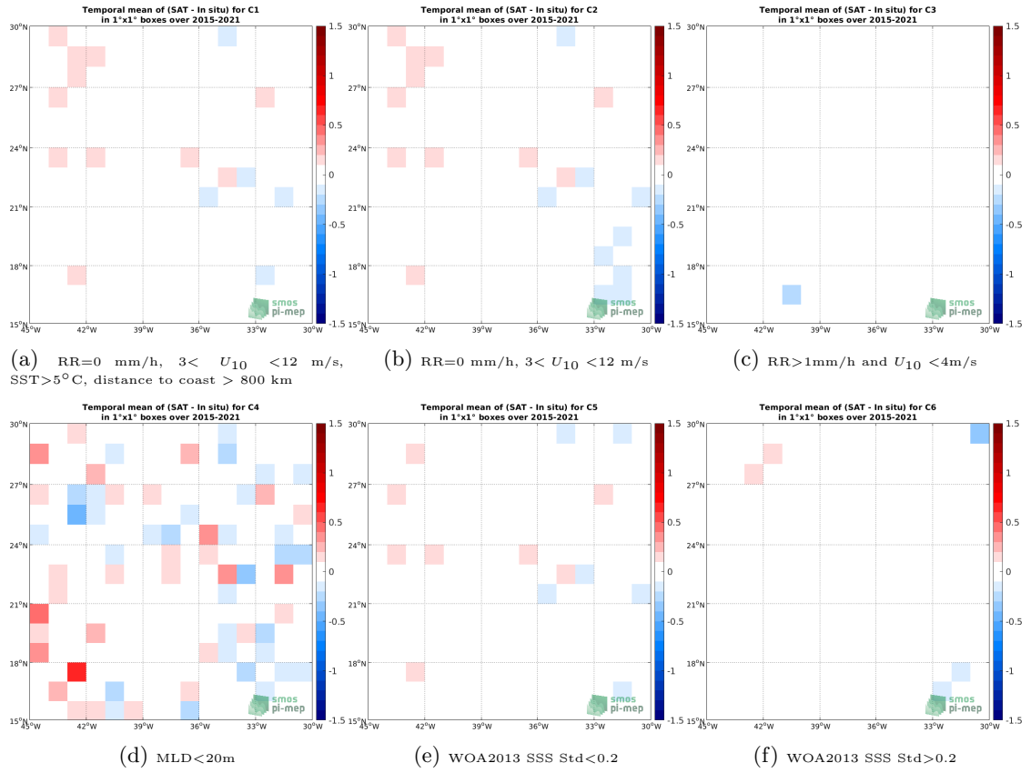
Figure 12: Temporal mean gridded over spatial boxes of size 1^\circ \times 1^\circ of \Delta SSS (SMAP SSS L3 v4 - 8-Day running (RSS) - Argo) for 6 different subdatasets corresponding to:RR=0 mm/h, 3 < U_{10} < 12 m/s, SST >5^\circ C, distance to coast > 800 km (a), RR=0 mm/h, 3 < U_{10} < 12 m/s (b), RR >1 mm/h and U_{10} < 4 m/s (c),MLD <20 m (d),WOA2013 SSS Std <0.2 (e),WOA2013 SSS Std >0.2 (f).
