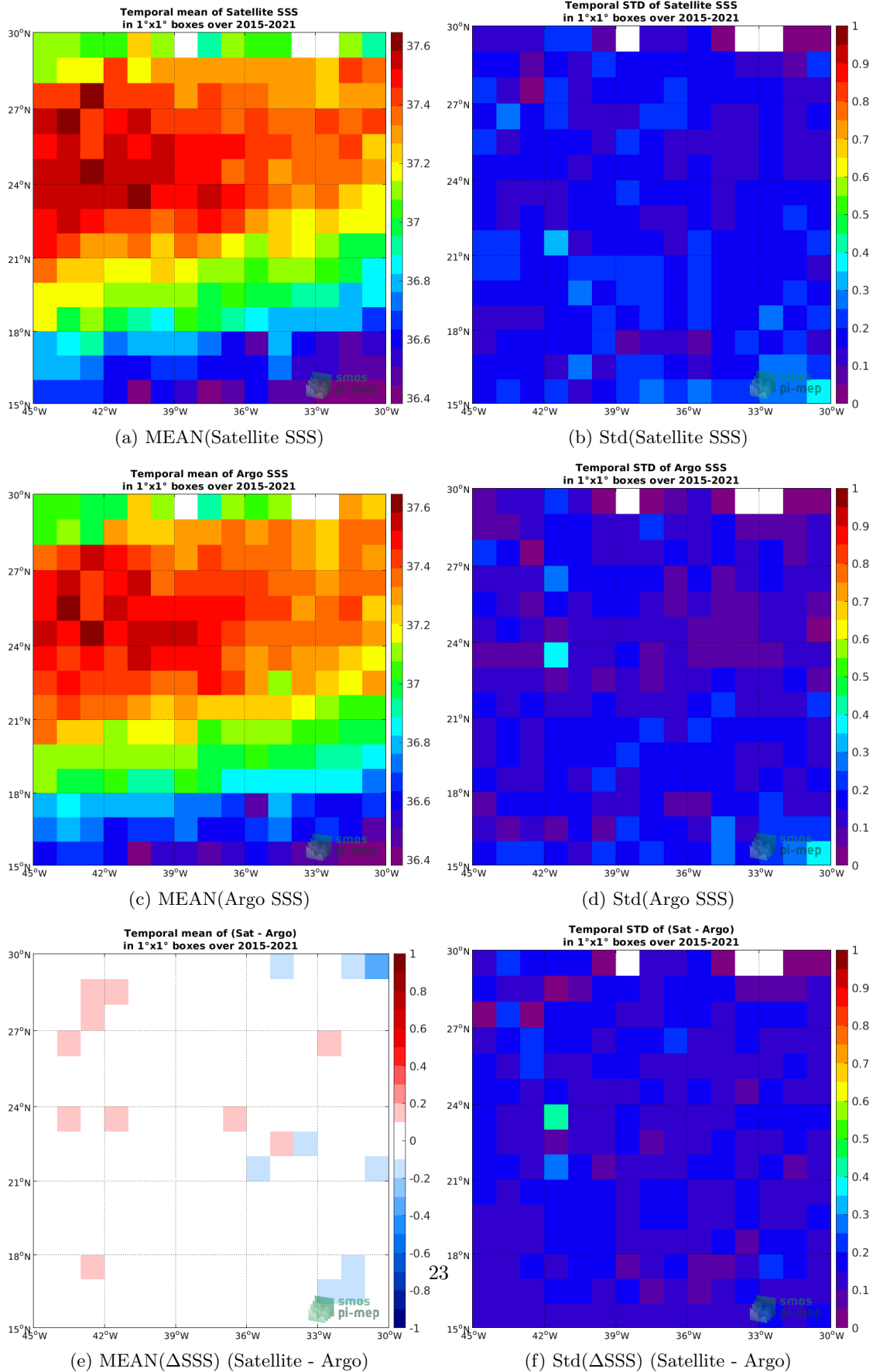
Figure 6: Temporal mean (left) and Std (right) of SSS from SMAP SSS L3 v4 - 8-Day running (RSS) (top), Argo (middle), and of \Delta SSS (Satellite - Argo). Only match-up pairs are used to generate these maps.
