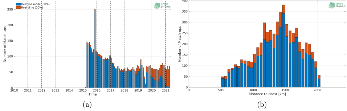
Figure 1: Number of match-ups between Argo and SMAP SSS L3 v4 - 8-Day running (RSS) SSS as a function of time (a) and as function of the distance to coast (b) over the SPURS 1 Pi-MEP region and for the full satellite product period.
