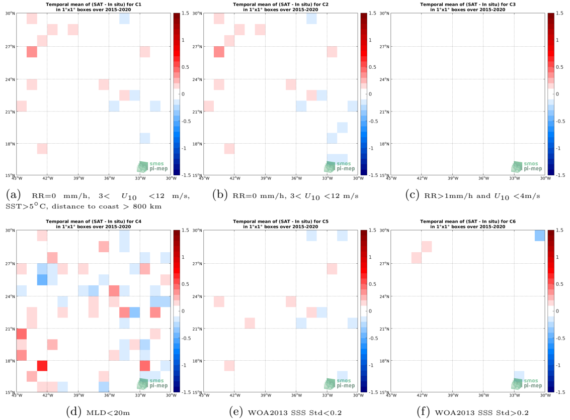
Figure 12: Temporal mean gridded over spatial boxes of size 1^\circ \times 1^\circ of \Delta SSS (SMAP SSS L3 v4 - 8-Day running (RSS) - Argo) for 6 different subdatasets corresponding to: RR=0 mm/h, 3 < U_{10} < 12 m/s, SST > 5^\circ\text{C} , distance to coast > 800 km (a), RR=0 mm/h, 3 < U_{10} < 12 m/s (b), RR > 1 mm/h and U_{10} < 4 m/s (c), MLD < 20 m (d), WOA2013 SSS Std < 0.2 (e), WOA2013 SSS Std > 0.2 (f).
