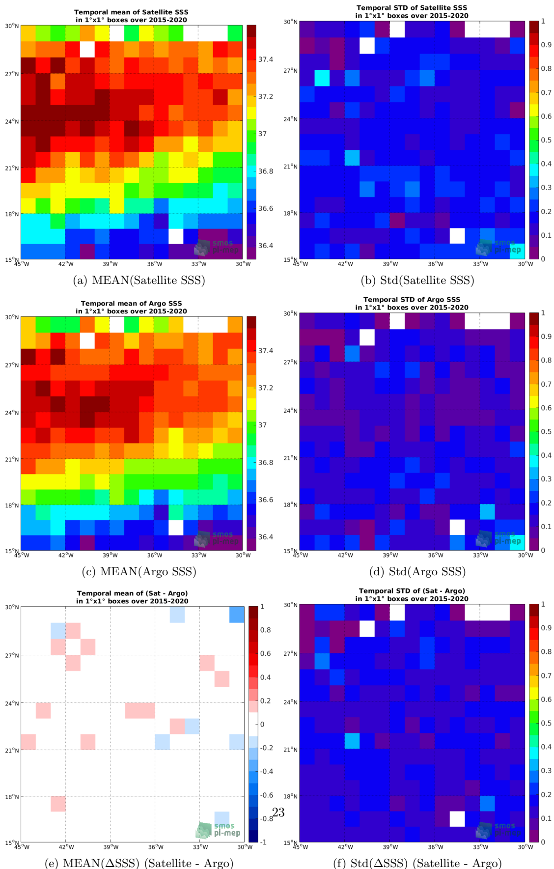
Figure 6: Temporal mean (left) and Std (right) of SSS from SMAP-L3-RSS-V4-8DAY-RUNNING (top), Argo (middle), and of \Delta SSS (Satellite - Argo). Only match-up pairs are used to generate these maps.
