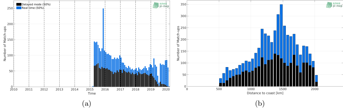
Figure 1: Number of match-ups between Argo and SMAP-L3-RSS-V4-8DAY-RUNNING SSS as a function of time (a) and as function of the distance to coast (b) over the SPURS 1 Pi-MEP region and for the full satellite product period.
