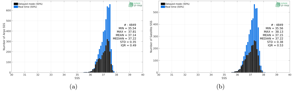
Figure 2: Histograms of SSS from Argo (a) and SMAP-L3-RSS-V4-8DAY-RUNNING (b) considering all match-up pairs per bins of 0.1 over the SPURS 1 Pi-MEP region and for the full satellite product period.
