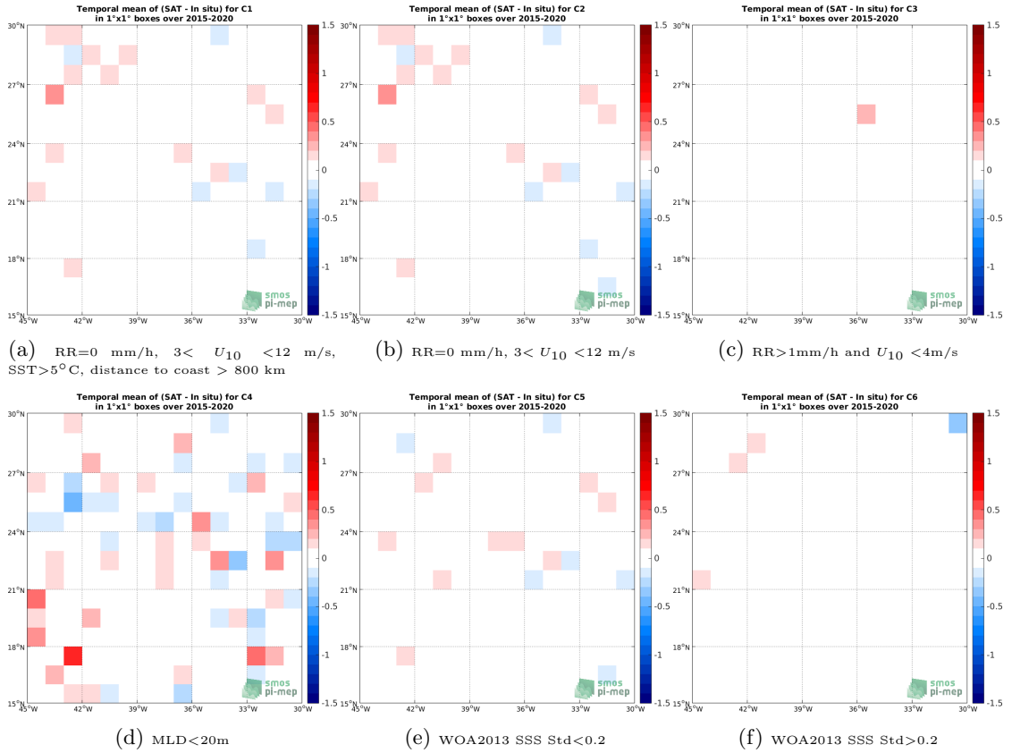
Figure 12: Temporal mean gridded over spatial boxes of size 1^\circ \times 1^\circ of \Delta SSS (SMAP-L3-RSS-V4-8DAY-RUNNING - Argo) for 6 different subdatasets corresponding to:RR=0 mm/h, 3 < U_{10} < 12 m/s, SST>5°C, distance to coast > 800 km (a), RR=0 mm/h, 3 < U_{10} < 12 m/s (b), RR>1mm/h and U_{10} < 4 m/s (c),MLD<20m (d),WOA2013 SSS Std<0.2 (e),WOA2013 SSS Std>0.2 (f).
