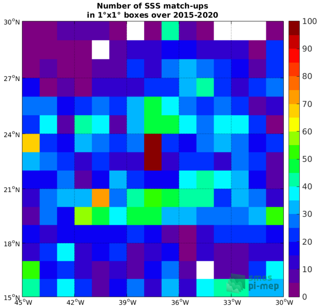
Figure 4: Number of SSS match-ups between Argo SSS and the SMAP-L3-RSS-V4-8DAY-RUNNING SSS product for the SPURS 1 Pi-MEP region over 1°x1° boxes and for the full satellite product period.
