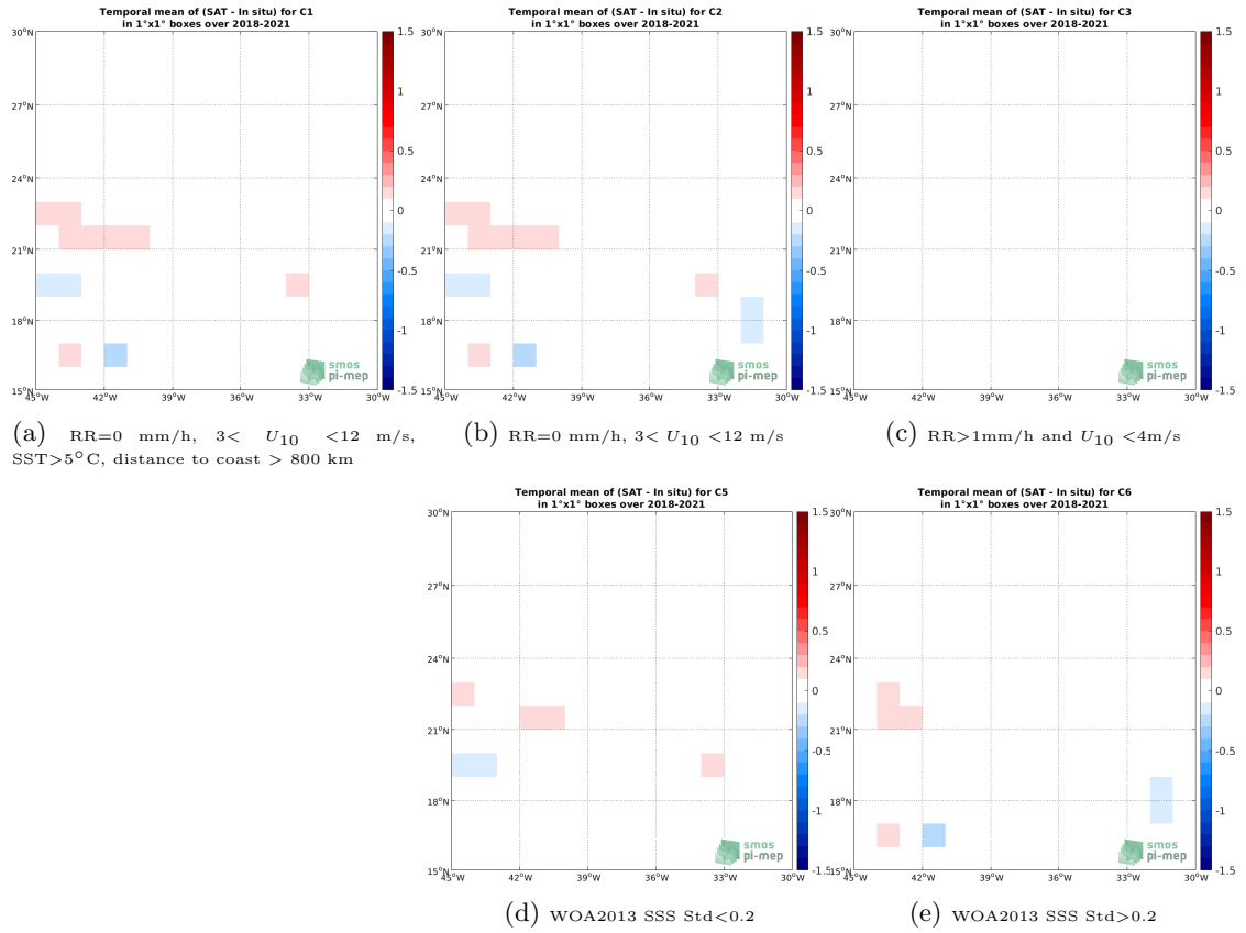
Figure 12: Temporal mean gridded over spatial boxes of size 1^\circ \times 1^\circ of \Delta SSS (SMAP SSS L3 v4 - Monthly (RSS) - TSG (SAMOS)) for 5 different subdatasets corresponding to: RR=0 mm/h, 3 < U_{10} < 12 m/s, SST > 5^\circ\text{C} , distance to coast > 800 km (a), RR=0 mm/h, 3 < U_{10} < 12 m/s (b), RR > 1 mm/h and U_{10} < 4 m/s (c), WOA2013 SSS Std < 0.2 (d), WOA2013 SSS Std > 0.2 (e).
