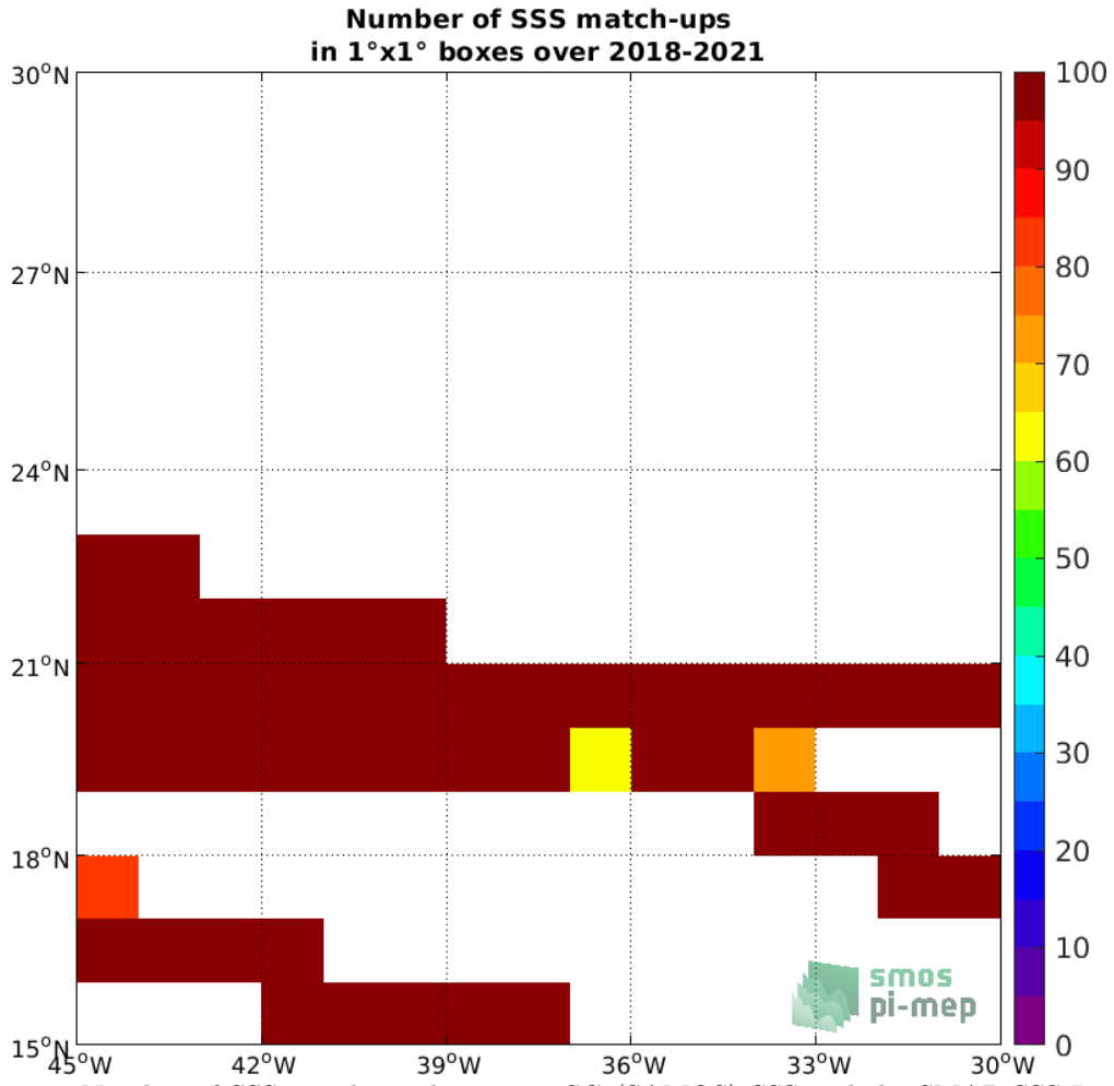
Figure 4: Number of SSS match-ups between TSG (SAMOS) SSS and the SMAP SSS L3 v4 - Monthly (RSS) SSS product for the SPURS 1 Pi-MEP region over 1°x1° boxes and for the full satellite product period.
