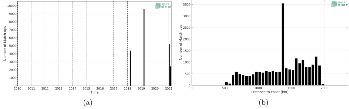
Figure 1: Number of match-ups between TSG (SAMOS) and SMAP SSS L3 v4 - Monthly (RSS) SSS as a function of time (a) and as function of the distance to coast (b) over the SPURS 1 Pi-MEP region and for the full satellite product period.
