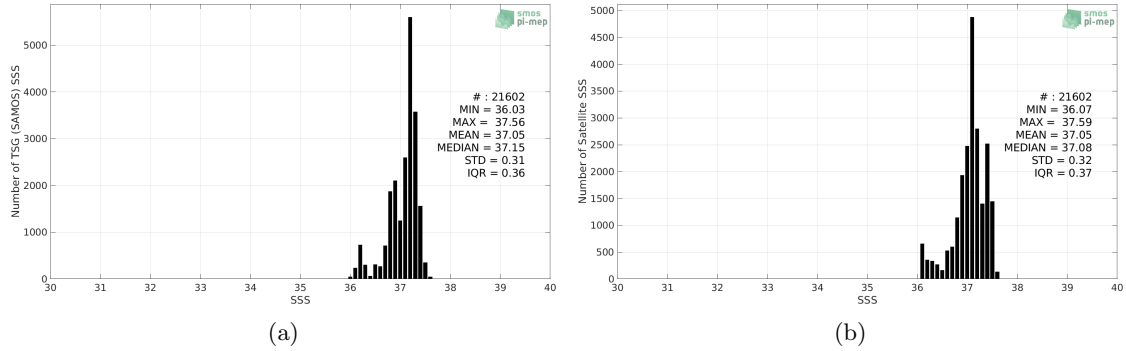
Figure 2: Histograms of SSS from TSG (SAMOS) (a) and SMAP SSS L3 v4 - Monthly (RSS) (b) considering all match-up pairs per bins of 0.1 over the SPURS 1 Pi-MEP region and for the full satellite product period.
