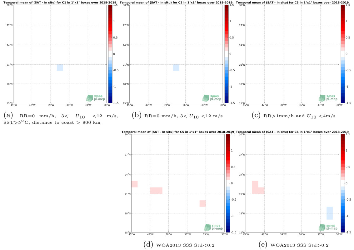
Figure 12: Temporal mean gridded over spatial boxes of size 1^\circ \times 1^\circ of \Delta SSS (SMAP-L3-RSS-V4-MONTHLY - TSG-SAMOS) for 5 different subdatasets corresponding to: RR=0 mm/h, 3 < U_{10} < 12 m/s, SST > 5^\circ\text{C} , distance to coast > 800 km (a), RR=0 mm/h, 3 < U_{10} < 12 m/s (b), RR > 1 mm/h and U_{10} < 4 m/s (c), WOA2013 SSS Std < 0.2 (d), WOA2013 SSS Std > 0.2 (e).
