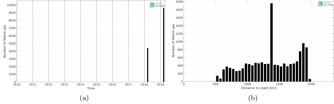
Figure 1: Number of match-ups between TSG-SAMOS and SMAP-L3-RSS-V4-MONTHLY SSS as a function of time (a) and as function of the distance to coast (b) over the SPURS 1 Pi-MEP region and for the full satellite product period.
