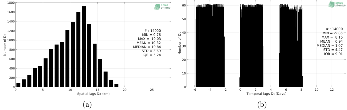
Figure 5: Histograms of the spatial (a) and temporal (b) lags between the time of the TSG-SAMOS measurements and the date of the corresponding SMAP-L3-RSS-V4-MONTHLY SSS product.
