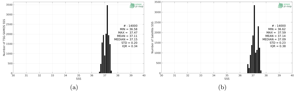
Figure 2: Histograms of SSS from TSG-SAMOS (a) and SMAP-L3-RSS-V4-MONTHLY (b) considering all match-up pairs per bins of 0.1 over the SPURS 1 Pi-MEP region and for the full satellite product period.
