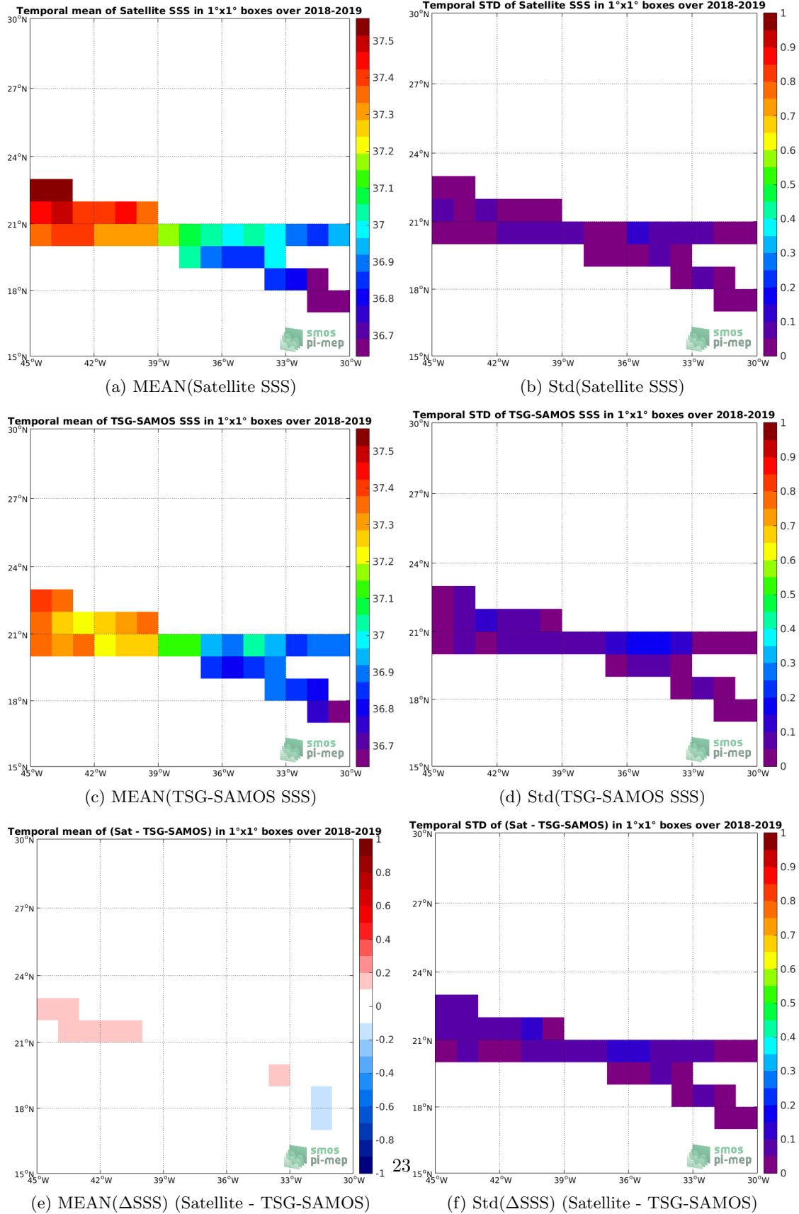
Figure 6: Temporal mean (left) and Std (right) of SSS from SMAP-L3-RSS-V4-MONTHLY (top), TSG-SAMOS (middle), and of \Delta SSS (Satellite - TSG-SAMOS). Only match-up pairs are used to generate these maps.
