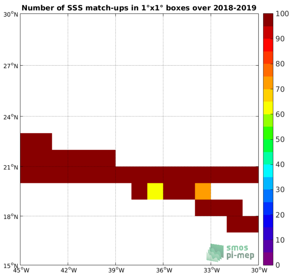
Figure 4: Number of SSS match-ups between TSG-SAMOS SSS and the SMAP-L3-RSS-V4-MONTHLY SSS product for the SPURS 1 Pi-MEP region over 1°x1° boxes and for the full satellite product period.
