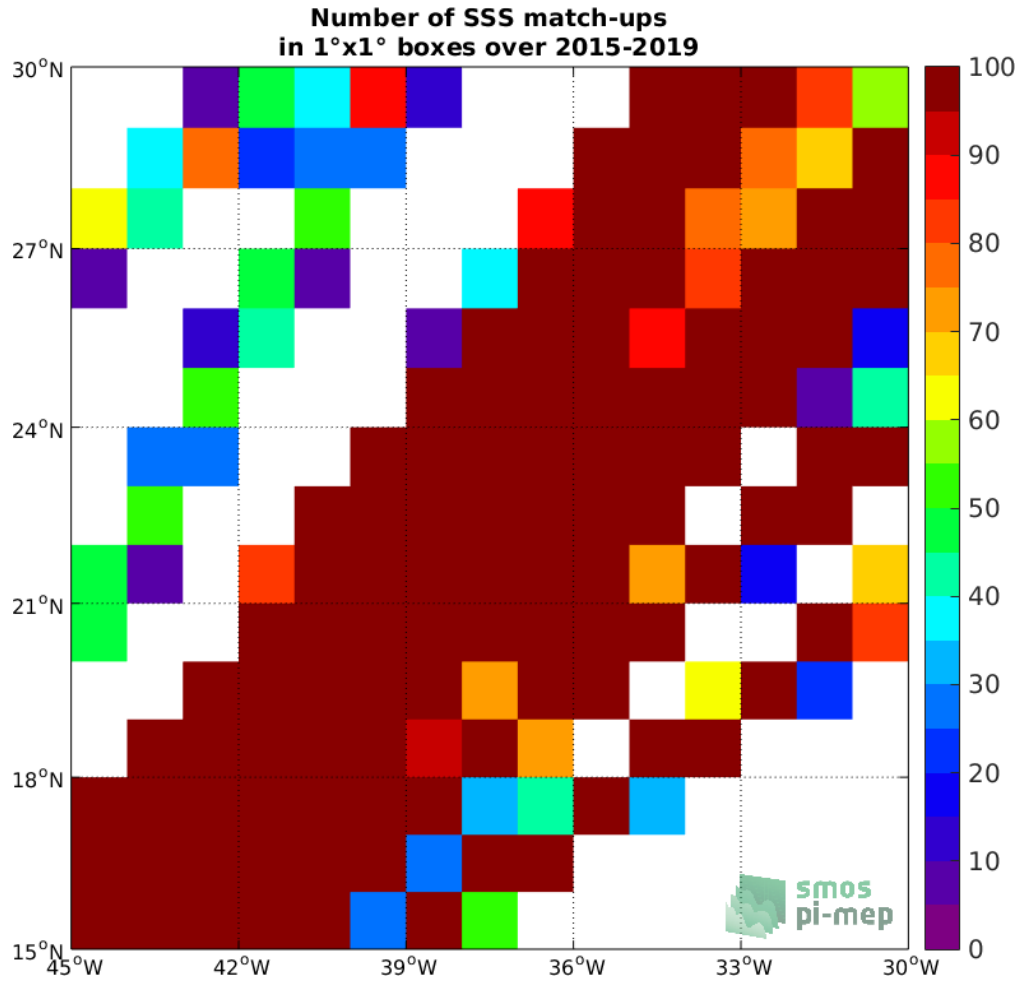
Figure 4: Number of SSS match-ups between TSG (LEGOS-DM) SSS and the SMAP SSS L3 v4 - Monthly (RSS) SSS product for the SPURS 1 Pi-MEP region over 1°×1° boxes and for the full satellite product period.
