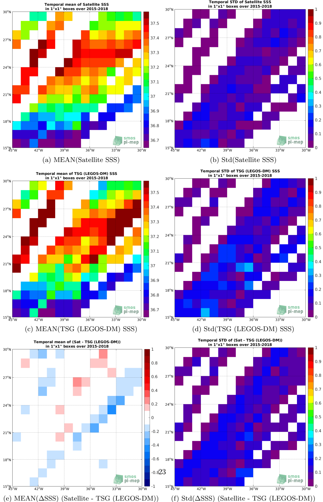
Figure 6: Temporal mean (left) and Std (right) of SSS from SMAP SSS L3 v4 - Monthly (RSS) (top), TSG (LEGOS-DM) (middle), and of \Delta SSS (Satellite - TSG (LEGOS-DM)). Only match-up pairs are used to generate these maps.
