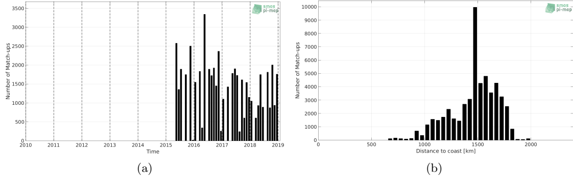
Figure 1: Number of match-ups between TSG-LEGOS-DM and SMAP-L3-RSS-V4-MONTHLY SSS as a function of time (a) and as function of the distance to coast (b) over the SPURS 1 Pi-MEP region and for the full satellite product period.
