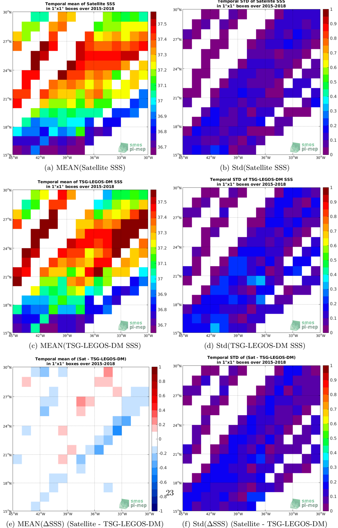
Figure 6: Temporal mean (left) and Std (right) of SSS from SMAP-L3-RSS-V4-MONTHLY (top), TSG-LEGOS-DM (middle), and of \Delta SSS (Satellite - TSG-LEGOS-DM). Only match-up pairs are used to generate these maps.
