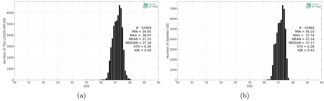
Figure 2: Histograms of SSS from TSG-LEGOS-DM (a) and SMAP-L3-RSS-V4-MONTHLY (b) considering all match-up pairs per bins of 0.1 over the SPURS 1 Pi-MEP region and for the full satellite product period.
