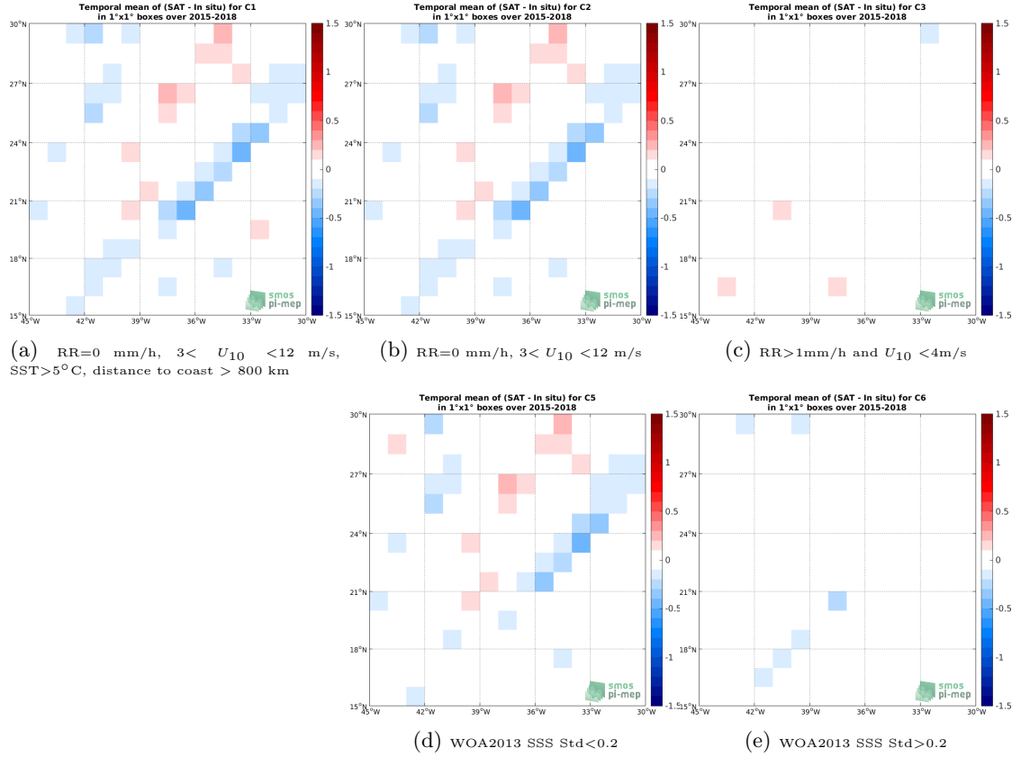
Figure 12: Temporal mean gridded over spatial boxes of size 1^\circ \times 1^\circ of \Delta SSS (SMAP-L3-RSS-V4-MONTHLY - TSG-LEGOS-DM) for 5 different subdatasets corresponding to:RR=0 mm/h, 3 < U_{10} < 12 m/s, SST>5°C, distance to coast > 800 km (a), RR=0 mm/h, 3 < U_{10} < 12 m/s (b), RR>1mm/h and U_{10} < 4 m/s (c), WOA2013 SSS Std<0.2 (d), WOA2013 SSS Std>0.2 (e).
