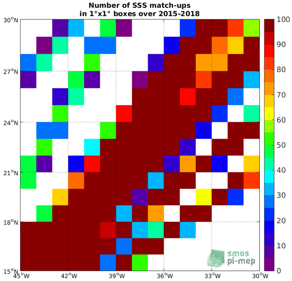
Figure 4: Number of SSS match-ups between TSG-LEGOS-DM SSS and the SMAP-L3-RSS-V4-MONTHLY SSS product for the SPURS 1 Pi-MEP region over 1°x1° boxes and for the full satellite product period.
