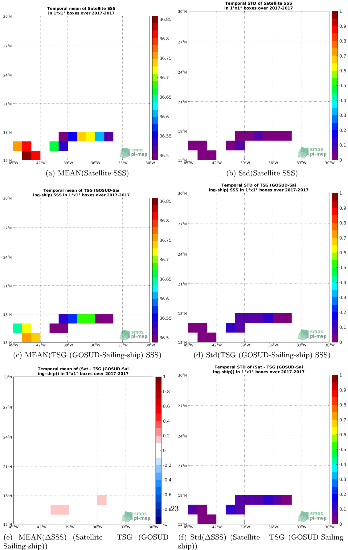
Figure 6: Temporal mean (left) and Std (right) of SSS from SMAP SSS L3 v4 - Monthly (RSS) (top), TSG (GOSUD-Sailing-ship) (middle), and of \Delta SSS (Satellite - TSG (GOSUD-Sailing-ship)). Only match-up pairs are used to generate these maps.
