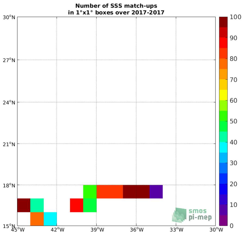
Figure 4: Number of SSS match-ups between TSG (GOSUD-Sailing-ship) SSS and the SMAP SSS L3 v4 - Monthly (RSS) SSS product for the SPURS 1 Pi-MEP region over 1°x1° boxes and for the full satellite product period.
