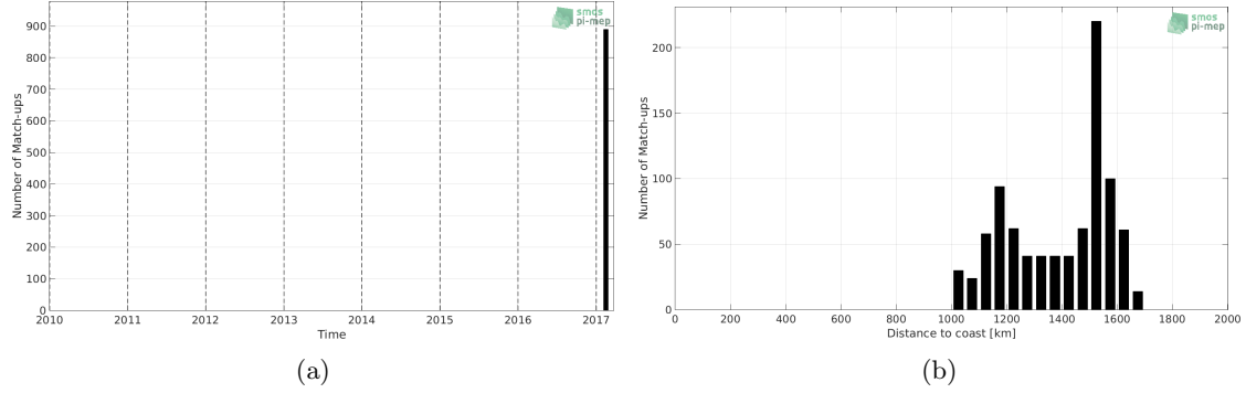
Figure 1: Number of match-ups between TSG-GOSUD-Sailing-ship and SMAP-L3-RSS-V4-MONTHLY SSS as a function of time (a) and as function of the distance to coast (b) over the SPURS 1 Pi-MEP region and for the full satellite product period.
