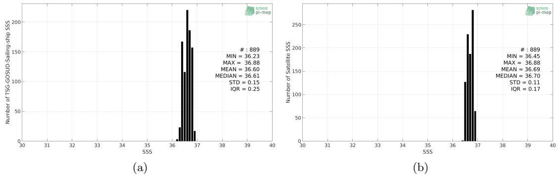
Figure 2: Histograms of SSS from TSG-GOSUD-Sailing-ship (a) and SMAP-L3-RSS-V4-MONTHLY (b) considering all match-up pairs per bins of 0.1 over the SPURS 1 Pi-MEP region and for the full satellite product period.
