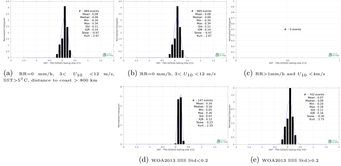
Figure 13: Normalized histogram of \Delta\text{SSS} (SMAP-L3-RSS-V4-MONTHLY - TSG-GOSUD-Sailing-ship) for 5 different subdatasets corresponding to: RR=0 mm/h, 3 < U_{10} < 12 m/s, SST > 5^\circ\text{C} , distance to coast > 800 km (a), RR=0 mm/h, 3 < U_{10} < 12 m/s (b), RR > 1\text{mm/h} and U_{10} < 4\text{m/s} (c), WOA2013 SSS Std <0.2 (d), WOA2013 SSS Std >0.2 (e).
