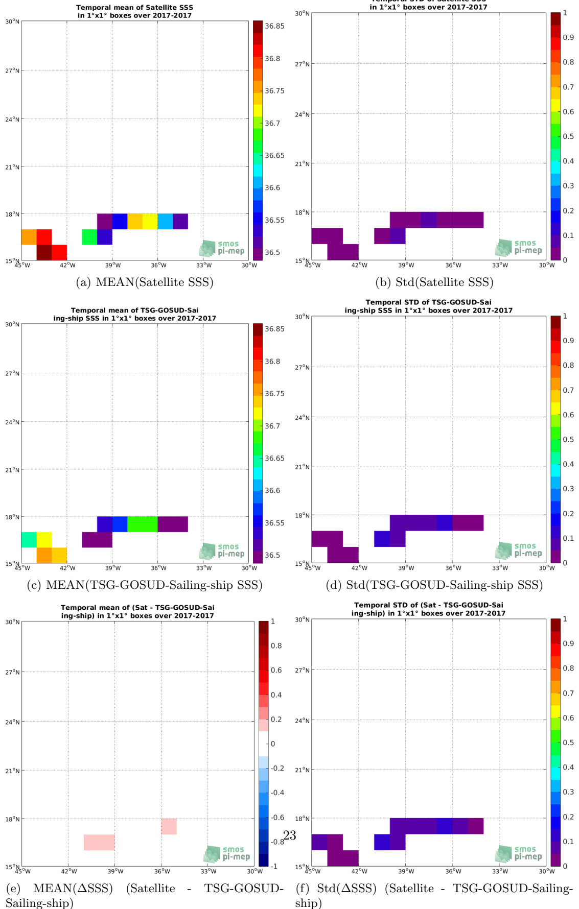
Figure 6: Temporal mean (left) and Std (right) of SSS from SMAP-L3-RSS-V4-MONTHLY (top), TSG-GOSUD-Sailing-ship (middle), and of ΔSSS (Satellite - TSG-GOSUD-Sailing-ship). Only match-up pairs are used to generate these maps.
