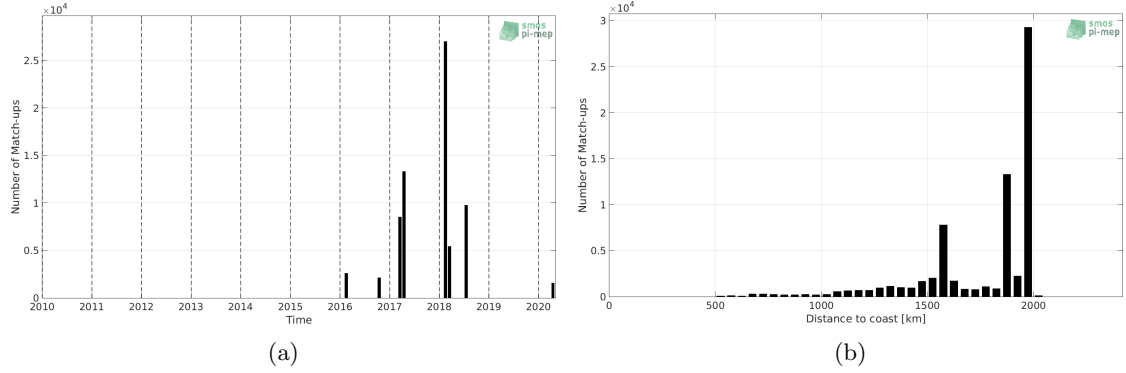
Figure 1: Number of match-ups between TSG (GOSUD-Research-vessel) and SMAP SSS L3 v4 - Monthly (RSS) SSS as a function of time (a) and as function of the distance to coast (b) over the SPURS 1 Pi-MEP region and for the full satellite product period.
