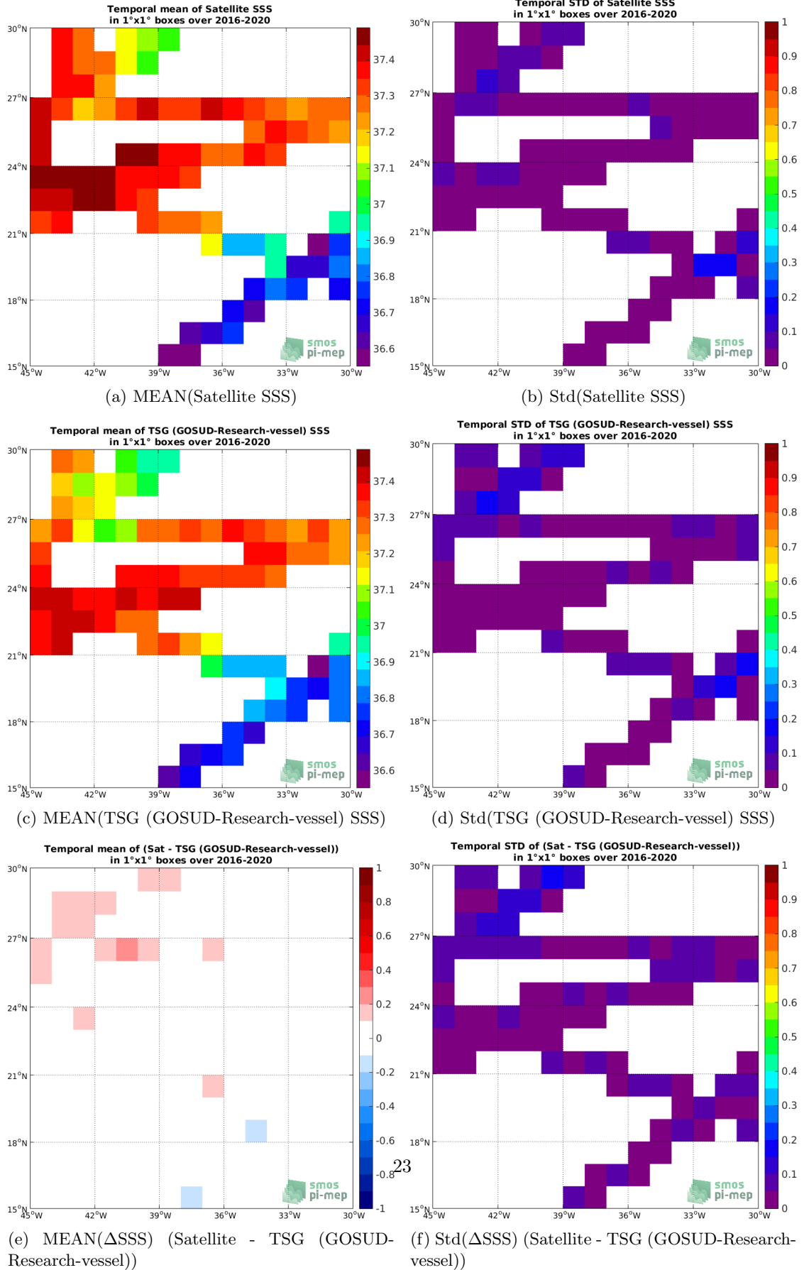
Figure 6: Temporal mean (left) and Std (right) of SSS from SMAP SSS L3 v4 - Monthly (RSS) (top), TSG (GOSUD-Research-vessel) (middle), and of \Delta SSS (Satellite - TSG (GOSUD-Research-vessel)). Only match-up pairs are used to generate these maps.
