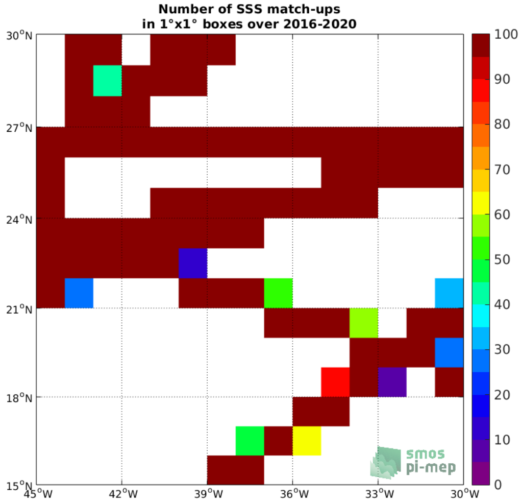
Figure 4: Number of SSS match-ups between TSG (GOSUD-Research-vessel) SSS and the SMAP SSS L3 v4 - Monthly (RSS) SSS product for the SPURS 1 Pi-MEP region over 1°x1° boxes and for the full satellite product period.
