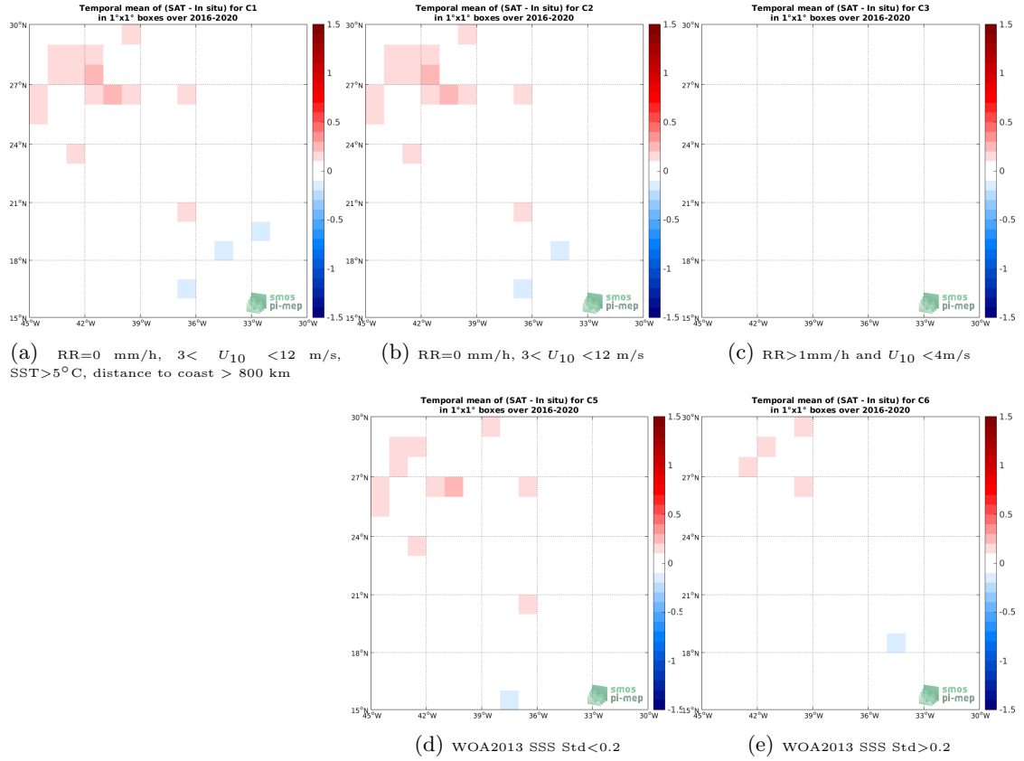
Figure 12: Temporal mean gridded over spatial boxes of size 1^\circ \times 1^\circ of \Delta SSS (SMAP SSS L3 v4 - Monthly (RSS) - TSG (GOSUD-Research-vessel)) for 5 different subdatasets corresponding to: RR=0 mm/h, 3 < U_{10} < 12 m/s, SST > 5^\circ C , distance to coast > 800 km (a), RR=0 mm/h, 3 < U_{10} < 12 m/s (b), RR > 1 mm/h and U_{10} < 4 m/s (c), WOA2013 SSS Std < 0.2 (d), WOA2013 SSS Std > 0.2 (e).
