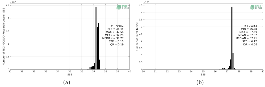
Figure 2: Histograms of SSS from TSG (GOSUD-Research-vessel) (a) and SMAP SSS L3 v4 - Monthly (RSS) (b) considering all match-up pairs per bins of 0.1 over the SPURS 1 Pi-MEP region and for the full satellite product period.
