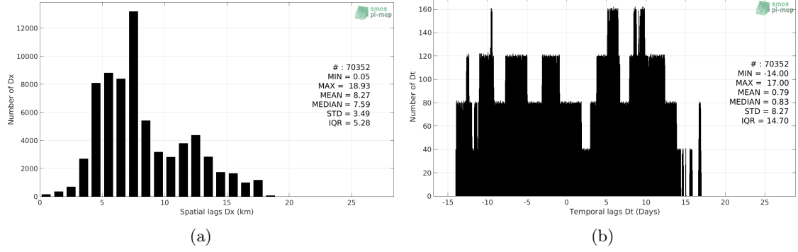
Figure 5: Histograms of the spatial (a) and temporal (b) lags between the location/time of the TSG (GOSUD-Research-vessel) measurement and the date of the corresponding SMAP SSS L3 v4 - Monthly (RSS) SSS pixel.
