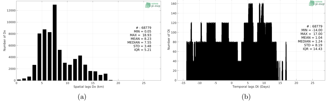
Figure 5: Histograms of the spatial (a) and temporal (b) lags between the time of the TSG (GOSUD-Research-vessel) measurements and the date of the corresponding SMAP SSS L3 v4 - Monthly (RSS) SSS product.
