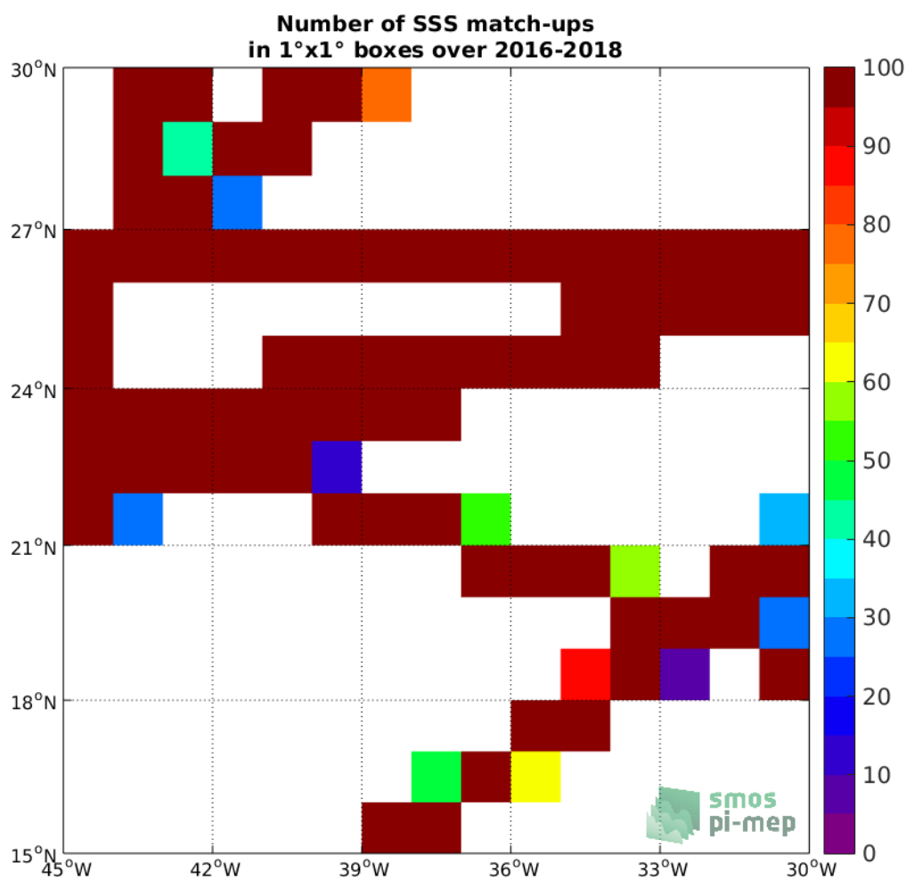
Figure 4: Number of SSS match-ups between TSG-GOSUD-Research-vessel SSS and the SMAP-L3-RSS-V4-MONTHLY SSS product for the SPURS 1 Pi-MEP region over 1°x1° boxes and for the full satellite product period.
