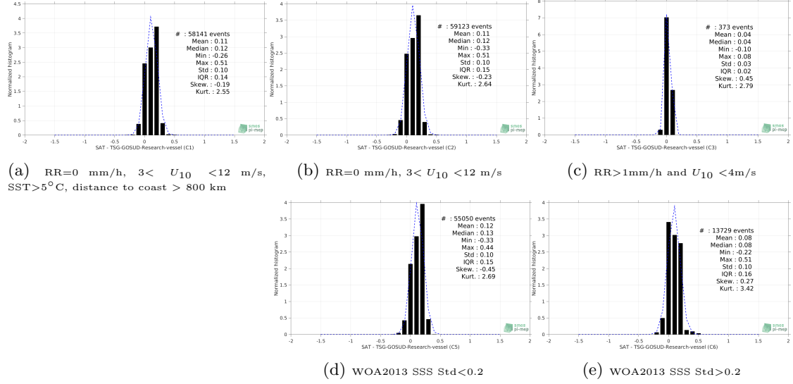
Figure 13: Normalized histogram of \Delta SSS (SMAP-L3-RSS-V4-MONTHLY - TSG-GOSUD-Research-vessel) for 5 different subdatasets corresponding to: RR=0 mm/h, 3 < U_{10} < 12 m/s, SST>5°C, distance to coast > 800 km (a), RR=0 mm/h, 3 < U_{10} < 12 m/s (b), RR>1mm/h and U_{10} < 4 m/s (c), WOA2013 SSS Std<0.2 (d), WOA2013 SSS Std>0.2 (e).
