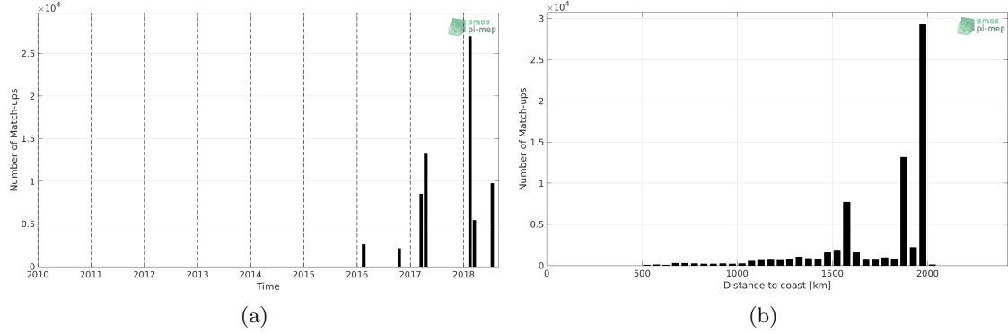
Figure 1: Number of match-ups between TSG-GOSUD-Research-vessel and SMAP-L3-RSS-V4-MONTHLY SSS as a function of time (a) and as function of the distance to coast (b) over the SPURS 1 Pi-MEP region and for the full satellite product period.
