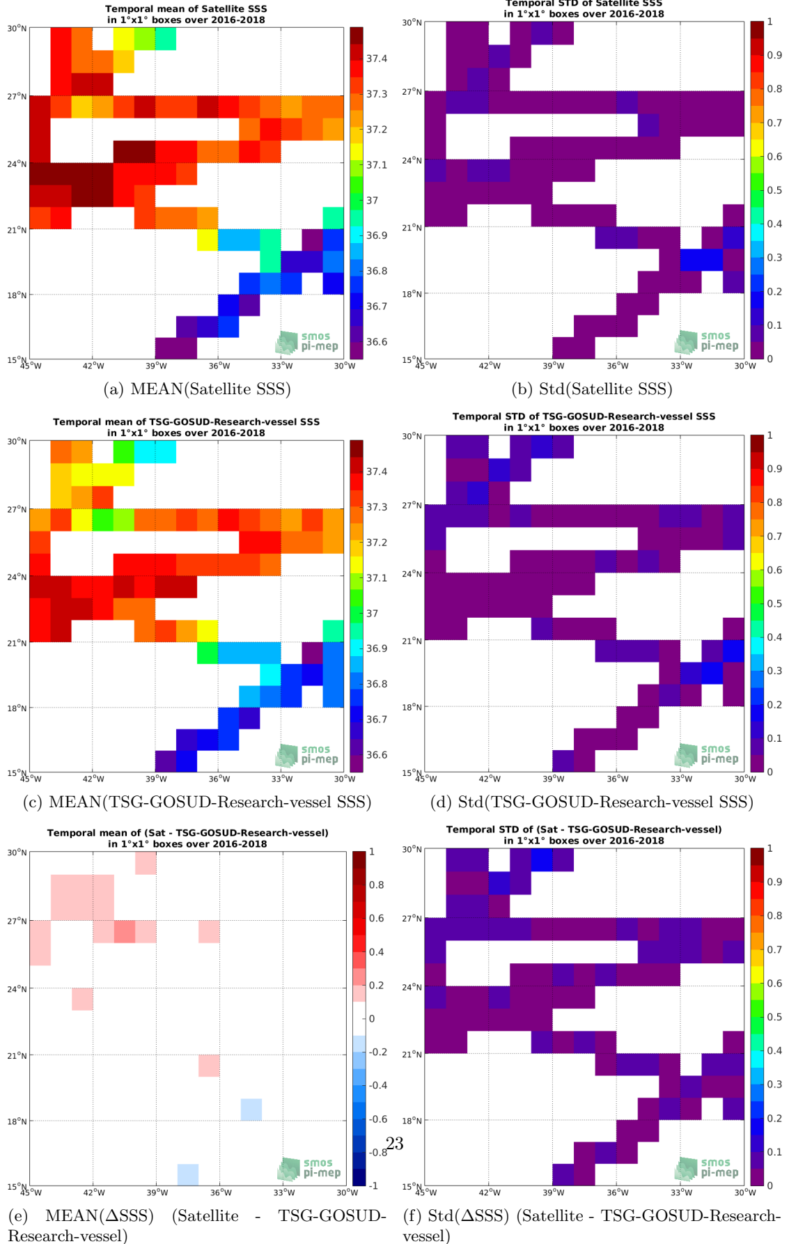
Figure 6: Temporal mean (left) and Std (right) of SSS from SMAP-L3-RSS-V4-MONTHLY (top), TSG-GOSUD-Research-vessel (middle), and of \Delta SSS (Satellite - TSG-GOSUD-Research-vessel). Only match-up pairs are used to generate these maps.
