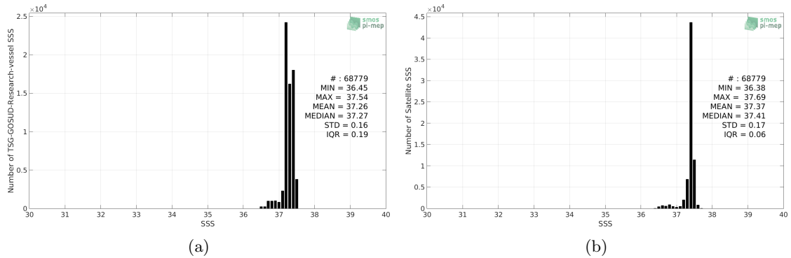
Figure 2: Histograms of SSS from TSG-GOSUD-Research-vessel (a) and SMAP-L3-RSS-V4-MONTHLY (b) considering all match-up pairs per bins of 0.1 over the SPURS 1 Pi-MEP region and for the full satellite product period.
