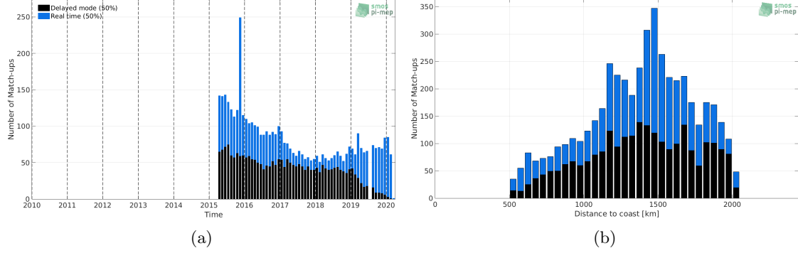
Figure 1: Number of match-ups between Argo and SMAP-L3-RSS-V4-MONTHLY SSS as a function of time (a) and as function of the distance to coast (b) over the SPURS 1 Pi-MEP region and for the full satellite product period.
