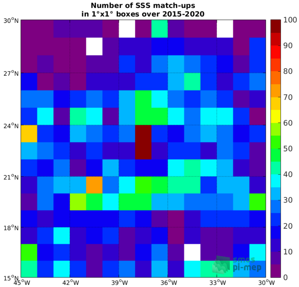
Figure 4: Number of SSS match-ups between Argo SSS and the SMAP-L3-RSS-V4-MONTHLY SSS product for the SPURS 1 Pi-MEP region over 1°x1° boxes and for the full satellite product period.
