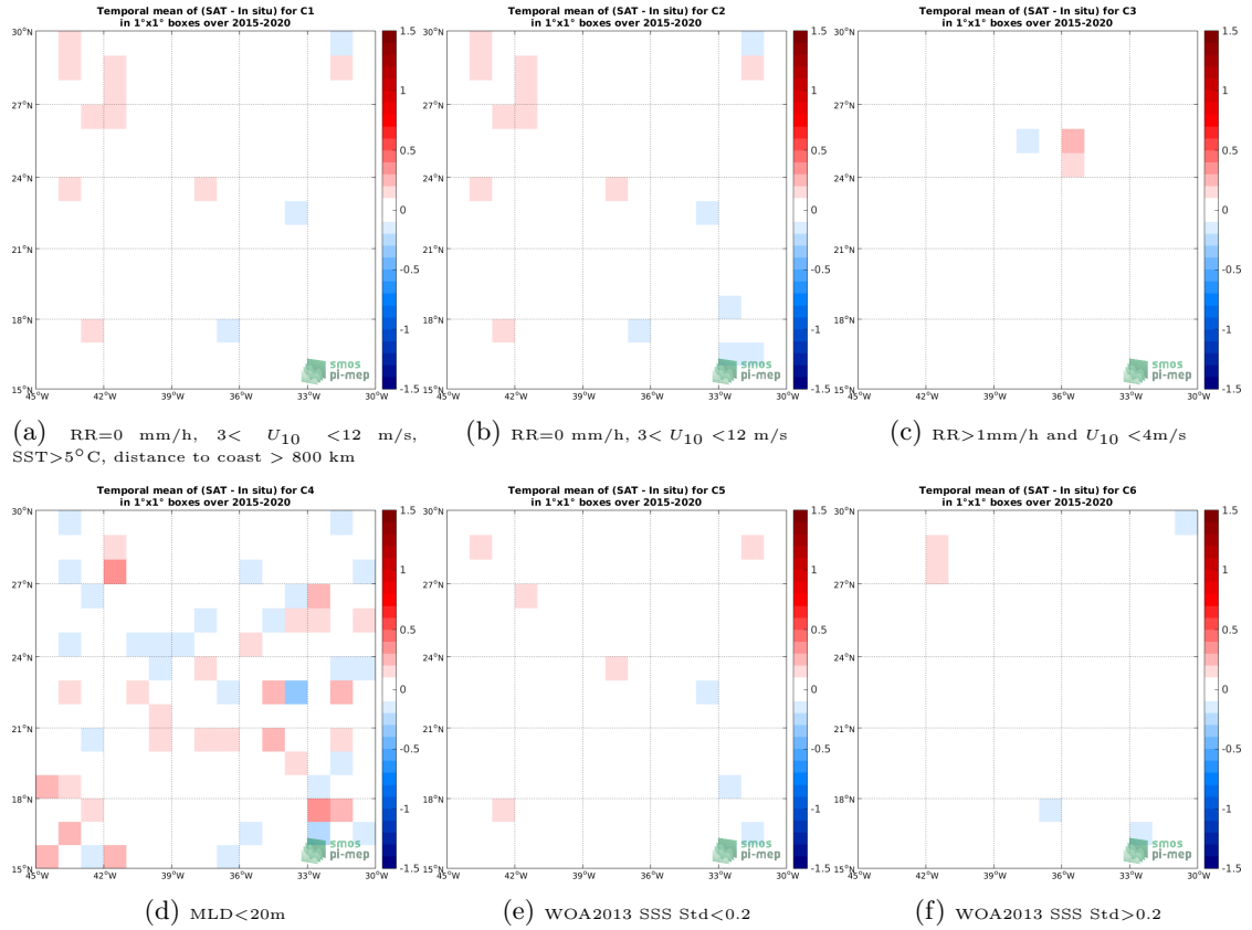
Figure 12: Temporal mean gridded over spatial boxes of size 1^\circ \times 1^\circ of \Delta SSS (SMAP-L3-RSS-V4-MONTHLY - Argo) for 6 different subdatasets corresponding to:RR=0 mm/h, 3 < U_{10} < 12 m/s, SST >5^\circ\text{C} , distance to coast > 800 km (a), RR=0 mm/h, 3 < U_{10} < 12 m/s (b), RR >1 mm/h and U_{10} < 4 m/s (c),MLD <20 m (d),WOA2013 SSS Std <0.2 (e),WOA2013 SSS Std >0.2 (f).
