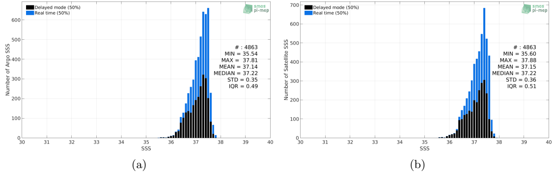
Figure 2: Histograms of SSS from Argo (a) and SMAP-L3-RSS-V4-MONTHLY (b) considering all match-up pairs per bins of 0.1 over the SPURS 1 Pi-MEP region and for the full satellite product period.
