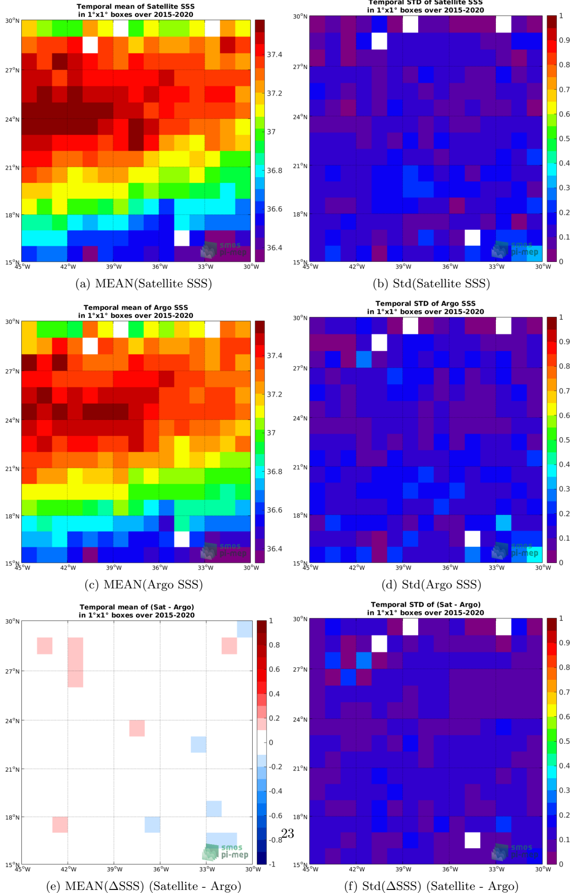
Figure 6: Temporal mean (left) and Std (right) of SSS from SMAP-L3-RSS-V4-MONTHLY (top), Argo (middle), and of \Delta SSS (Satellite - Argo). Only match-up pairs are used to generate these maps.
