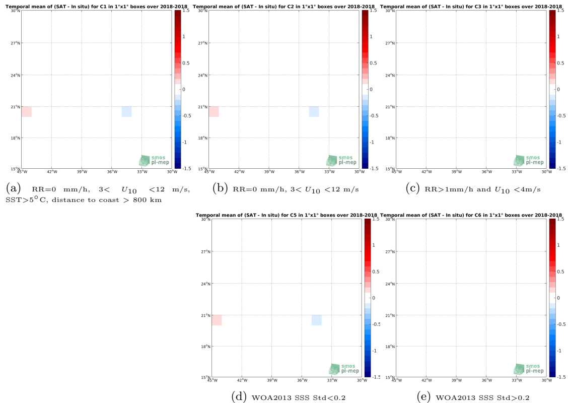
Figure 12: Temporal mean gridded over spatial boxes of size 1^\circ \times 1^\circ of \Delta SSS (SMAP-L3-RSS-V3-8DAY-RUNNING-70KM - TSG-SAMOS) for 5 different subdatasets corresponding to:RR=0 mm/h, 3 < U_{10} < 12 m/s, SST >5^\circ C, distance to coast > 800 km (a), RR=0 mm/h, 3 < U_{10} < 12 m/s (b), RR >1 mm/h and U_{10} < 4 m/s (c), WOA2013 SSS Std <0.2 (d), WOA2013 SSS Std >0.2 (e).
