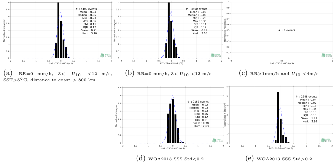
Figure 13: Normalized histogram of \Delta SSS (SMAP-L3-RSS-V3-8DAY-RUNNING-70KM - TSG-SAMOS) for 5 different subdatasets corresponding to: RR=0 mm/h, 3 < U_{10} < 12 m/s, SST > 5°C, distance to coast > 800 km (a), RR=0 mm/h, 3 < U_{10} < 12 m/s (b), RR > 1mm/h and U_{10} < 4 m/s (c), WOA2013 SSS Std < 0.2 (d), WOA2013 SSS Std > 0.2 (e).
