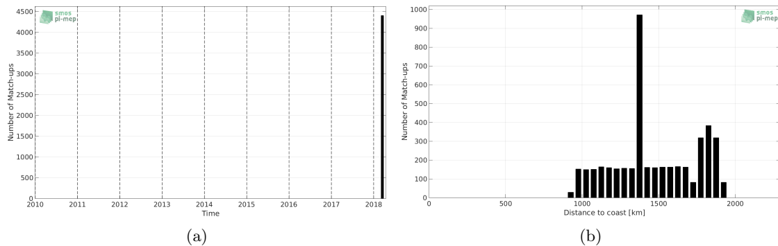
Figure 1: Number of match-ups between TSG-SAMOS and SMAP-L3-RSS-V3-8DAY-RUNNING-70KM SSS as a function of time (a) and as function of the distance to coast (b) over the SPURS 1 Pi-MEP region and for the full satellite product period.
