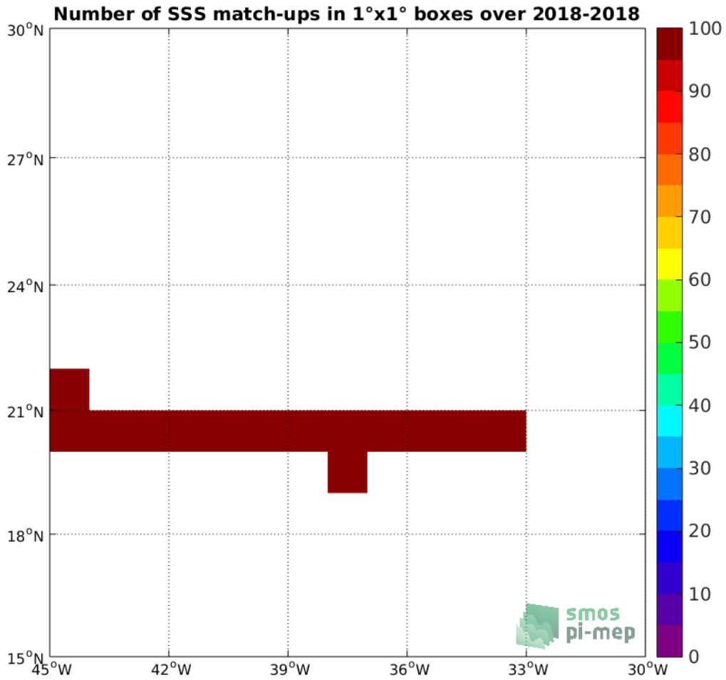
Figure 4: Number of SSS match-ups between TSG-SAMOS SSS and the SMAP-L3-RSS-V3-8DAY-RUNNING-70KM SSS product for the SPURS 1 Pi-MEP region over 1°x1° boxes and for the full satellite product period.
