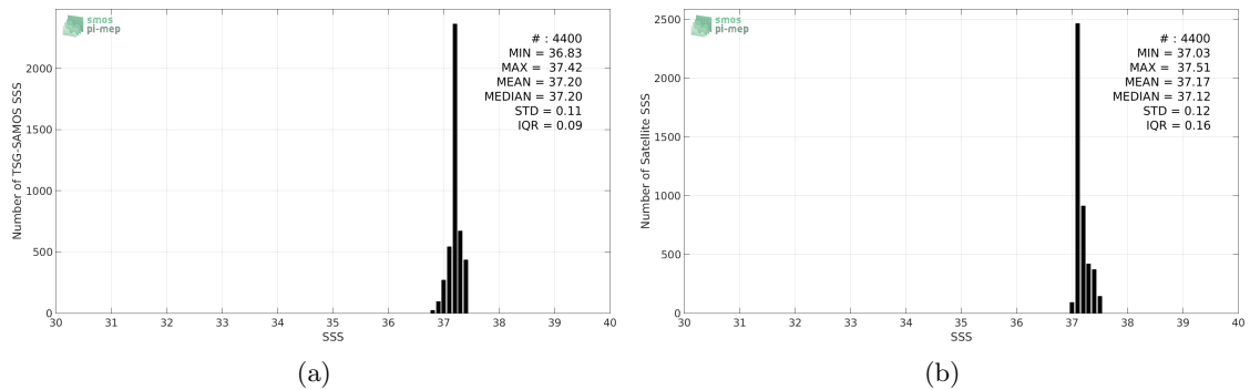
Figure 2: Histograms of SSS from TSG-SAMOS (a) and SMAP-L3-RSS-V3-8DAY-RUNNING-70KM (b) considering all match-up pairs per bins of 0.1 over the SPURS 1 Pi-MEP region and for the full satellite product period.
