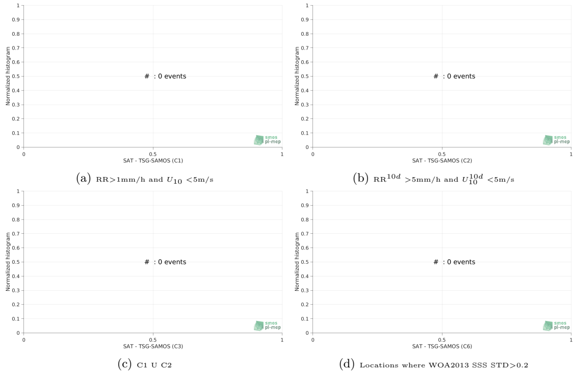
Figure 13: Normalized histogram of \Delta\text{SSS} (SMAP-L3-RSS-V3-8DAY-RUNNING-70KM - TSG-SAMOS) for 6 different subdatasets corresponding to: RR > 1\text{mm/h} and U_{10} < 5\text{m/s} (a), RR^{10d} > 5\text{mm/h} and U_{10}^{10d} < 5\text{m/s} (b), C1 \cup C2 (c), Locations where WOA2013 SSS STD > 0.2 (d).
