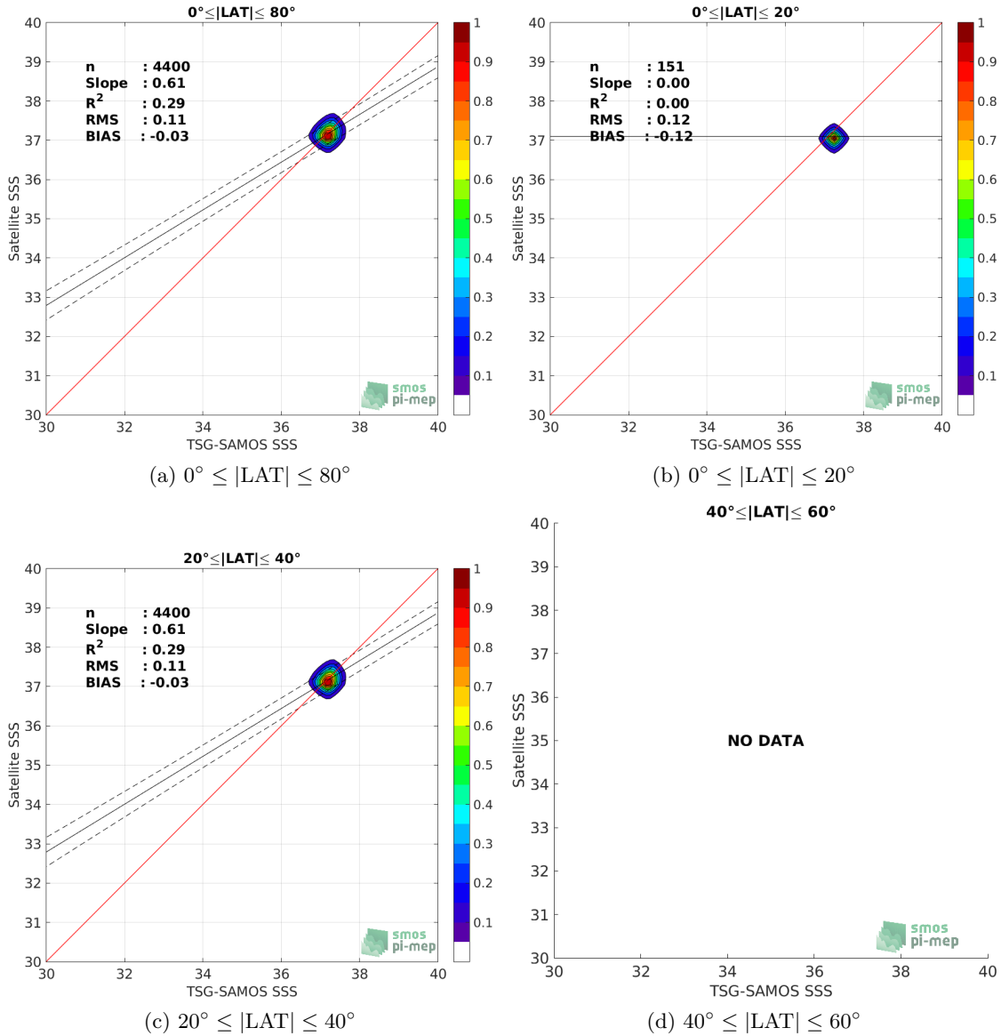
Figure 9: Contour maps of the concentration of SMAP-L3-RSS-V3-8DAY-RUNNING-70KM SSS (y-axis) versus TSG-SAMOS SSS (x-axis) at match-up pairs for different latitude bands. For each plot, the red line shows x=y . The black thin and dashed lines indicate a linear fit through the data cloud and the \pm 95\% confidence levels, respectively. The number match-up pairs n , the slope and R^2 coefficient of the linear fit, the root mean square (RMS) and the mean bias between satellite and in situ data are indicated for each latitude band in each plots.
