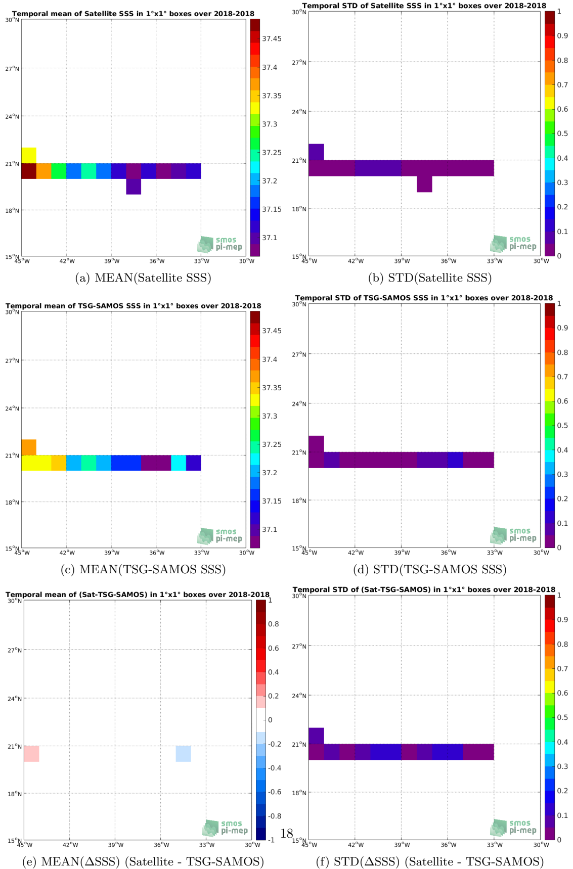
Figure 6: Temporal mean (left) and STD (right) of SSS from SMAP-L3-RSS-V3-8DAY-RUNNING-70KM (top), TSG-SAMOS (middle), and of \Delta SSS (Satellite - TSG-SAMOS). Only match-up pairs are used to generate these maps.
