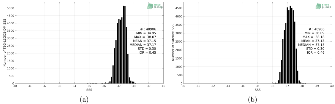
Figure 2: Histograms of SSS from TSG-LEGOS-DM (a) and SMAP-L3-RSS-V3-8DAY-RUNNING-70KM (b) considering all match-up pairs per bins of 0.1 over the SPURS 1 Pi-MEP region and for the full satellite product period.
