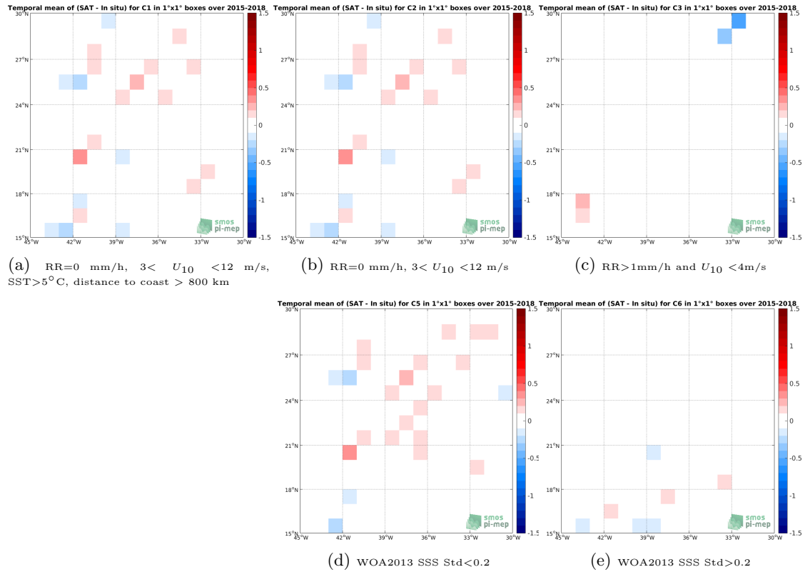
Figure 12: Temporal mean gridded over spatial boxes of size 1^\circ \times 1^\circ of \Delta SSS (SMAP-L3-RSS-V3-8DAY-RUNNING-70KM - TSG-LEGOS-DM) for 5 different subdatasets corresponding to:RR=0 mm/h, 3 < U_{10} < 12 m/s, SST >5^\circ C, distance to coast > 800 km (a), RR=0 mm/h, 3 < U_{10} < 12 m/s (b), RR >1 mm/h and U_{10} < 4 m/s (c), WOA2013 SSS Std <0.2 (d), WOA2013 SSS Std >0.2 (e).
