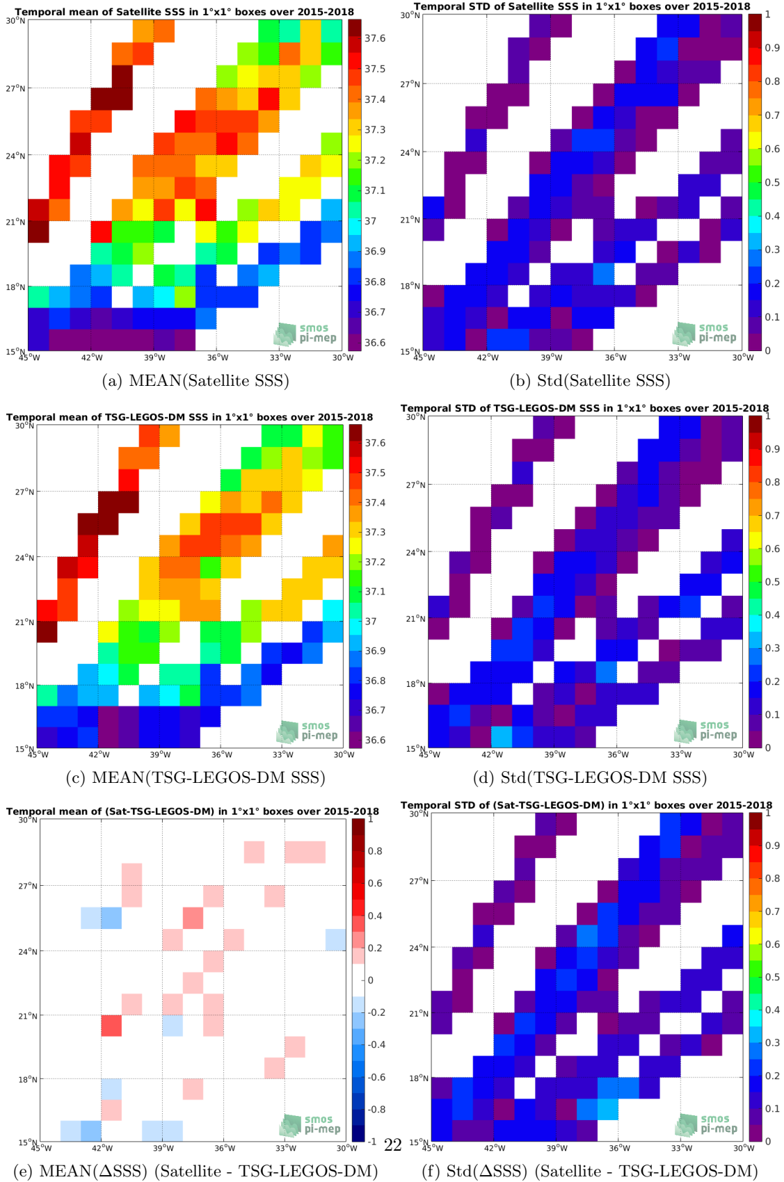
Figure 6: Temporal mean (left) and Std (right) of SSS from SMAP-L3-RSS-V3-8DAY-RUNNING-70KM (top), TSG-LEGOS-DM (middle), and of \Delta SSS (Satellite - TSG-LEGOS-DM). Only match-up pairs are used to generate these maps.
