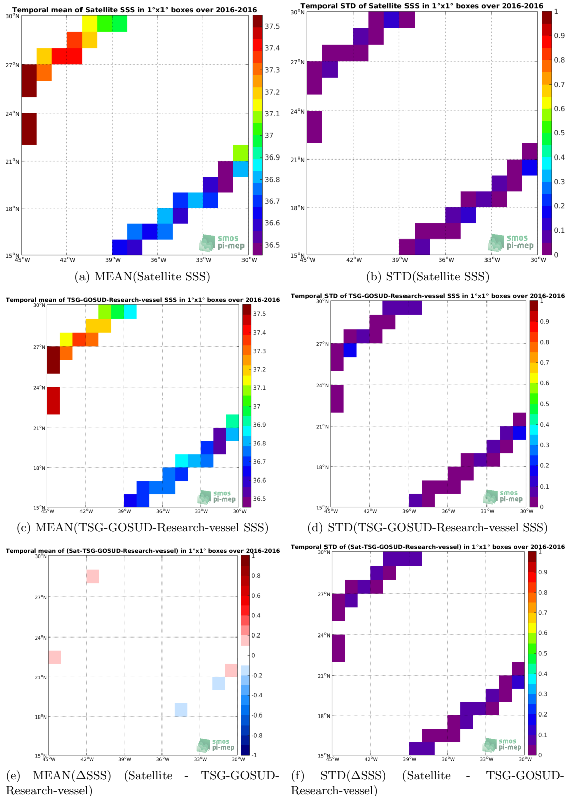
Figure 6: Temporal mean (left) and STD (right) of SSS from SMAP-L3-RSS-V3-8DAY-RUNNING-70KM (top), TSG-GOSUD-Research-vessel (middle), and of \Delta SSS (Satellite - TSG-GOSUD-Research-vessel). Only match-up pairs are used to generate these maps.
