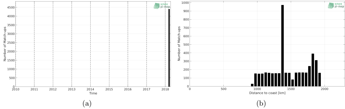
Figure 1: Number of match-ups between TSG-SAMOS and SMAP-L3-RSS-V3-8DAY-RUNNING-40KM SSS as a function of time (a) and as function of the distance to coast (b) over the SPURS 1 Pi-MEP region and for the full satellite product period.
