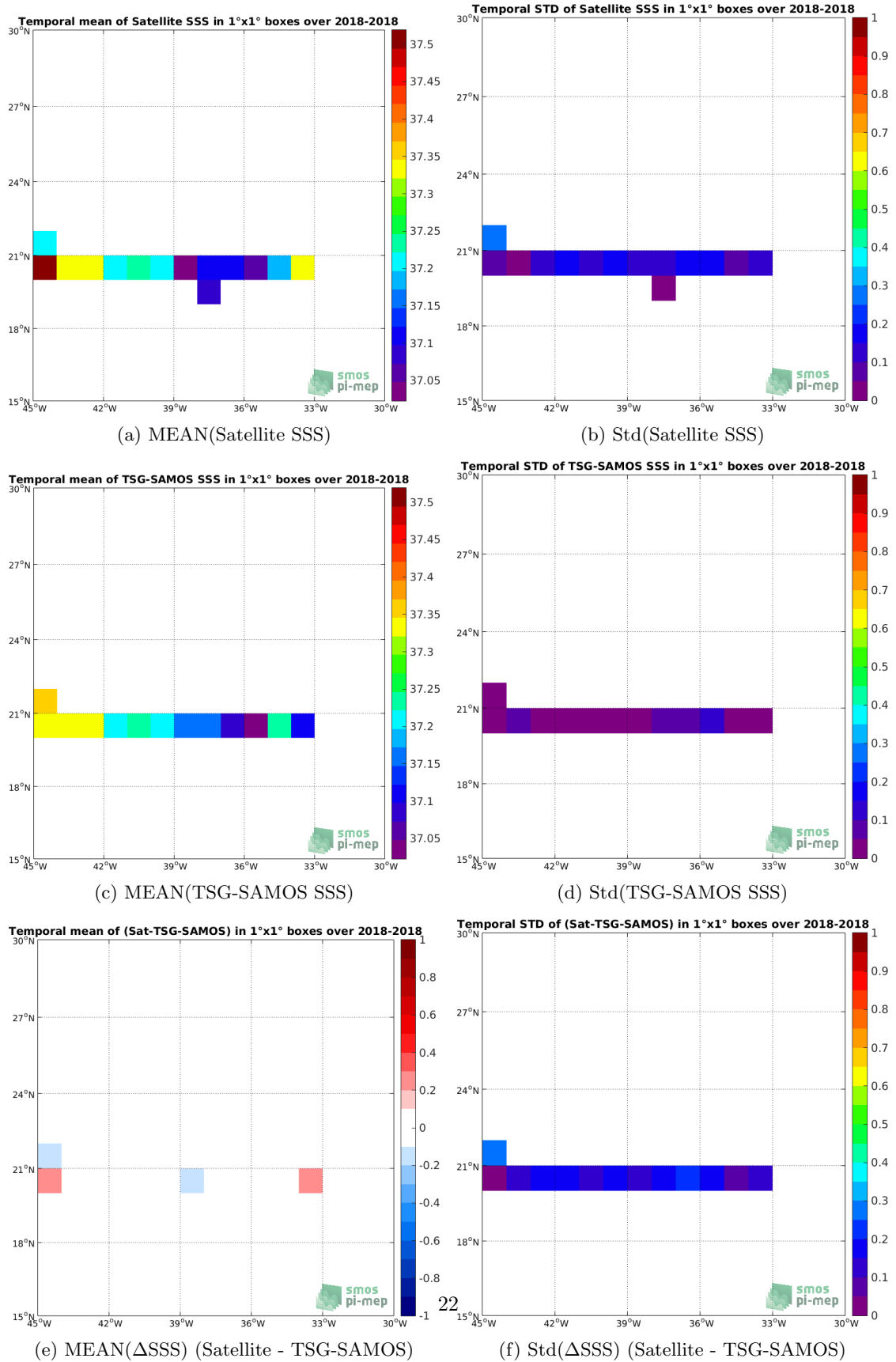
Figure 6: Temporal mean (left) and Std (right) of SSS from SMAP-L3-RSS-V3-8DAY-RUNNING-40KM (top), TSG-SAMOS (middle), and of \Delta SSS (Satellite - TSG-SAMOS). Only match-up pairs are used to generate these maps.
