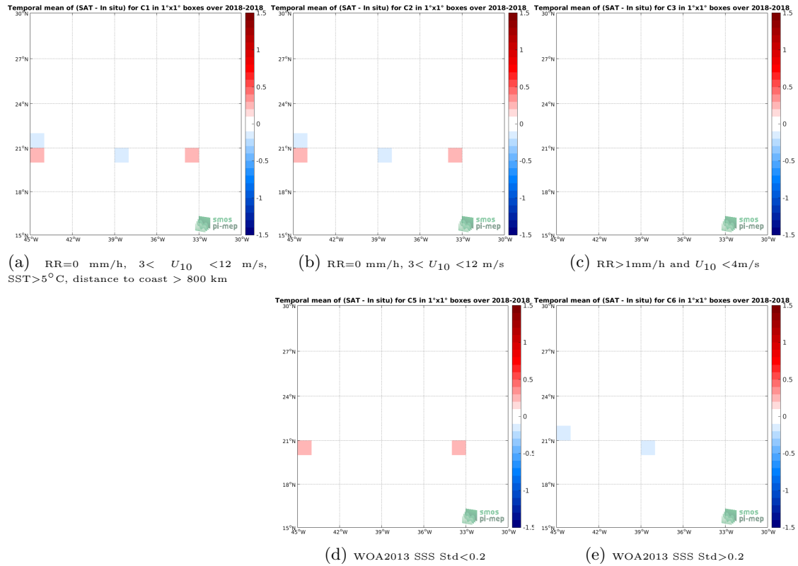
Figure 12: Temporal mean gridded over spatial boxes of size 1^\circ \times 1^\circ of \Delta SSS (SMAP-L3-RSS-V3-8DAY-RUNNING-40KM - TSG-SAMOS) for 5 different subdatasets corresponding to:RR=0 mm/h, 3 < U_{10} < 12 m/s, SST >5^\circ C, distance to coast > 800 km (a), RR=0 mm/h, 3 < U_{10} < 12 m/s (b), RR >1 mm/h and U_{10} < 4 m/s (c), WOA2013 SSS Std <0.2 (d), WOA2013 SSS Std >0.2 (e).
