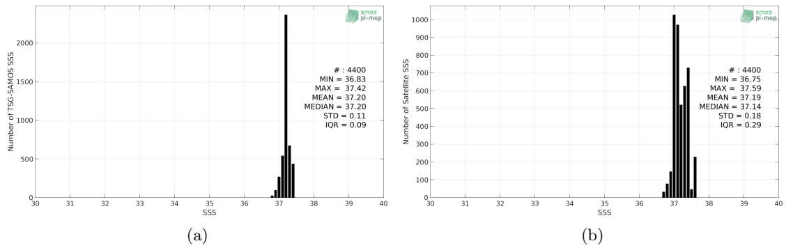
Figure 2: Histograms of SSS from TSG-SAMOS (a) and SMAP-L3-RSS-V3-8DAY-RUNNING-40KM (b) considering all match-up pairs per bins of 0.1 over the SPURS 1 Pi-MEP region and for the full satellite product period.
