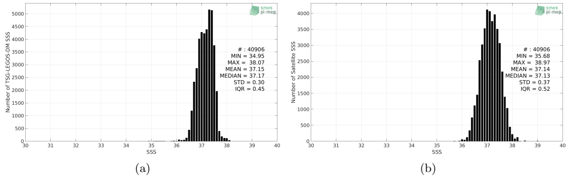
Figure 2: Histograms of SSS from TSG-LEGOS-DM (a) and SMAP-L3-RSS-V3-8DAY-RUNNING-40KM (b) considering all match-up pairs per bins of 0.1 over the SPURS 1 Pi-MEP region and for the full satellite product period.
