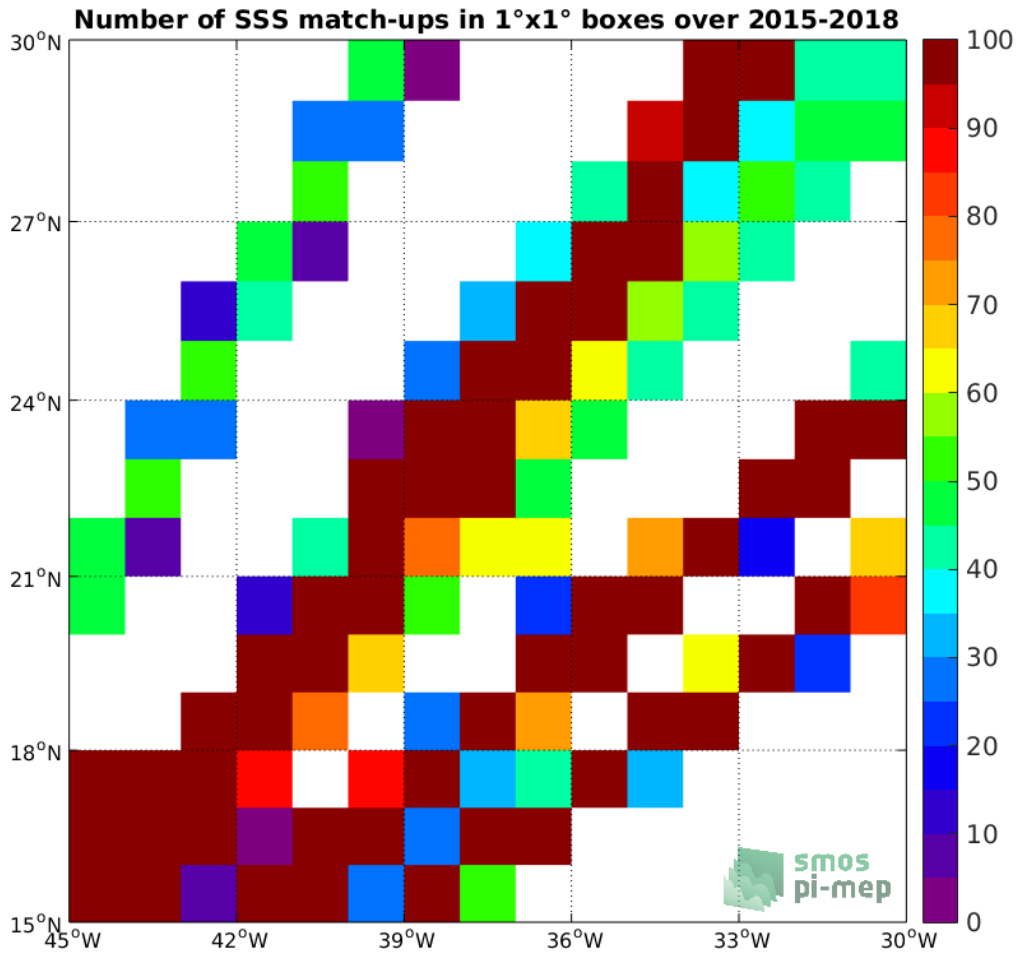
Figure 4: Number of SSS match-ups between TSG-LEGOS-DM SSS and the SMAP-L3-RSS-V3-8DAY-RUNNING-40KM SSS product for the SPURS 1 Pi-MEP region over 1°x1° boxes and for the full satellite product period.
