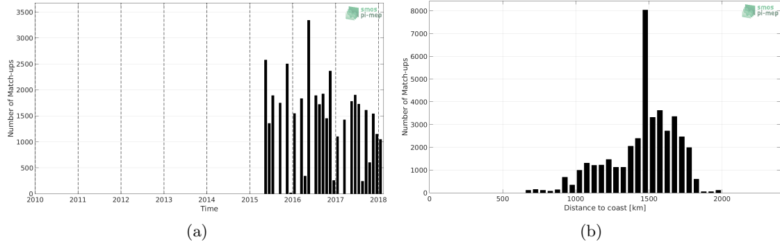
Figure 1: Number of match-ups between TSG-LEGOS-DM and SMAP-L3-RSS-V3-8DAY-RUNNING-40KM SSS as a function of time (a) and as function of the distance to coast (b) over the SPURS 1 Pi-MEP region and for the full satellite product period.
