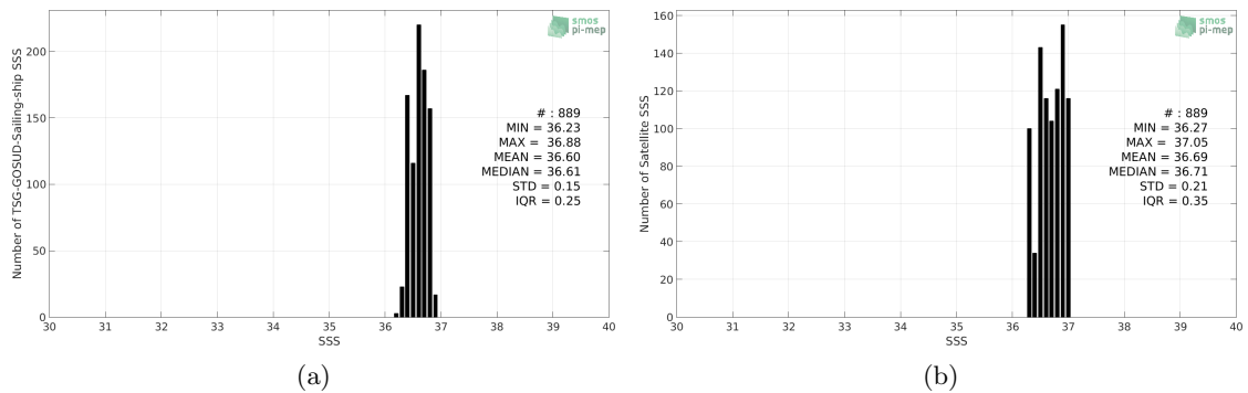
Figure 2: Histograms of SSS from TSG-GOSUD-Sailing-ship (a) and SMAP-L3-RSS-V3-8DAY-RUNNING-40KM (b) considering all match-up pairs per bins of 0.1 over the SPURS 1 Pi-MEP region and for the full satellite product period.
