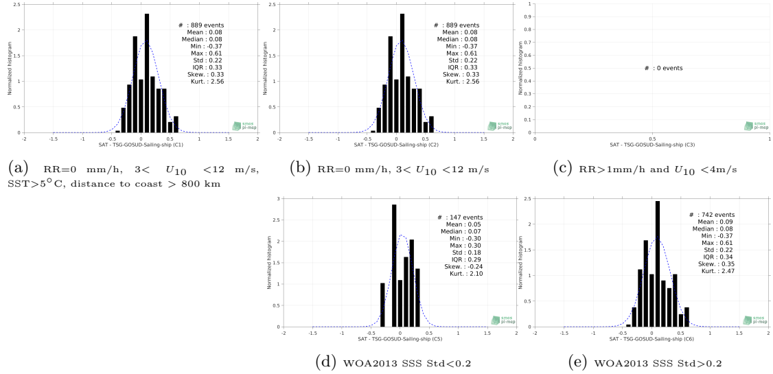
Figure 13: Normalized histogram of \Delta SSS (SMAP-L3-RSS-V3-8DAY-RUNNING-40KM - TSG-GOSUD-Sailing-ship) for 5 different subdatasets corresponding to: RR=0 mm/h, 3 < U_{10} < 12 m/s, SST>5°C, distance to coast > 800 km (a), RR=0 mm/h, 3 < U_{10} < 12 m/s (b), RR>1mm/h and U_{10} < 4 m/s (c), WOA2013 SSS Std<0.2 (d), WOA2013 SSS Std>0.2 (e).
