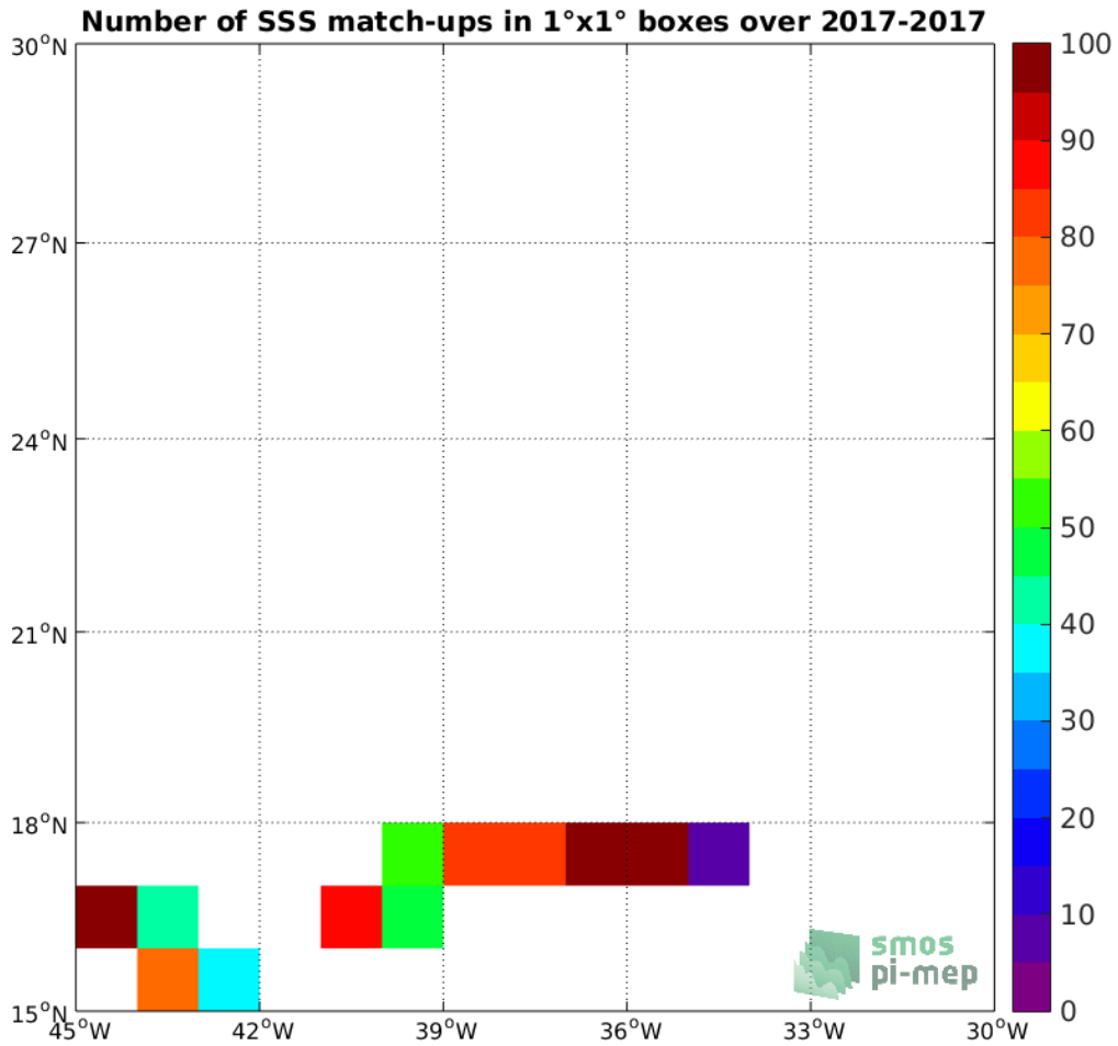
Figure 4: Number of SSS match-ups between TSG-GOSUD-Sailing-ship SSS and the SMAP-L3-RSS-V3-8DAY-RUNNING-40KM SSS product for the SPURS 1 Pi-MEP region over 1°x1° boxes and for the full satellite product period.
