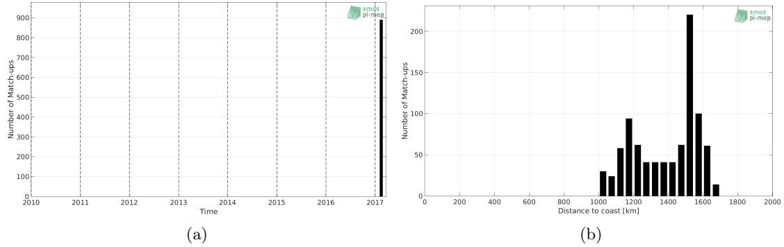
Figure 1: Number of match-ups between TSG-GOSUD-Sailing-ship and SMAP-L3-RSS-V3-8DAY-RUNNING-40KM SSS as a function of time (a) and as function of the distance to coast (b) over the SPURS 1 Pi-MEP region and for the full satellite product period.
