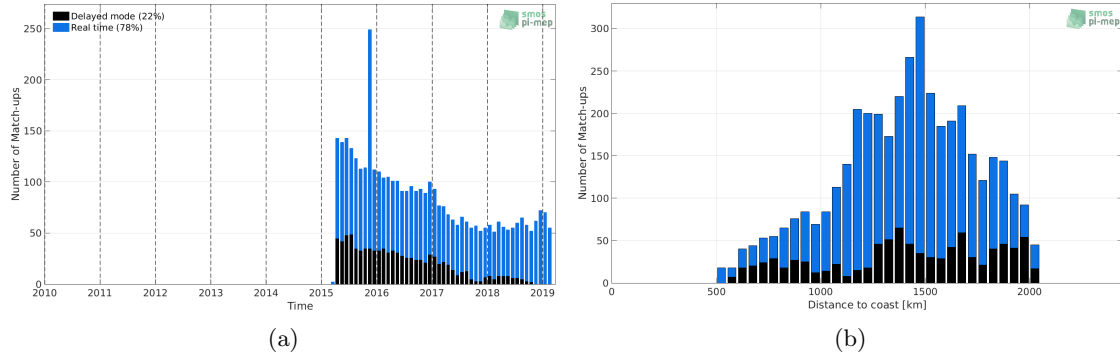
Figure 1: Number of match-ups between Argo and SMAP-L3-RSS-V3-8DAY-RUNNING-40KM SSS as a function of time (a) and as function of the distance to coast (b) over the SPURS 1 Pi-MEP region and for the full satellite product period.
