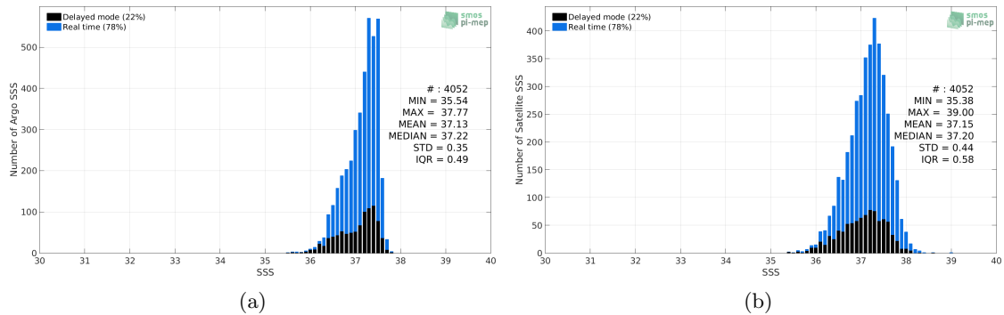
Figure 2: Histograms of SSS from Argo (a) and SMAP-L3-RSS-V3-8DAY-RUNNING-40KM (b) considering all match-up pairs per bins of 0.1 over the SPURS 1 Pi-MEP region and for the full satellite product period.
