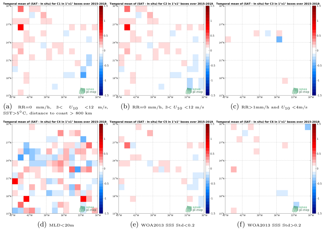
Figure 12: Temporal mean gridded over spatial boxes of size 1^\circ \times 1^\circ of \Delta SSS (SMAP-L3-RSS-V3-8DAY-RUNNING-40KM - Argo) for 6 different subdatasets corresponding to: RR=0 mm/h, 3 < U_{10} < 12 m/s, SST > 5^\circ\text{C} , distance to coast > 800 km (a), RR=0 mm/h, 3 < U_{10} < 12 m/s (b), RR > 1 mm/h and U_{10} < 4 m/s (c), MLD < 20 m (d), WOA2013 SSS Std < 0.2 (e), WOA2013 SSS Std > 0.2 (f).
