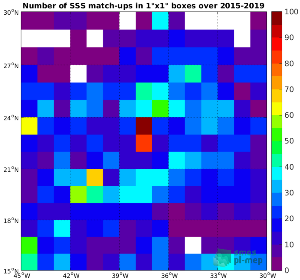
Figure 4: Number of SSS match-ups between Argo SSS and the SMAP-L3-RSS-V3-8DAY-RUNNING-40KM SSS product for the SPURS 1 Pi-MEP region over 1°x1° boxes and for the full satellite product period.
