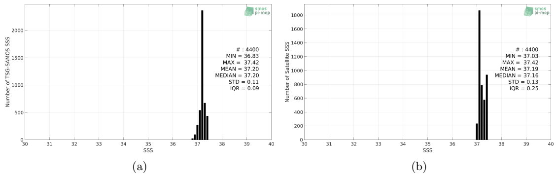
Figure 2: Histograms of SSS from TSG-SAMOS (a) and SMAP-L3-RSS-V3-MONTHLY-70KM (b) considering all match-up pairs per bins of 0.1 over the SPURS 1 Pi-MEP region and for the full satellite product period.
