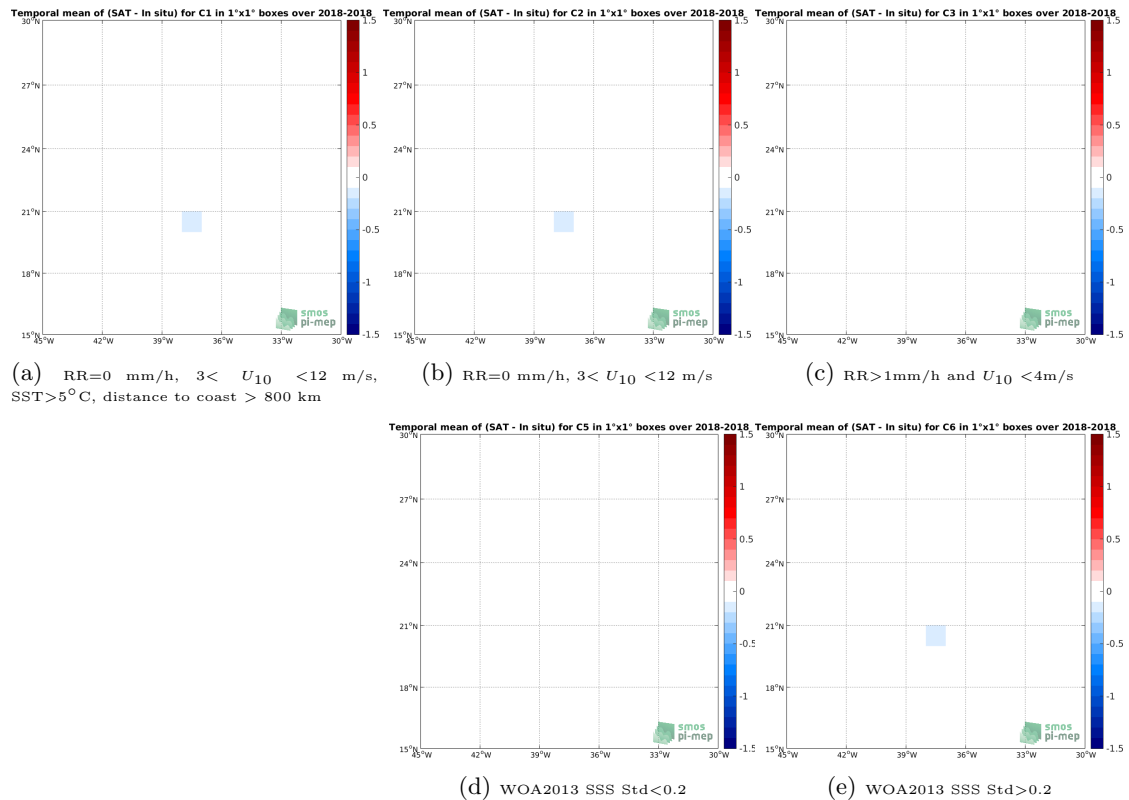
Figure 12: Temporal mean gridded over spatial boxes of size 1^\circ \times 1^\circ of \Delta SSS (SMAP-L3-RSS-V3-MONTHLY-70KM - TSG-SAMOS) for 5 different subdatasets corresponding to: RR=0 mm/h, 3 < U_{10} < 12 m/s, SST > 5^\circ\text{C} , distance to coast > 800 km (a), RR=0 mm/h, 3 < U_{10} < 12 m/s (b), RR > 1\text{mm/h} and U_{10} < 4\text{m/s} (c), WOA2013 SSS Std < 0.2 (d), WOA2013 SSS Std > 0.2 (e).
