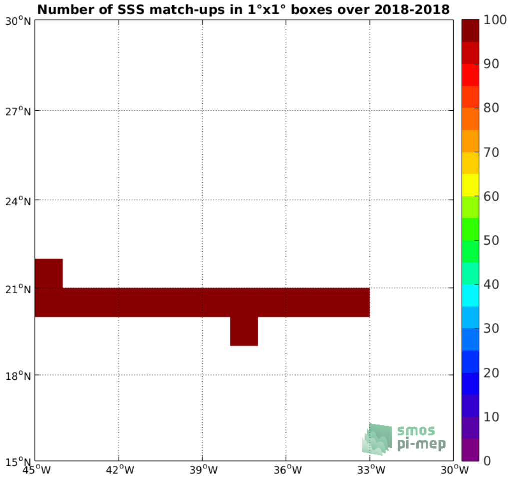
Figure 4: Number of SSS match-ups between TSG-SAMOS SSS and the SMAP-L3-RSS-V3-MONTHLY-70KM SSS product for the SPURS 1 Pi-MEP region over 1°x1° boxes and for the full satellite product period.
