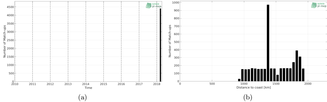
Figure 1: Number of match-ups between TSG-SAMOS and SMAP-L3-RSS-V3-MONTHLY-70KM SSS as a function of time (a) and as function of the distance to coast (b) over the SPURS 1 Pi-MEP region and for the full satellite product period.
