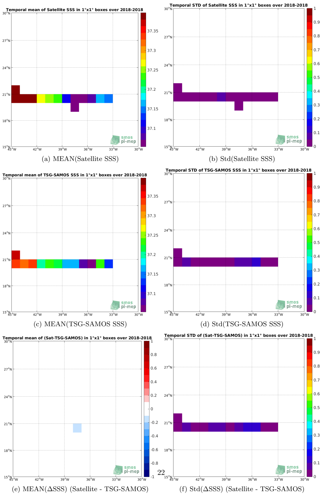
Figure 6: Temporal mean (left) and Std (right) of SSS from SMAP-L3-RSS-V3-MONTHLY-70KM (top), TSG-SAMOS (middle), and of \Delta SSS (Satellite - TSG-SAMOS). Only match-up pairs are used to generate these maps.
