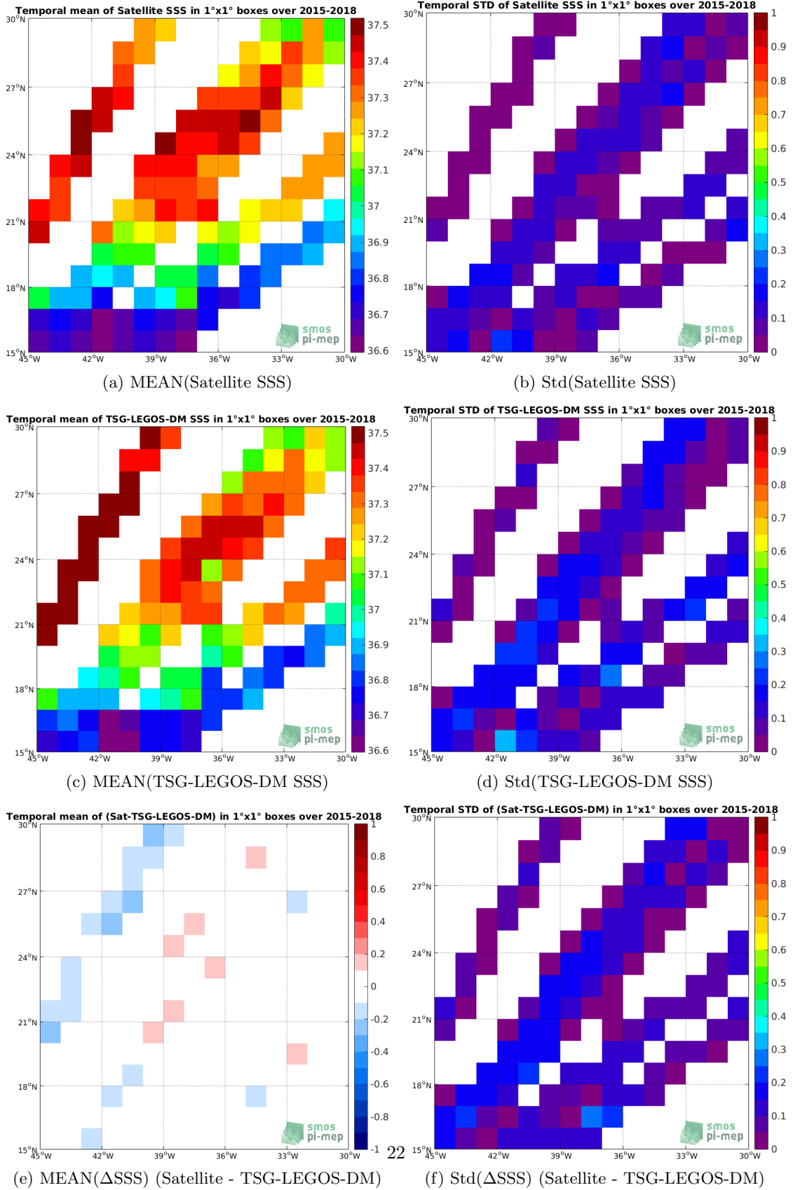
Figure 6: Temporal mean (left) and Std (right) of SSS from SMAP-L3-RSS-V3-MONTHLY-70KM (top), TSG-LEGOS-DM (middle), and of \Delta SSS (Satellite - TSG-LEGOS-DM). Only match-up pairs are used to generate these maps.
