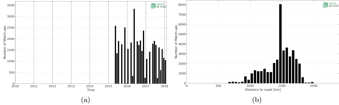
Figure 1: Number of match-ups between TSG-LEGOS-DM and SMAP-L3-RSS-V3-MONTHLY-70KM SSS as a function of time (a) and as function of the distance to coast (b) over the SPURS 1 Pi-MEP region and for the full satellite product period.
