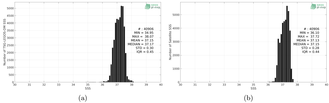
Figure 2: Histograms of SSS from TSG-LEGOS-DM (a) and SMAP-L3-RSS-V3-MONTHLY-70KM (b) considering all match-up pairs per bins of 0.1 over the SPURS 1 Pi-MEP region and for the full satellite product period.
