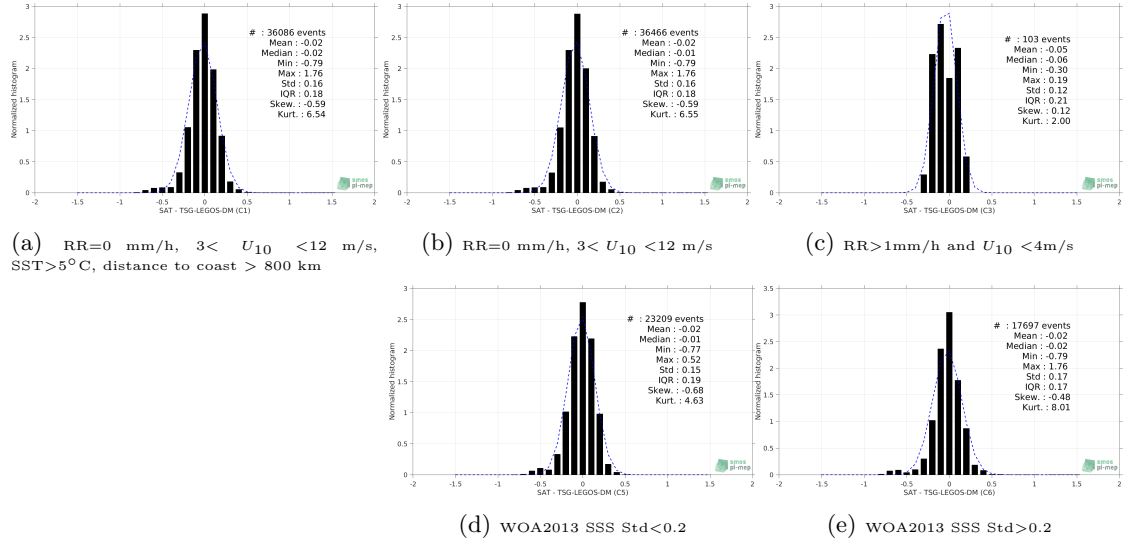
Figure 13: Normalized histogram of \Delta SSS (SMAP-L3-RSS-V3-MONTHLY-70KM - TSG-LEGOS-DM) for 5 different subdatasets corresponding to: RR=0 mm/h, 3 < U_{10} < 12 m/s, SST>5°C, distance to coast > 800 km (a), RR=0 mm/h, 3 < U_{10} < 12 m/s (b), RR>1mm/h and U_{10} < 4 m/s (c), WOA2013 SSS Std<0.2 (d), WOA2013 SSS Std>0.2 (e).
