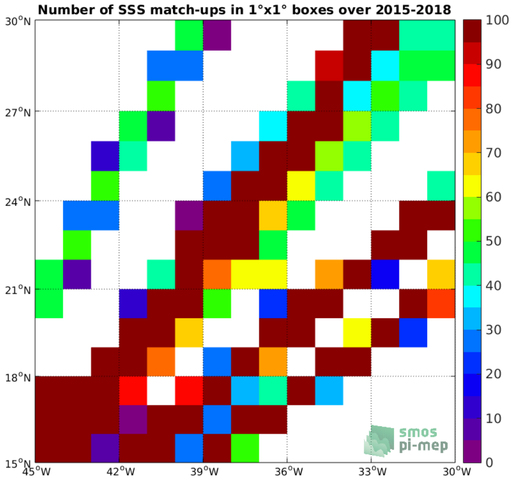
Figure 4: Number of SSS match-ups between TSG-LEGOS-DM SSS and the SMAP-L3-RSS-V3-MONTHLY-70KM SSS product for the SPURS 1 Pi-MEP region over 1°x1° boxes and for the full satellite product period.
