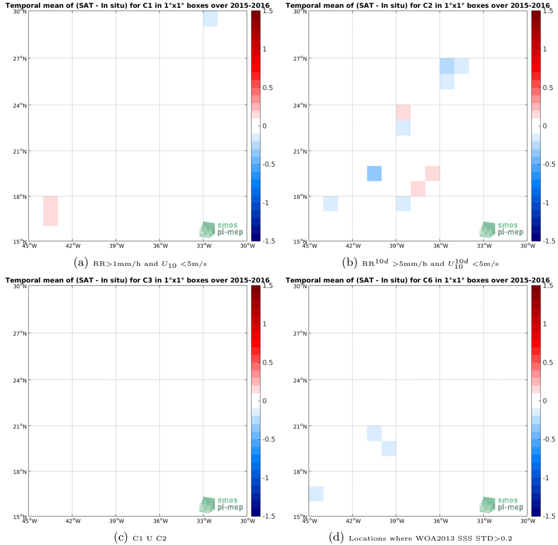
Figure 12: Temporal mean gridded over spatial boxes of size 1^\circ \times 1^\circ of \Delta SSS (SMAP-L3-RSS-V3-MONTHLY-70KM - TSG-LEGOS-DM) for 4 different subdatasets corresponding to: RR > 1\text{mm/h} and U_{10} < 5\text{m/s} (a), RR^{10d} > 5\text{mm/h} and U_{10}^{10d} < 5\text{m/s} (b), C1 U C2 (c), Locations where WOA2013 SSS STD > 0.2 (d).
