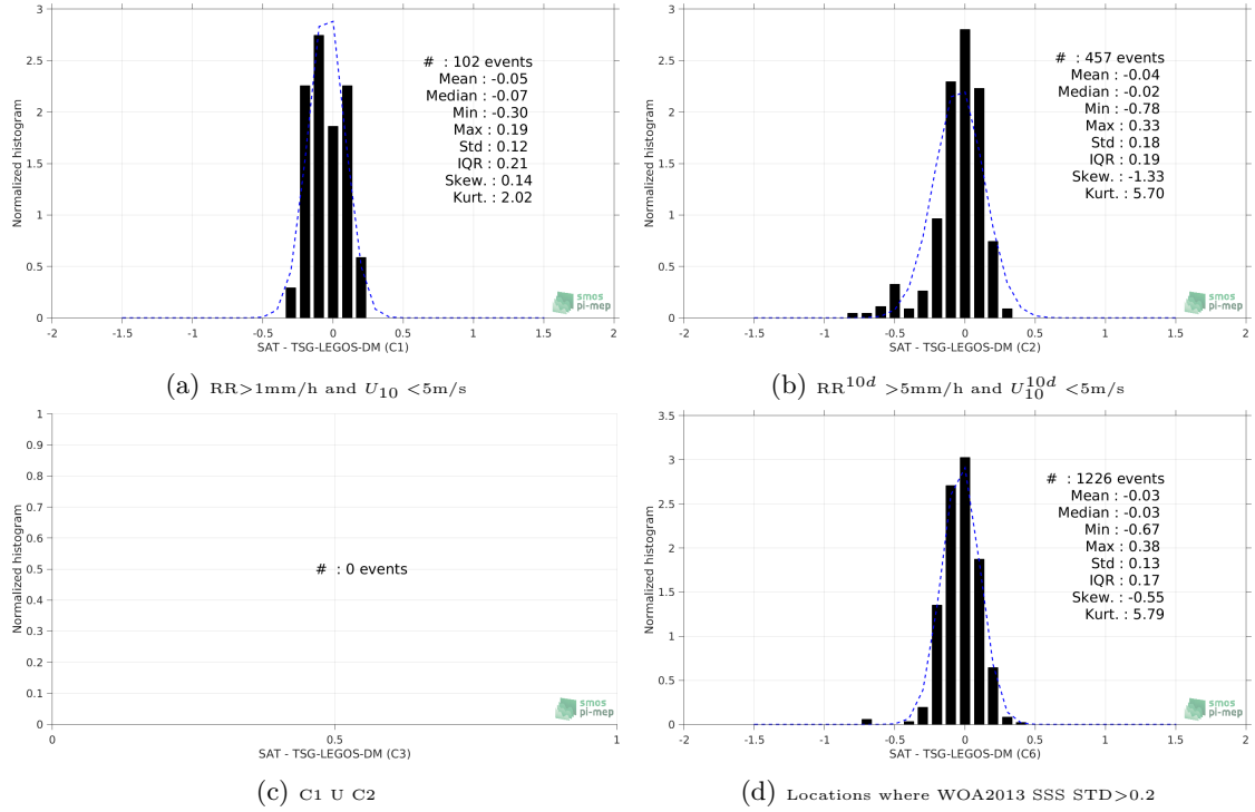
Figure 13: Normalized histogram of \Delta SSS (SMAP-L3-RSS-V3-MONTHLY-70KM - TSG-LEGOS-DM) for 6 different subdatasets corresponding to: RR > 1\text{mm/h} and U_{10} < 5\text{m/s} (a), RR^{10d} > 5\text{mm/h} and U_{10}^{10d} < 5\text{m/s} (b), C1 \cup C2 (c), Locations where WOA2013 SSS STD > 0.2 (d).
