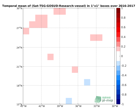
(e) MEAN( \Delta SSS) (Satellite - TSG-GOSUD-Research-vessel)
