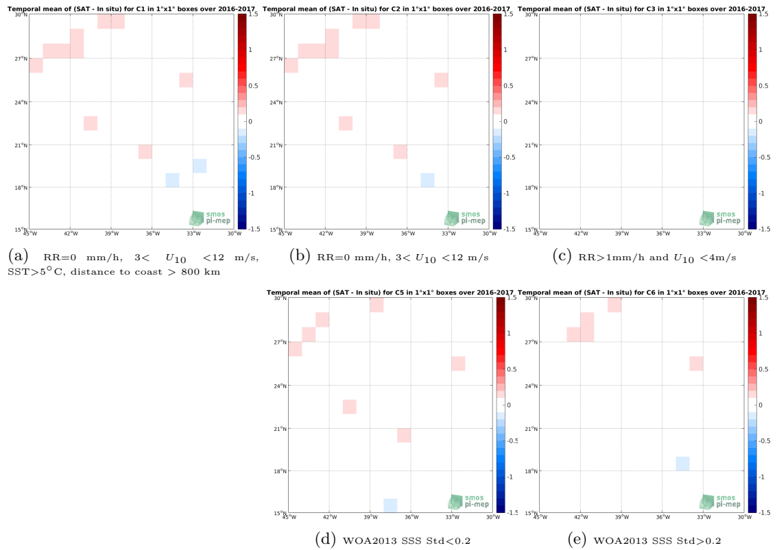
Figure 12: Temporal mean gridded over spatial boxes of size 1^\circ \times 1^\circ of \Delta SSS (SMAP-L3-RSS-V3-MONTHLY-70KM - TSG-GOSUD-Research-vessel) for 5 different subdatasets corresponding to:RR=0 mm/h, 3 < U_{10} < 12 m/s, SST >5^\circ C, distance to coast > 800 km (a), RR=0 mm/h, 3 < U_{10} < 12 m/s (b), RR >1 mm/h and U_{10} < 4 m/s (c), WOA2013 SSS Std <0.2 (d), WOA2013 SSS Std >0.2 (e).
