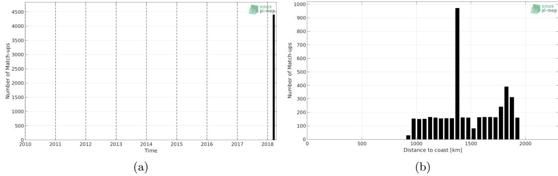
Figure 1: Number of match-ups between TSG-SAMOS and SMAP-L3-RSS-V3-MONTHLY-0.25DEG-40KM SSS as a function of time (a) and as function of the distance to coast (b) over the SPURS 1 Pi-MEP region and for the full satellite product period.
