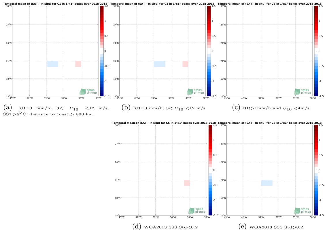
Figure 12: Temporal mean gridded over spatial boxes of size 1^\circ \times 1^\circ of \Delta SSS (SMAP-L3-RSS-V3-MONTHLY-0.25DEG-40KM - TSG-SAMOS) for 5 different subdatasets corresponding to:RR=0 mm/h, 3 < U_{10} < 12 m/s, SST >5^\circ\text{C} , distance to coast > 800 km (a), RR=0 mm/h, 3 < U_{10} < 12 m/s (b), RR >1 mm/h and U_{10} < 4 m/s (c), WOA2013 SSS Std <0.2 (d), WOA2013 SSS Std >0.2 (e).
