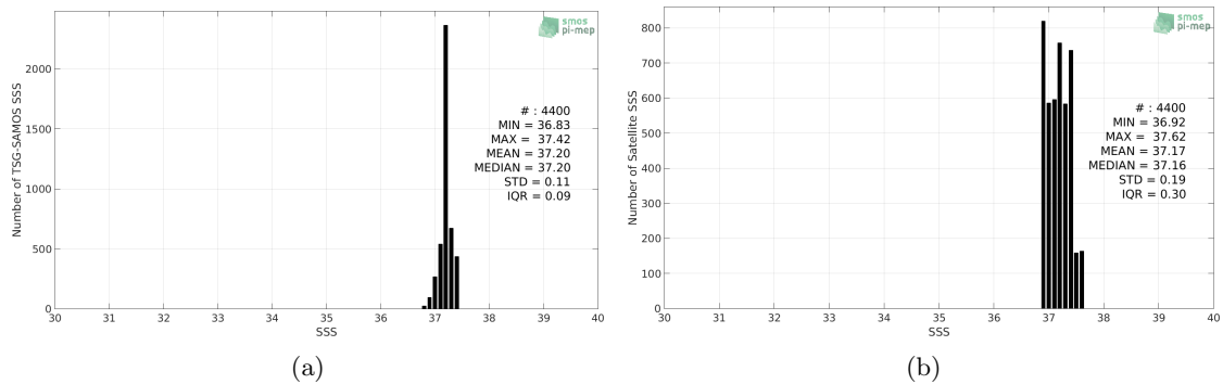
Figure 2: Histograms of SSS from TSG-SAMOS (a) and SMAP-L3-RSS-V3-MONTHLY-0.25DEG-40KM (b) considering all match-up pairs per bins of 0.1 over the SPURS 1 Pi-MEP region and for the full satellite product period.
