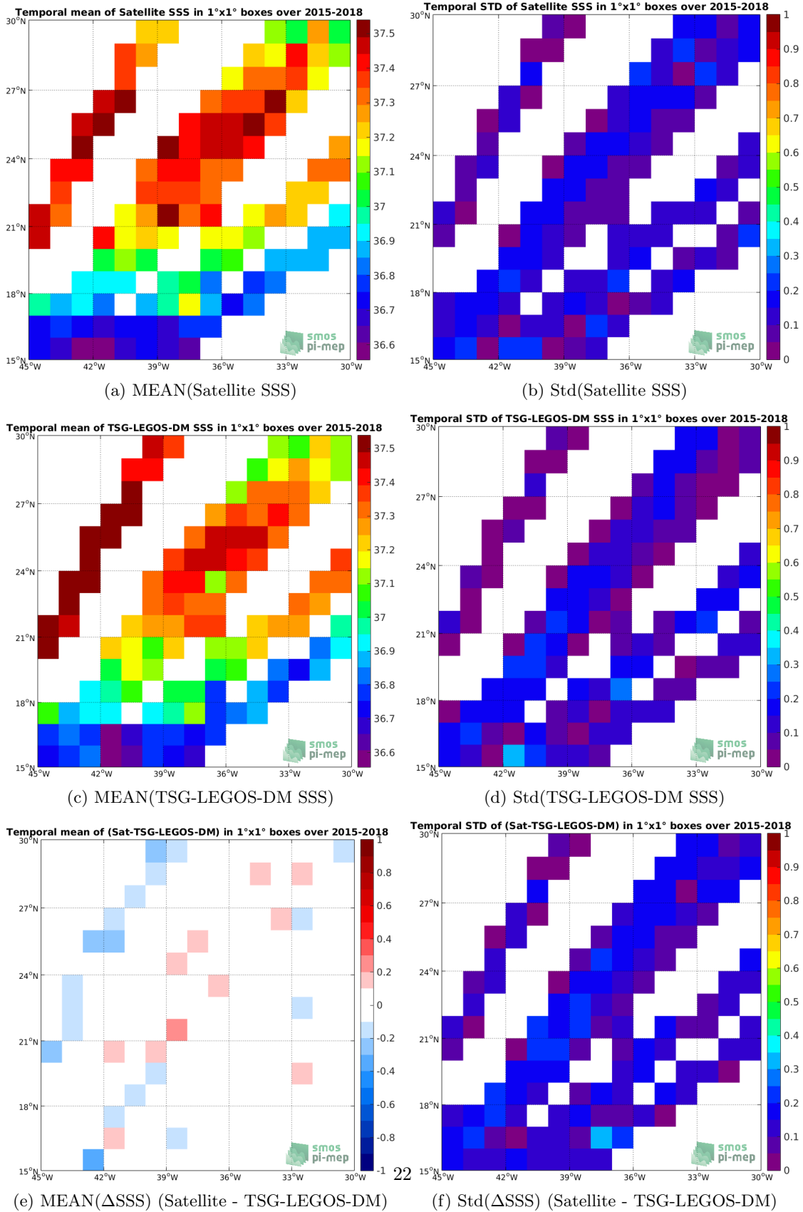
Figure 6: Temporal mean (left) and Std (right) of SSS from SMAP-L3-RSS-V3-MONTHLY-0.25DEG-40KM (top), TSG-LEGOS-DM (middle), and of \Delta SSS (Satellite - TSG-LEGOS-DM). Only match-up pairs are used to generate these maps.
