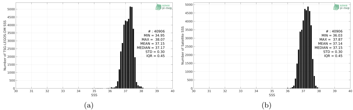
Figure 2: Histograms of SSS from TSG-LEGOS-DM (a) and SMAP-L3-RSS-V3-MONTHLY-0.25DEG-40KM (b) considering all match-up pairs per bins of 0.1 over the SPURS 1 Pi-MEP region and for the full satellite product period.
