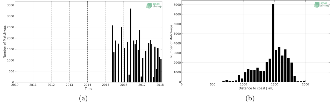
Figure 1: Number of match-ups between TSG-LEGOS-DM and SMAP-L3-RSS-V3-MONTHLY-0.25DEG-40KM SSS as a function of time (a) and as function of the distance to coast (b) over the SPURS 1 Pi-MEP region and for the full satellite product period.
