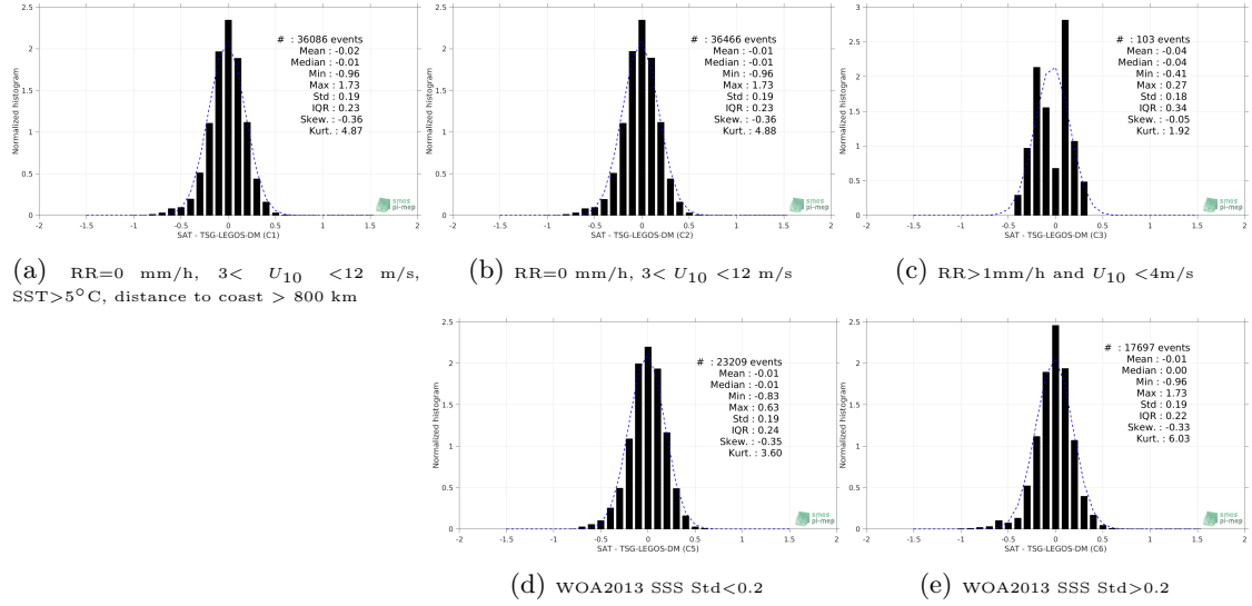
Figure 13: Normalized histogram of \Delta SSS (SMAP-L3-RSS-V3-MONTHLY-0.25DEG-40KM - TSG-LEGOS-DM) for 5 different subdatasets corresponding to: RR=0 mm/h, 3 < U_{10} < 12 m/s, SST>5°C, distance to coast > 800 km (a), RR=0 mm/h, 3 < U_{10} < 12 m/s (b), RR>1mm/h and U_{10} < 4 m/s (c), WOA2013 SSS Std<0.2 (d), WOA2013 SSS Std>0.2 (e).
