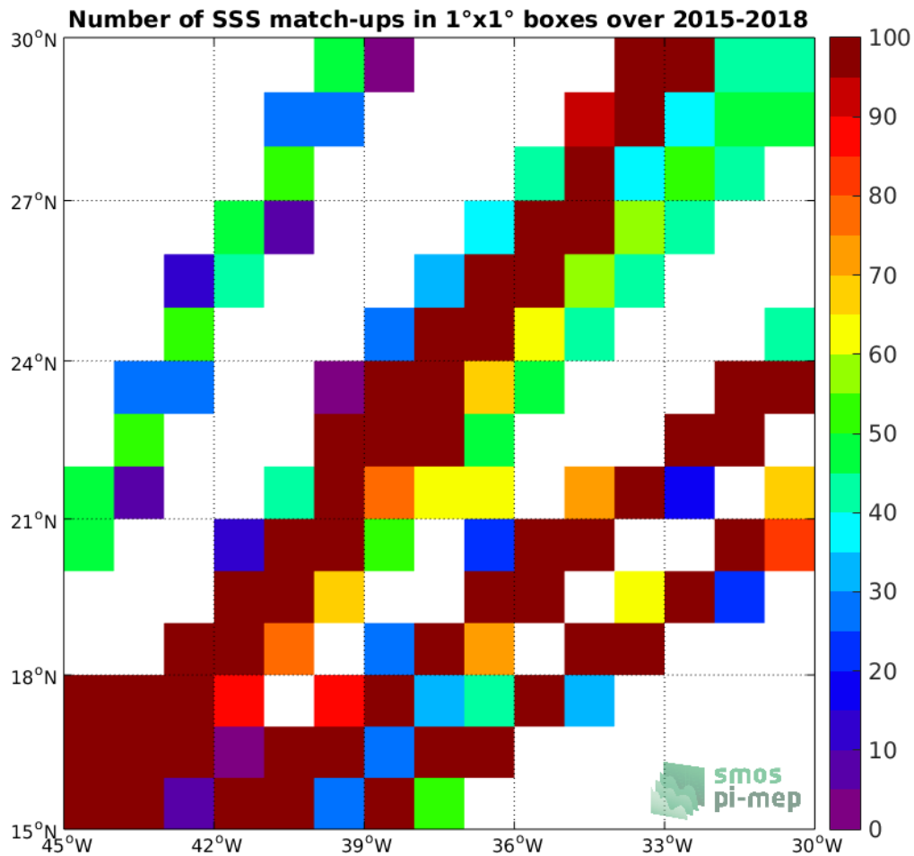
Figure 4: Number of SSS match-ups between TSG-LEGOS-DM SSS and the SMAP-L3-RSS-V3-MONTHLY-0.25DEG-40KM SSS product for the SPURS 1 Pi-MEP region over 1°x1° boxes and for the full satellite product period.
