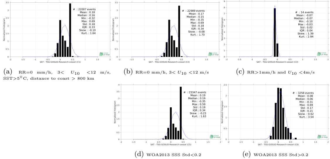
Figure 13: Normalized histogram of \Delta\text{SSS} (SMAP-L3-RSS-V3-MONTHLY-0.25DEG-40KM - TSG-GOSUD-Research-vessel) for 5 different subdatasets corresponding to: RR=0 mm/h, 3 < U_{10} < 12 m/s, SST > 5^\circ\text{C} , distance to coast > 800 km (a), RR=0 mm/h, 3 < U_{10} < 12 m/s (b), RR > 1\text{mm/h} and U_{10} < 4\text{m/s} (c), WOA2013 SSS Std < 0.2 (d), WOA2013 SSS Std > 0.2 (e).
