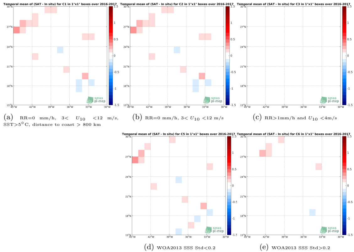
Figure 12: Temporal mean gridded over spatial boxes of size 1^\circ \times 1^\circ of \Delta SSS (SMAP-L3-RSS-V3-MONTHLY-0.25DEG-40KM - TSG-GOSUD-Research-vessel) for 5 different subdatasets corresponding to:RR=0 mm/h, 3 < U_{10} < 12 m/s, SST >5^\circ C, distance to coast > 800 km (a), RR=0 mm/h, 3 < U_{10} < 12 m/s (b), RR >1 mm/h and U_{10} < 4 m/s (c), WOA2013 SSS Std <0.2 (d), WOA2013 SSS Std >0.2 (e).
