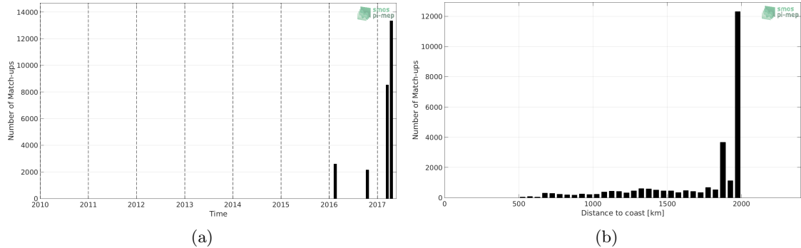
Figure 1: Number of match-ups between TSG-GOSUD-Research-vessel and SMAP-L3-RSS-V3-MONTHLY-0.25DEG-40KM SSS as a function of time (a) and as function of the distance to coast (b) over the SPURS 1 Pi-MEP region and for the full satellite product period.
