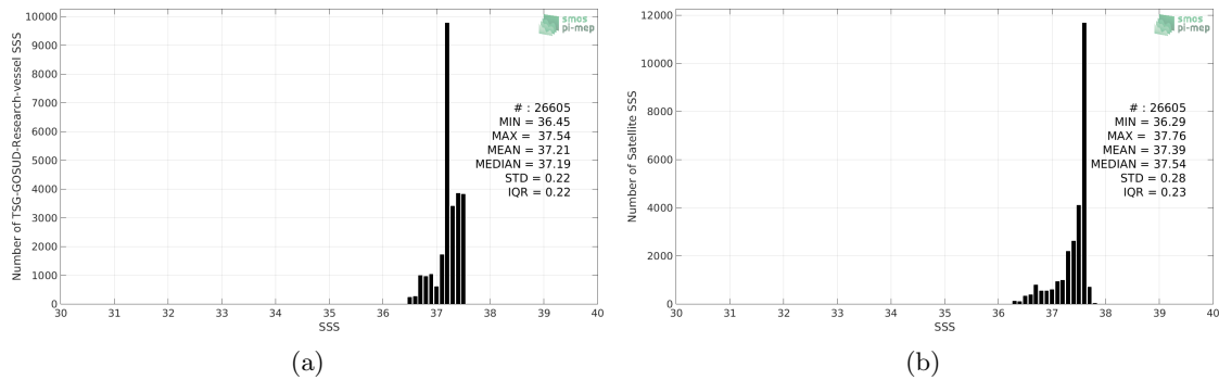
Figure 2: Histograms of SSS from TSG-GOSUD-Research-vessel (a) and SMAP-L3-RSS-V3-MONTHLY-0.25DEG-40KM (b) considering all match-up pairs per bins of 0.1 over the SPURS 1 Pi-MEP region and for the full satellite product period.
