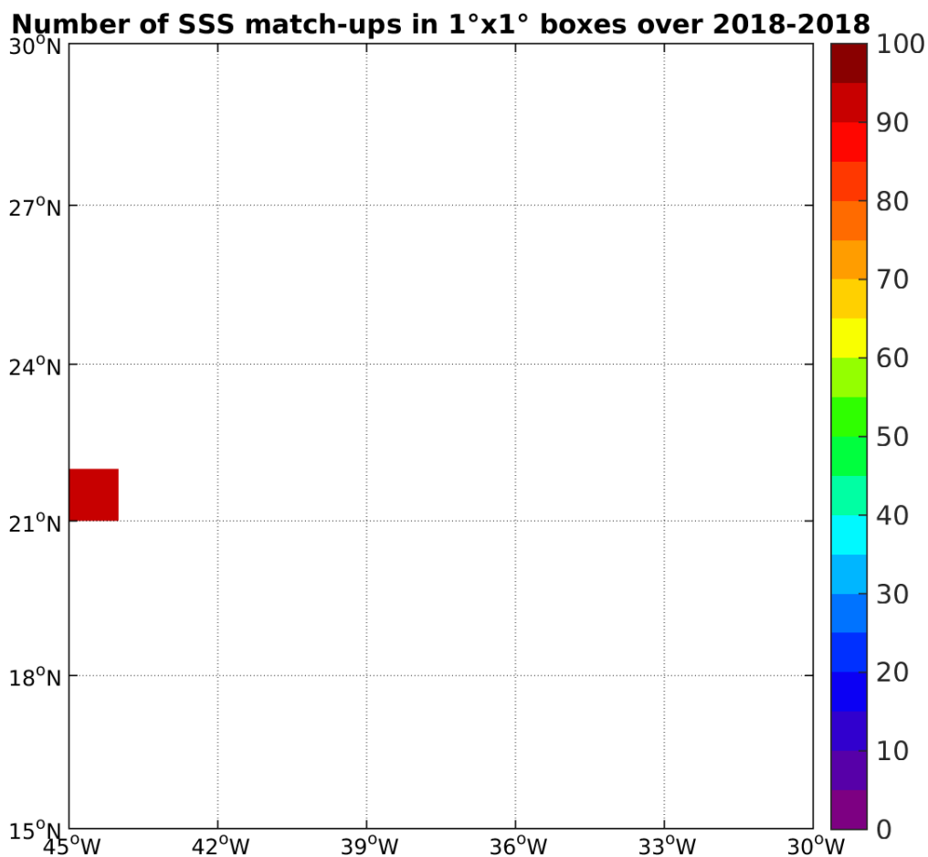
Figure 4: Number of SSS match-ups between TSG-SAMOS SSS and the SMAP-L3-RSS-V2-8DAY-RUNNING-40KM SSS product for the SPURS 1 Pi-MEP region over 1°x1° boxes and for the full satellite product period.
