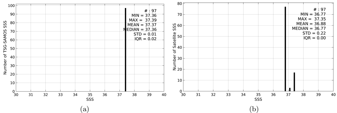
Figure 2: Histograms of SSS from TSG-SAMOS (a) and SMAP-L3-RSS-V2-8DAY-RUNNING-40KM (b) considering all match-up pairs per bins of 0.1 over the SPURS 1 Pi-MEP region and for the full satellite product period.
