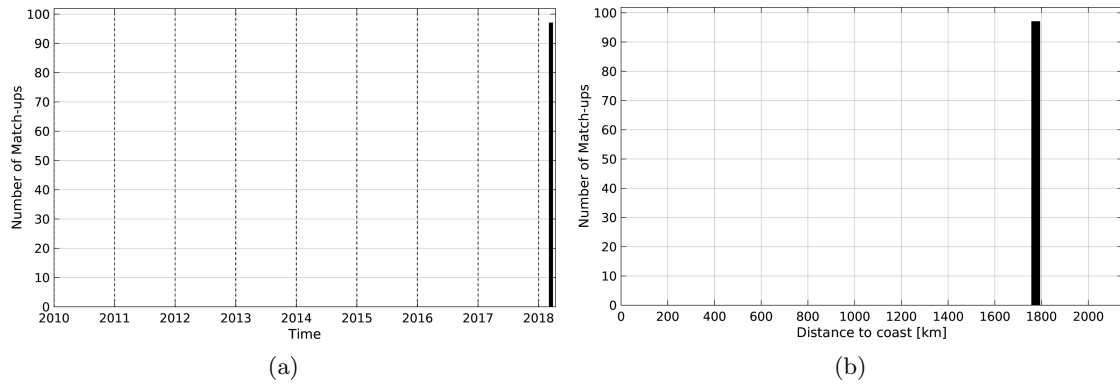
Figure 1: Number of match-ups between TSG-SAMOS and SMAP-L3-RSS-V2-8DAY-RUNNING-40KM SSS as a function of time (a) and as function of the distance to coast (b) over the SPURS 1 Pi-MEP region and for the full satellite product period.
