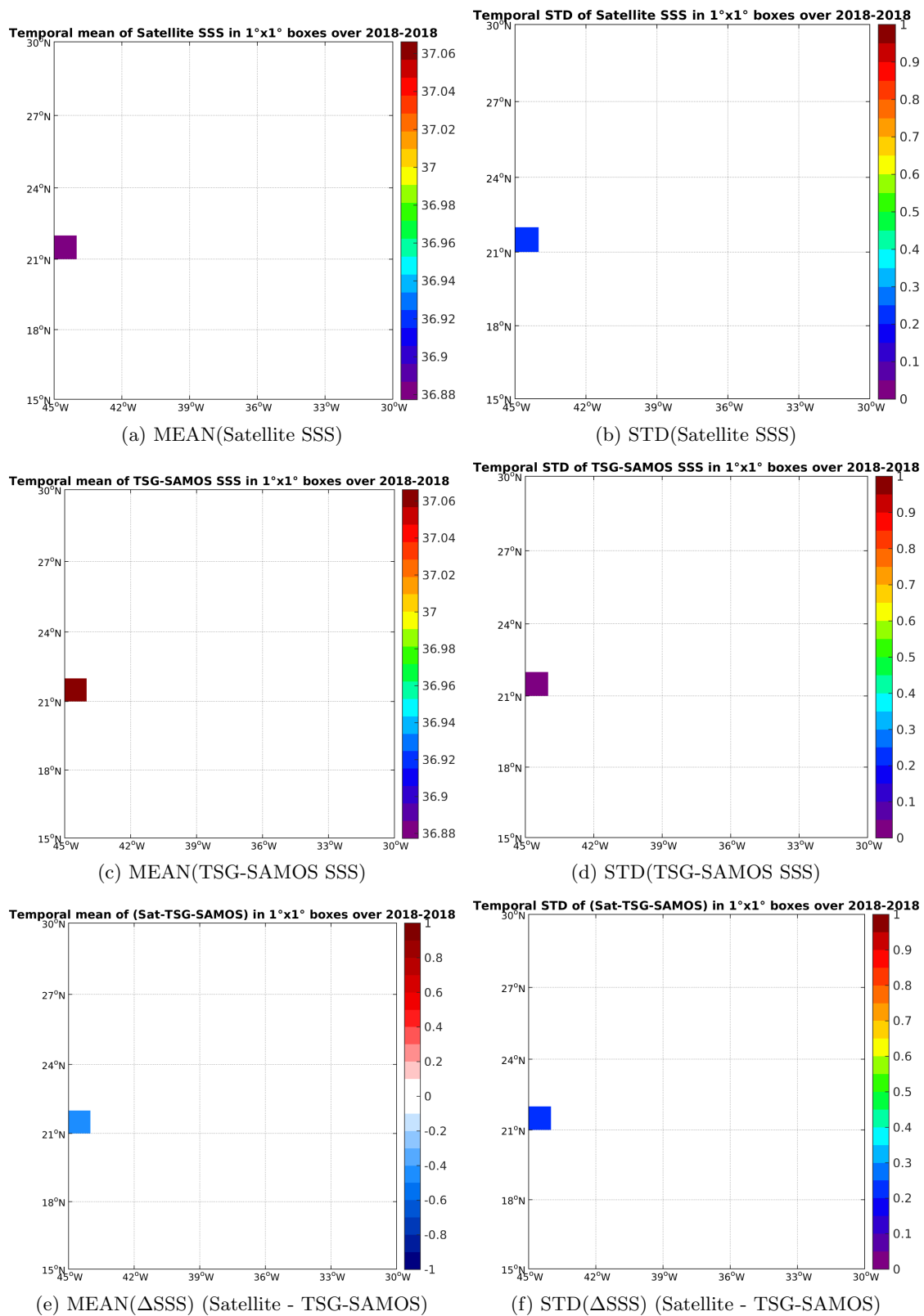
Figure 6: Temporal mean (left) and STD (right) of SSS from SMAP-L3-RSS-V2-8DAY-RUNNING-40KM (top), TSG-SAMOS (middle), and of \Delta SSS (Satellite - TSG-SAMOS). Only match-up pairs are used to generate these maps.
