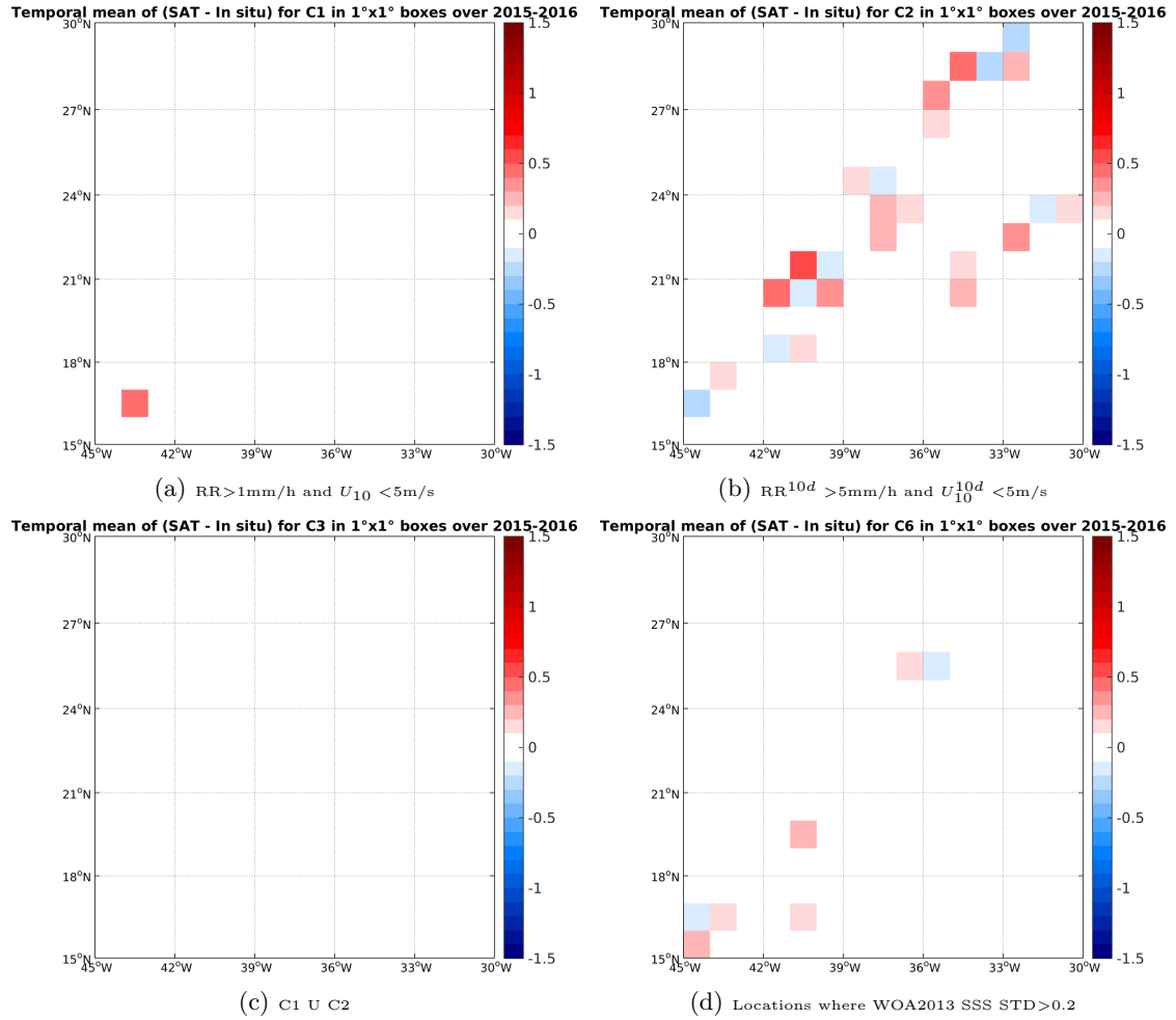
Figure 12: Temporal mean gridded over spatial boxes of size 1^\circ \times 1^\circ of \Delta SSS (SMAP-L3-RSS-V2-8DAY-RUNNING-40KM - TSG-LEGOS-DM) for 4 different subdatasets corresponding to: RR > 1mm/h and U_{10} < 5m/s (a), RR 10d > 5mm/h and U_{10}^{10d} < 5m/s (b), C1 U C2 (c), Locations where WOA2013 SSS STD > 0.2 (d).
