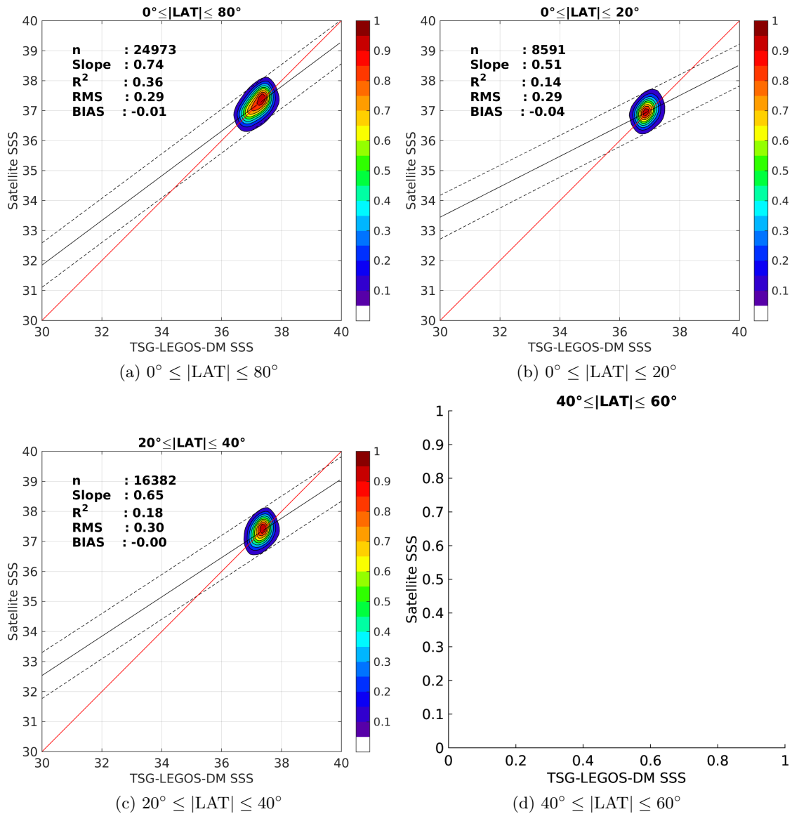
Figure 9: Contour maps of the concentration of SMAP-L3-RSS-V2-8DAY-RUNNING-40KM SSS (y-axis) versus TSG-LEGOS-DM SSS (x-axis) at match-up pairs for different latitude bands. For each plot, the red line shows x=y . The black thin and dashed lines indicate a linear fit through the data cloud and the \pm 95\% confidence levels, respectively. The number match-up pairs n , the slope and R^2 coefficient of the linear fit, the root mean square (RMS) and the mean bias between satellite and in situ data are indicated for each latitude band in each plots.
