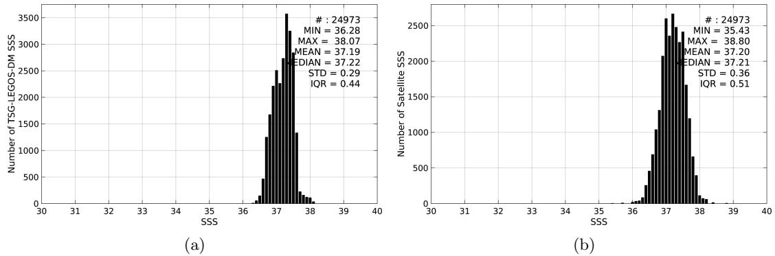
Figure 2: Histograms of SSS from TSG-LEGOS-DM (a) and SMAP-L3-RSS-V2-8DAY-RUNNING-40KM (b) considering all match-up pairs per bins of 0.1 over the SPURS 1 Pi-MEP region and for the full satellite product period.
