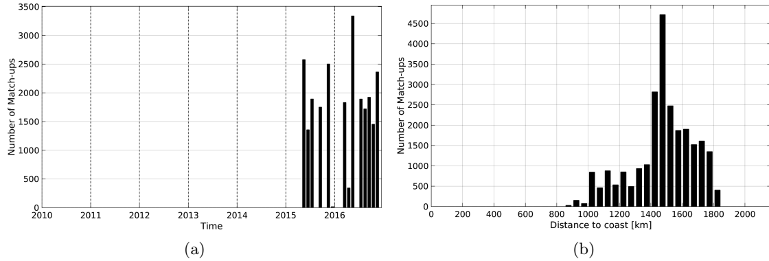
Figure 1: Number of match-ups between TSG-LEGOS-DM and SMAP-L3-RSS-V2-8DAY-RUNNING-40KM SSS as a function of time (a) and as function of the distance to coast (b) over the SPURS 1 Pi-MEP region and for the full satellite product period.
