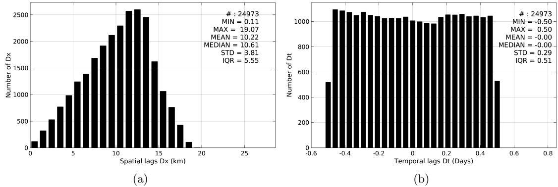
Figure 5: Histograms of the spatial (a) and temporal (b) lags between the time of the TSG-LEGOS-DM measurements and the date of the corresponding SMAP-L3-RSS-V2-8DAY-RUNNING-40KM SSS product.
