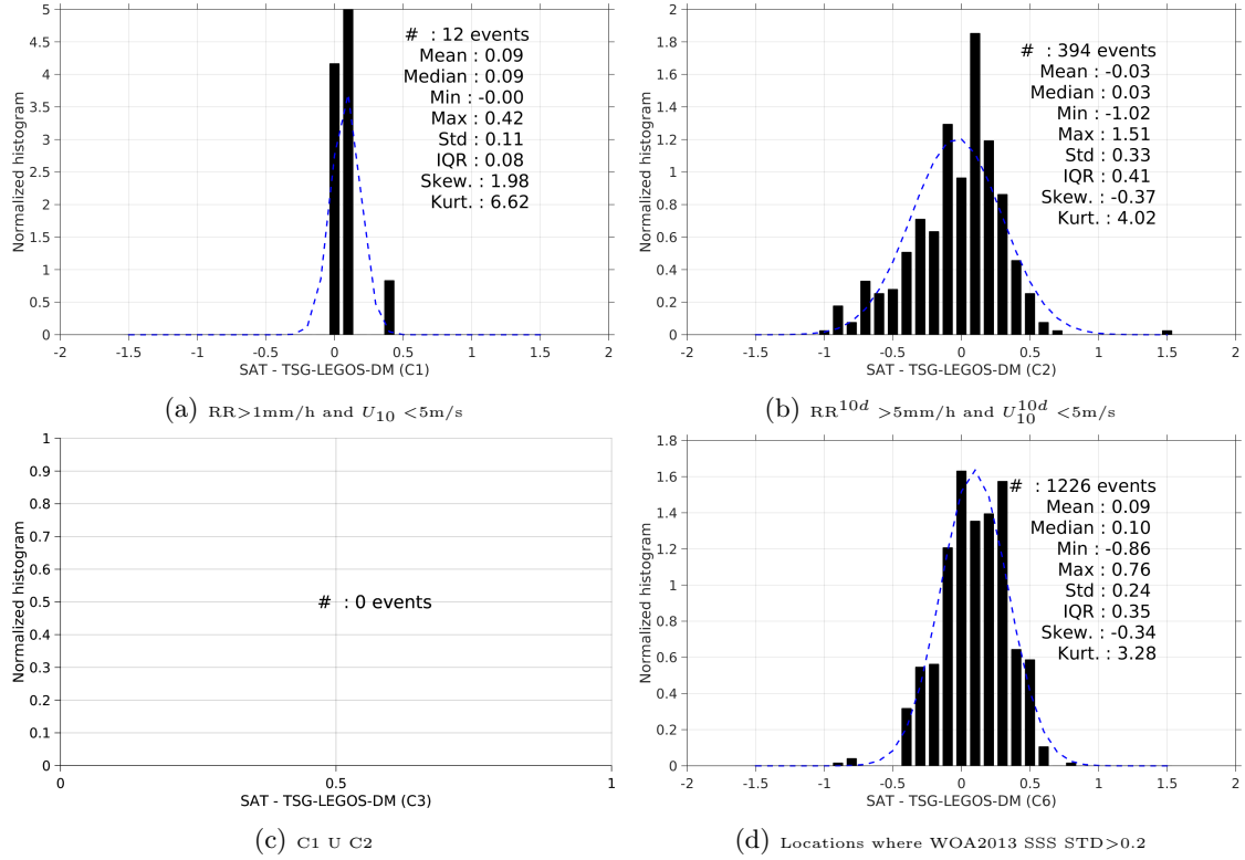
Figure 13: Normalized histogram of \Delta\text{SSS} (SMAP-L3-RSS-V2-8DAY-RUNNING-40KM - TSG-LEGOS-DM) for 6 different subdatasets corresponding to: RR > 1mm/h and U_{10} < 5\text{m/s} (a), RR^{10d} > 5\text{mm/h} and U_{10}^{10d} < 5\text{m/s} (b), C1 U C2 (c), Locations where WOA2013 SSS STD > 0.2 (d).
