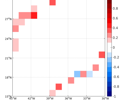
(e) MEAN( \Delta SSS) (Satellite - TSG-GOSUD-Research-vessel)
