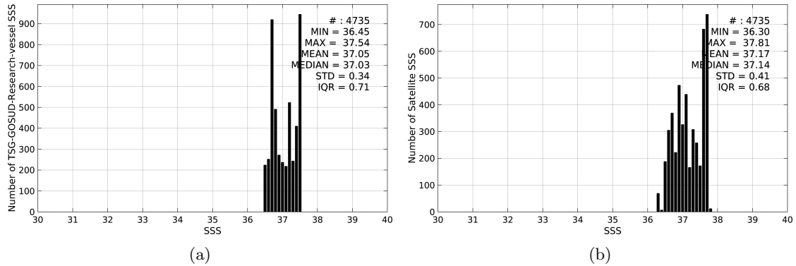
Figure 2: Histograms of SSS from TSG-GOSUD-Research-vessel (a) and SMAP-L3-RSS-V2-8DAY-RUNNING-40KM (b) considering all match-up pairs per bins of 0.1 over the SPURS 1 Pi-MEP region and for the full satellite product period.
