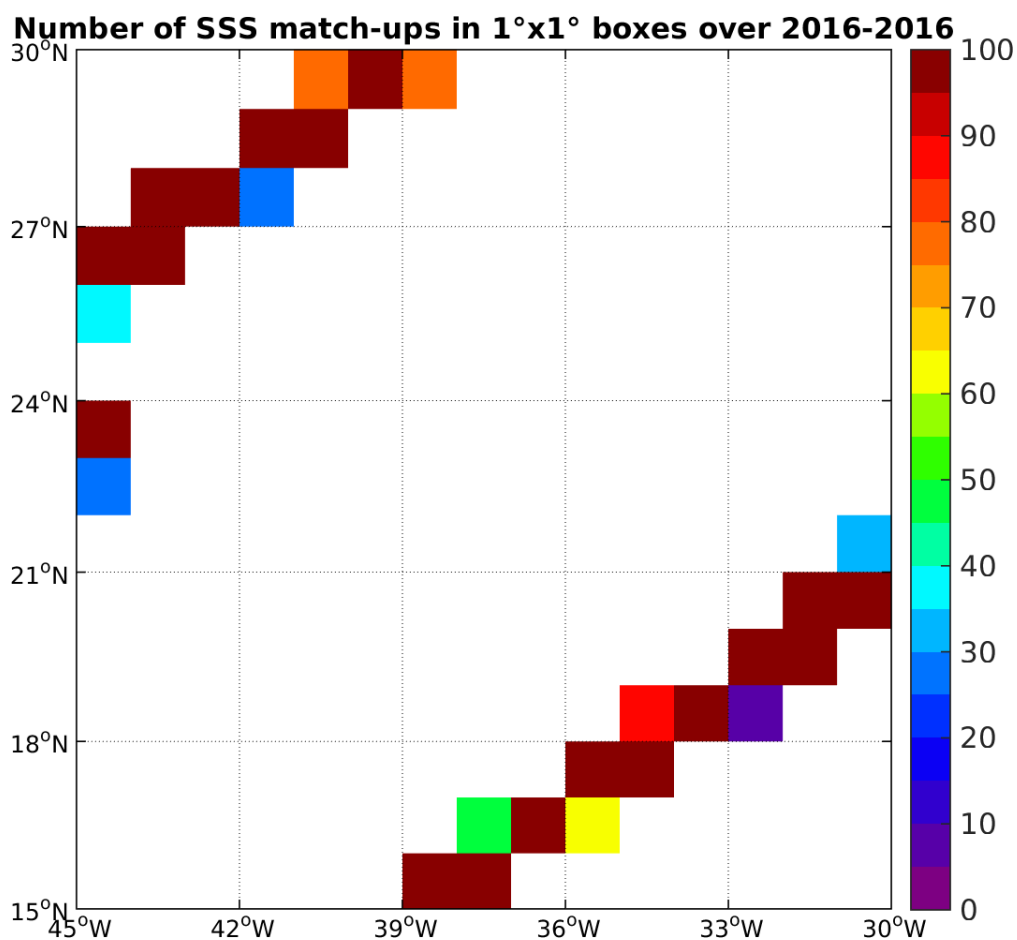
Figure 4: Number of SSS match-ups between TSG-GOSUD-Research-vessel SSS and the SMAP-L3-RSS-V2-8DAY-RUNNING-40KM SSS product for the SPURS 1 Pi-MEP region over 1°x1° boxes and for the full satellite product period.
