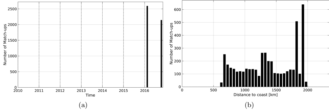
Figure 1: Number of match-ups between TSG-GOSUD-Research-vessel and SMAP-L3-RSS-V2-8DAY-RUNNING-40KM SSS as a function of time (a) and as function of the distance to coast (b) over the SPURS 1 Pi-MEP region and for the full satellite product period.
