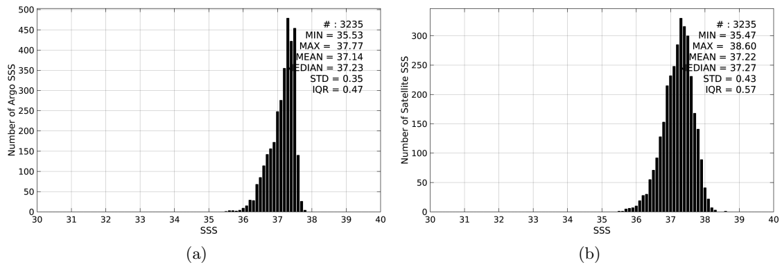
Figure 2: Histograms of SSS from Argo (a) and SMAP-L3-RSS-V2-8DAY-RUNNING-40KM (b) considering all match-up pairs per bins of 0.1 over the SPURS 1 Pi-MEP region and for the full satellite product period.
