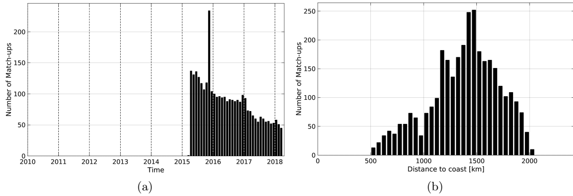
Figure 1: Number of match-ups between Argo and SMAP-L3-RSS-V2-8DAY-RUNNING-40KM SSS as a function of time (a) and as function of the distance to coast (b) over the SPURS 1 Pi-MEP region and for the full satellite product period.
