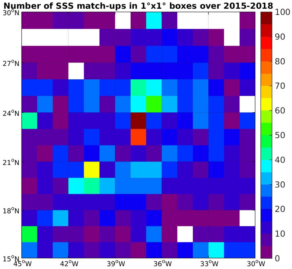
Figure 4: Number of SSS match-ups between Argo SSS and the SMAP-L3-RSS-V2-8DAY-RUNNING-40KM SSS product for the SPURS 1 Pi-MEP region over 1°x1° boxes and for the full satellite product period.
