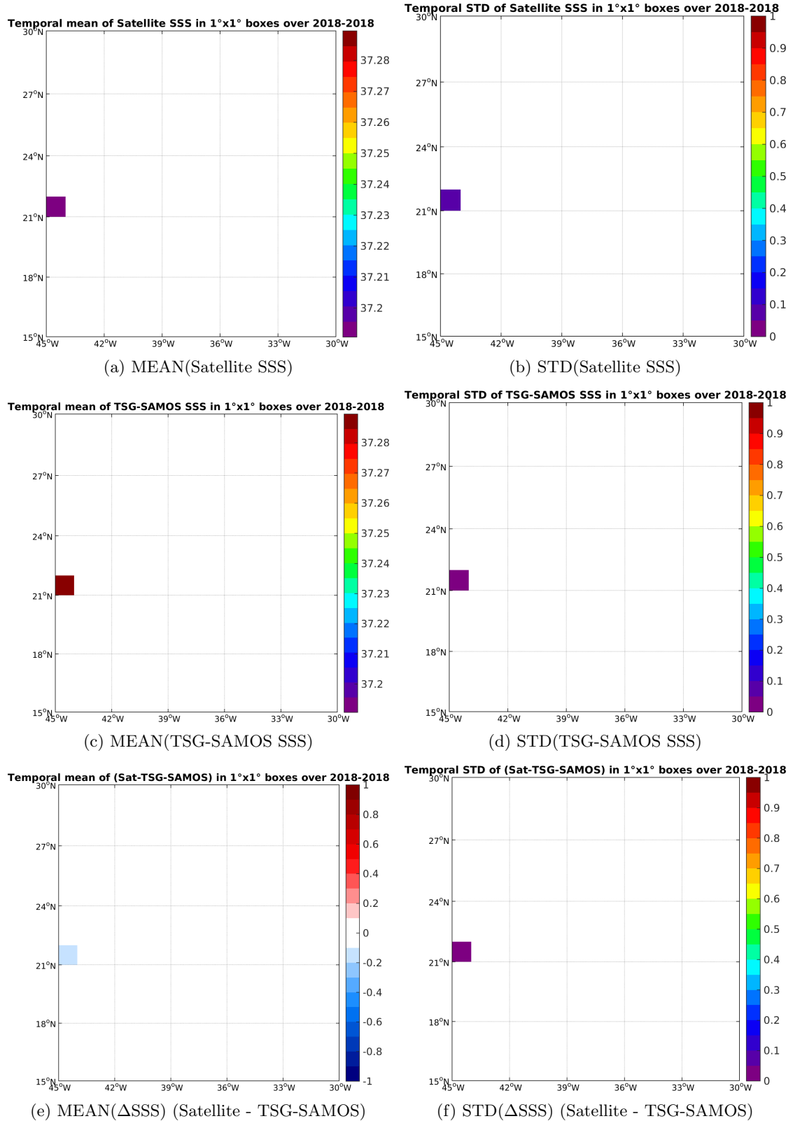
Figure 6: Temporal mean (left) and STD (right) of SSS from SMAP-L3-RSS-V2-8DAY-RUNNING-70KM (top), TSG-SAMOS (middle), and of \Delta SSS (Satellite - TSG-SAMOS). Only match-up pairs are used to generate these maps.
