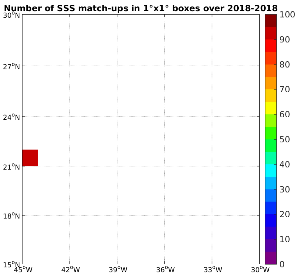
Figure 4: Number of SSS match-ups between TSG-SAMOS SSS and the SMAP-L3-RSS-V2-8DAY-RUNNING-70KM SSS product for the SPURS 1 Pi-MEP region over 1°x1° boxes and for the full satellite product period.
