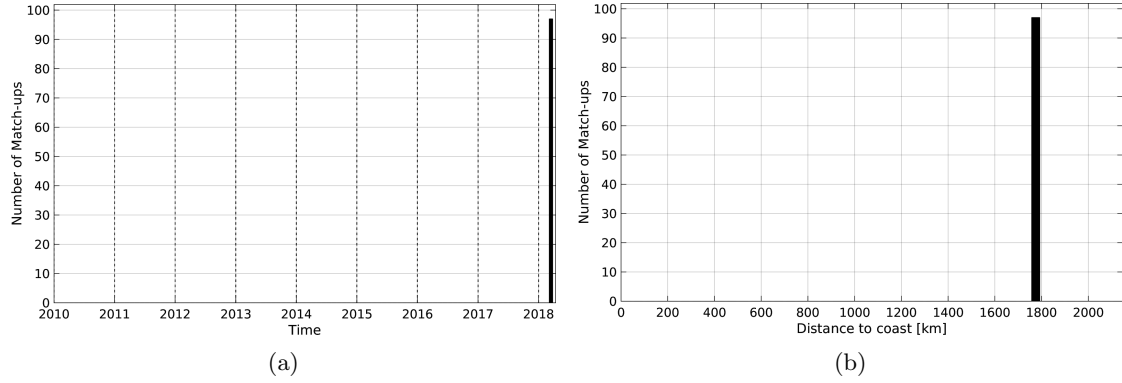
Figure 1: Number of match-ups between TSG-SAMOS and SMAP-L3-RSS-V2-8DAY-RUNNING-70KM SSS as a function of time (a) and as function of the distance to coast (b) over the SPURS 1 Pi-MEP region and for the full satellite product period.
