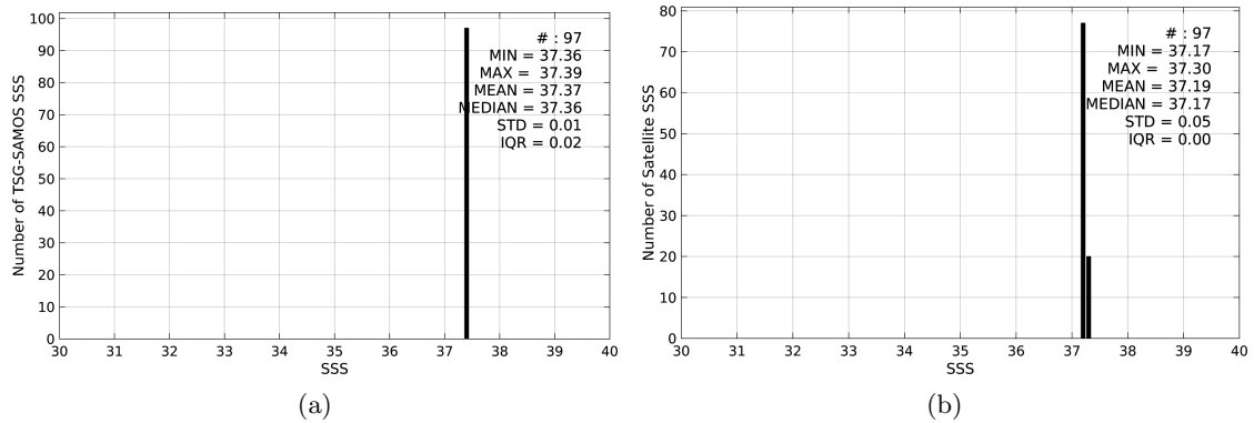
Figure 2: Histograms of SSS from TSG-SAMOS (a) and SMAP-L3-RSS-V2-8DAY-RUNNING-70KM (b) considering all match-up pairs per bins of 0.1 over the SPURS 1 Pi-MEP region and for the full satellite product period.
